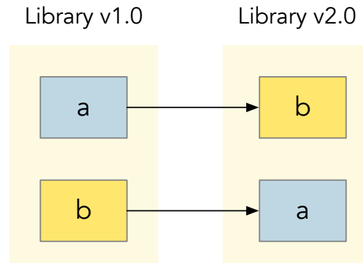
Figure 8.2: Circular renaming is a particularly challenging case when the names of two software artifacts are being swapped: a is renamed to b and at the same time b is renamed to a .
