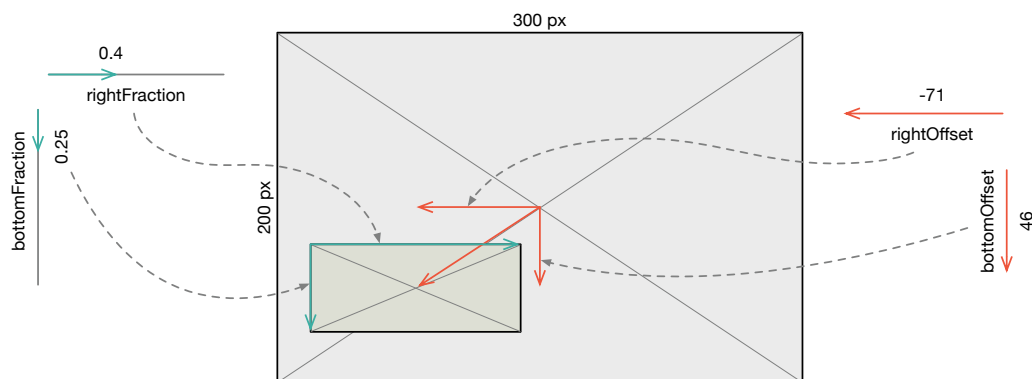
Figure 8.5: To position a submorph inside a parent morph, client provides four parameters: bottomFraction, rightFraction, bottomOffset, and rightOffset. All four are numbers. They can represent percentages (in the case of fractions), or be negative (in the case of offsets).
