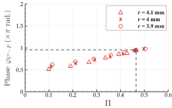
Figure 4.20: Phase \varphi_{U'-r} of the velocity-based flame describing function plotted against \Pi . The acoustic pressure is measured at the central flame location simultaneously with the axial velocity measurement at r = 3.9 mm, r = 4 mm and r = 4.1 mm. The meaning of the grey-filled symbols is indicated in the text. The acoustic forcing frequency f_r is 748 Hz.
