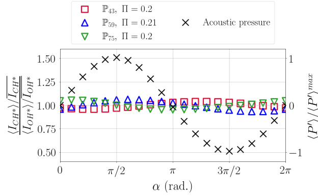
Figure 6.8: Relative equivalence ratio fluctuations estimated with the ratio between the reduced phase-averaged \text{CH}^* and \text{OH}^* intensities measured with PM.
