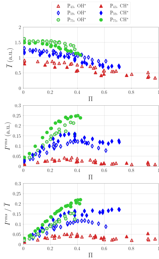
Figure 6.6: Response of the flame as a function of \Pi = P^{rms} / \rho^a U_b^2 for the three flame powers, and for CH^* and OH^* radicals. Top: Mean radical light intensity \bar{I}(\Pi, \mathbb{P}) ; middle: rms radical emission intensity I^{rms}(\Pi, \mathbb{P}) ; bottom: I^{rms} / \bar{I}(\Pi, \mathbb{P}) .
