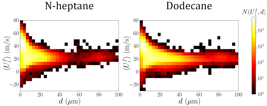
Figure 8.16: Fuel drop size-velocity correlations at z = 2.1 mm, \Pi = 0.22 . N(U_z^f, d) indicates the number of droplets in each class of diameter-width 3 \mu\text{m} and velocity-width 5 m/s. Left: n-heptane; right: dodecane.
