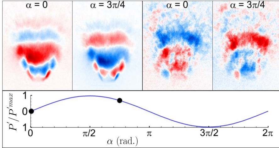
Figure 7.7: DMD images of 2000 instantaneous flame front \text{OH}^* emission images for \Pi = 0.45 (left) and 1.27 (right), post-synchronised with the acoustic pressure. \mathbb{P}_{43} , \phi = 0.85 . Points: values of the phase angle \alpha associated to the images.
