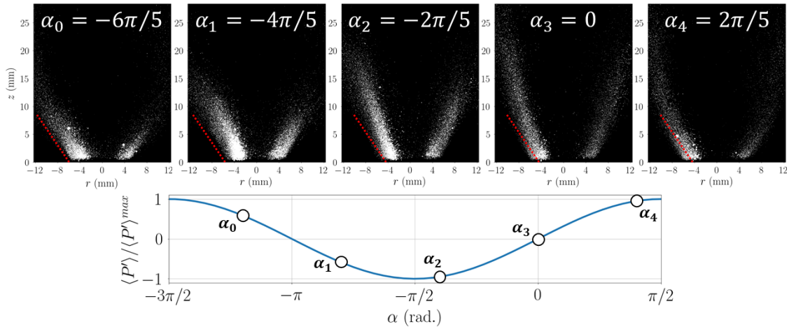
Figure 5.23: Phase-averaged spray images. \Pi \simeq 0.38 , f_r = 716 Hz. At the bottom, the phase-averaged acoustic pressure cycle is represented with five dots indicating the phase angle at which the images are obtained. The red line, identical on all the images, helps to appreciate the modification of the spray angle.
