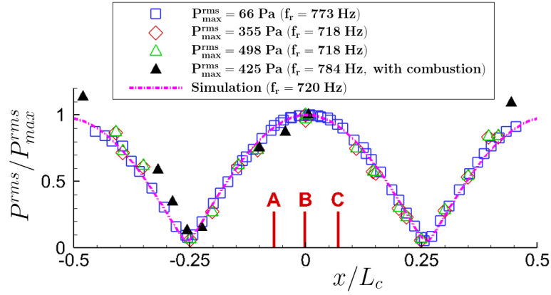
Figure 7.3: Pressure amplitude along the x-axis ( y = 0, z = 0.12h_c ). W/o combustion: L_c = 522 mm, f_r = 773 Hz (w/o the convergent part (c.p.)), f_r = 718 Hz (with c.p.). With combustion: L_c = 800 mm, f_r = 784 Hz (with c.p.). Red lines and letters A, B and C: position of flames.
