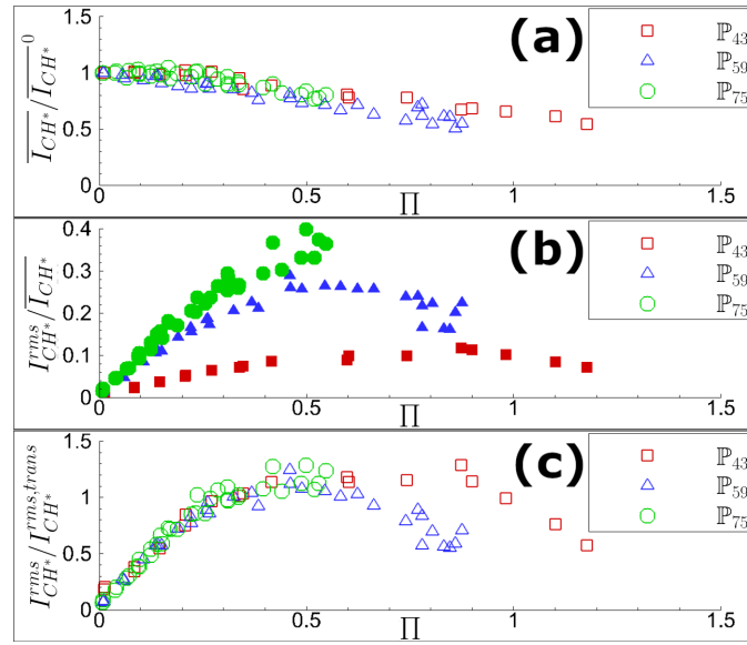
Figure 7.5: Response of the flame vs. \Pi = P^{rms} / \rho^a U_b^2 for three flame powers \mathbb{P} : (a) normalised mean intensity \overline{I_{CH^*}} / \overline{I_{CH^*}}^0 ; (b) reduced rms intensity I_{CH^*}^{rms} / \overline{I_{CH^*}} filtered at f_r ; (c) reduced rms intensity I_{CH^*}^{rms} / I_{CH^*}^{rms,trans} filtered at f_r .
