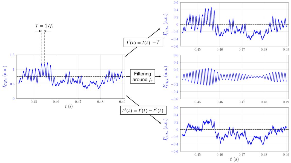
(a) Raw and filtered time-averaged CH * -intensity signals
