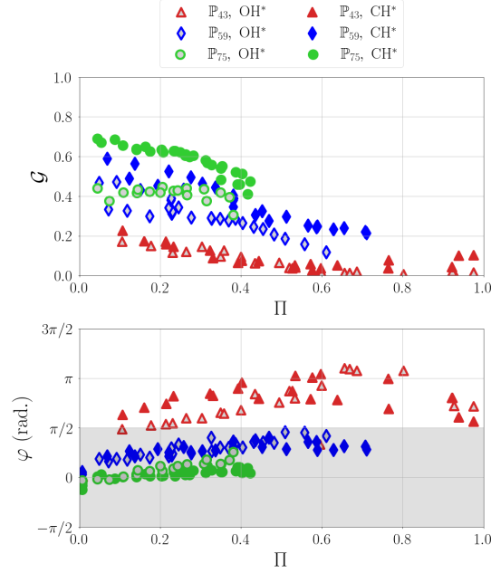
Figure 6.7: Flame describing function \mathcal{F} vs. \Pi = P^{rms}/\rho^a U_b^2 for the three flame powers for CH* and OH* radicals. Top: gain, bottom: phase. The grey zone indicates the region of potential instability.
