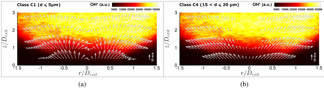
Figure 7.2: N-heptane droplets velocity field sorted by droplet size classes and mean OH* intensity field ( \phi = 0.95 ).
