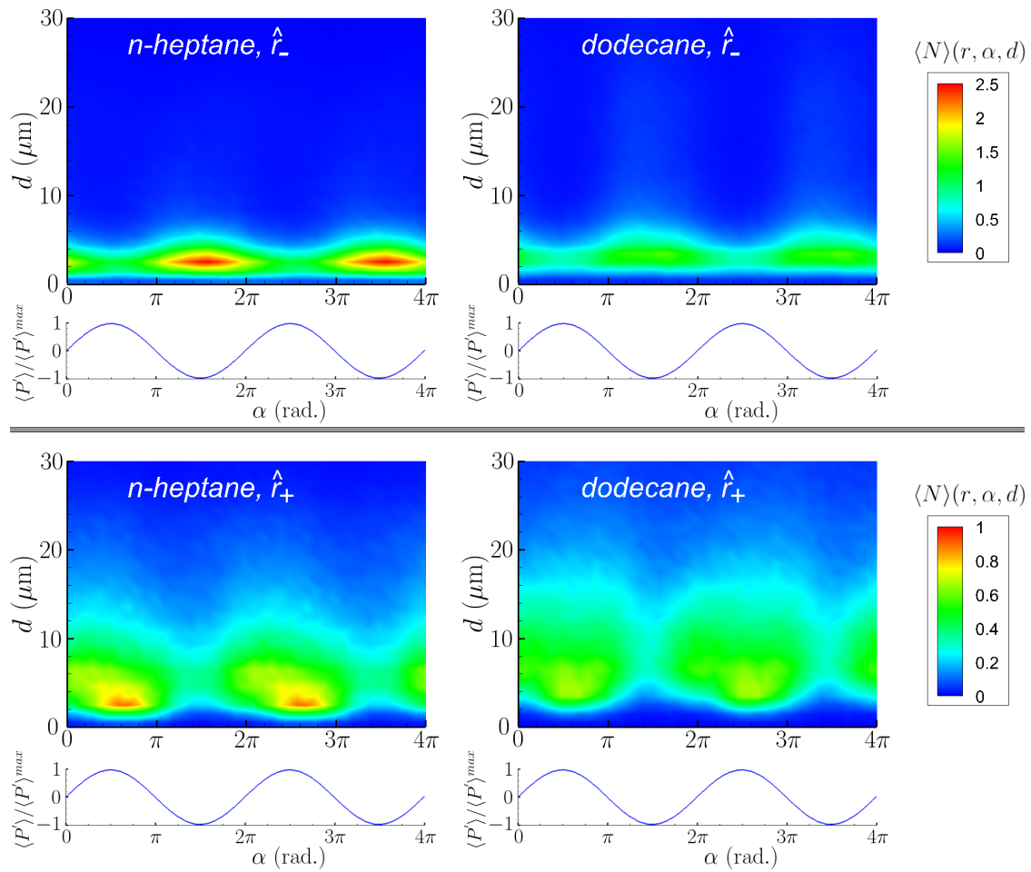
Figure 8.17: Phase-averaged drop size distribution \langle N \rangle(r, \alpha, d) at z = 2.1 \text{ mm} for \Pi = 0.22 . Left: n-heptane fuel; right: dodecane fuel; top: inner region of the spray, \hat{r}_- ( r \leq 4 \text{ mm} ); middle: outer region of the spray, \hat{r}_+ ( r > 4 \text{ mm} ); bottom: two reconstructed acoustic cycles.
