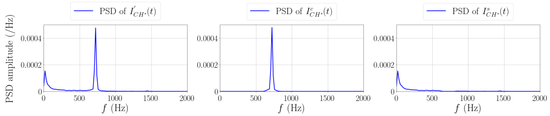
(b) PSDs of the raw and filtered CH * -intensity signals
