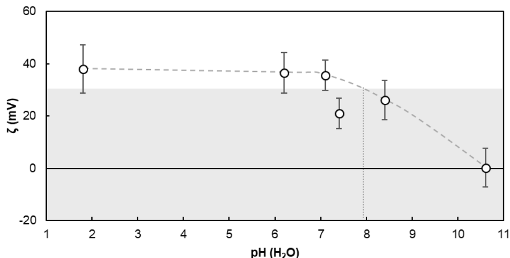
Figure 1.15. Evolution of 1 g/L TiO 2 P25 nanoparticle zeta potential with pH in methanol referred to the aqueous pH scale at 25.0 °C. pH is adjusted with HCl and NaOH. Ionic strength is kept constant at 10 -3 M with NaCl. Instability area is marked in grey.
