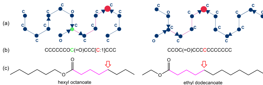
Figure 5. Encoding hexyl octanoate and ethyl dodecanoate into directed graphs: (a) directed graphs with root nodes in red; the root node position computed automatically for hexyl octanoate is colored in green and the path between the functional atom node and the root node in pink, (b) SMILES codes with the expected position of the root nodes indicated in red and (c) 2D formulas with expected positions for the root nodes (red arrows). The atom types C and O added on the directed graphs correspond to node labels that are inputs of the parameterized function implemented at each node of the graph to build the GM.
