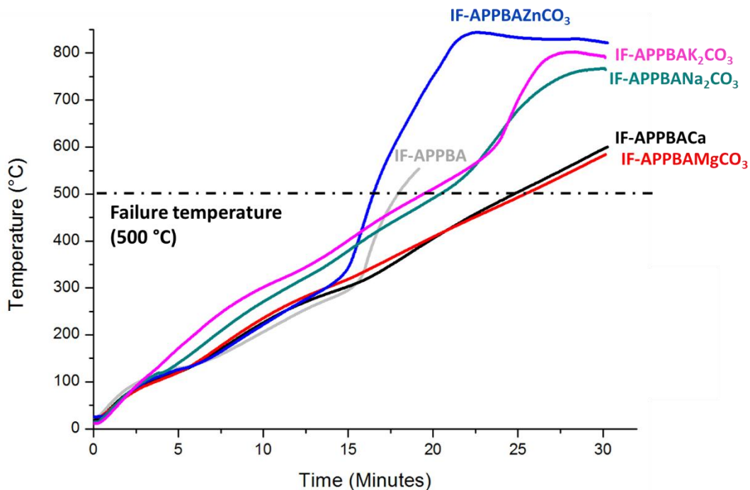
Figure 74 Time-temperature curves of IF-APPBACa, IF-APPBAMgCO 3 , IF-APPBAZnCO 3 , IF-APPBAK 2 CO 3 and IF-APPBANa 2 CO 3
