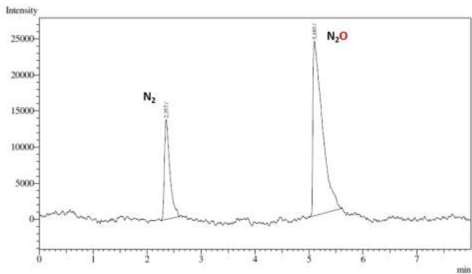
Figure S27: Control experiment without TEOA
