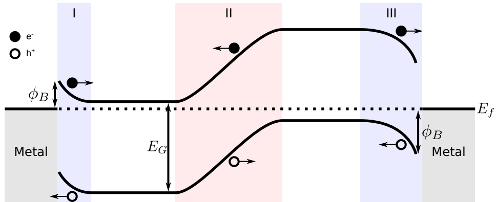
FIGURE 5.B.1: Band diagram of a p - n junction (II) with Schottky contacts (I & III). Arrows indicate the directions in which the carriers are accelerated. According to the current convention, the resulting current is positive for the Schottky contacts and negative for the p - n junction.
