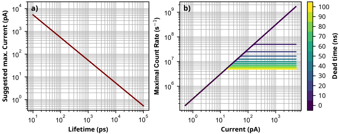
FIGURE 2.12: (a) Suggested maximal e-beam current for lifetimes ranging from 10 ps to 100 ns, based on equation (2.11) . (b) Maximal useful count rate per channel taking into account dead time and pile-up for different dead time, based on equations (2.17) and (2.26) .
