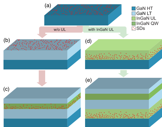
FIGURE 3.1: (a) Surface defects (SDs) are formed during the growth of high-temperature GaN. (b) These defects strongly segregate even during low-temperature growth of GaN. (c) SDs react with In atoms and are eventually trapped in the InGaN QW, creating non-radiative recombination centers. (d) InGaN underlayer in which SDs are trapped due to their interaction with In atoms. (e) After the InGaN underlayer, the GaN surface is free of defects leading to high-efficiency InGaN/GaN QW. Adapted from [Hal+19]
