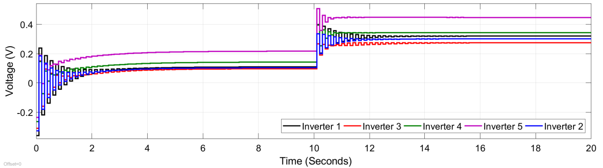
Figure 3.4 – MPC signals for all the inverters when there is a load change at t = 0s and t = 10s using the non-cooperative scheme.
