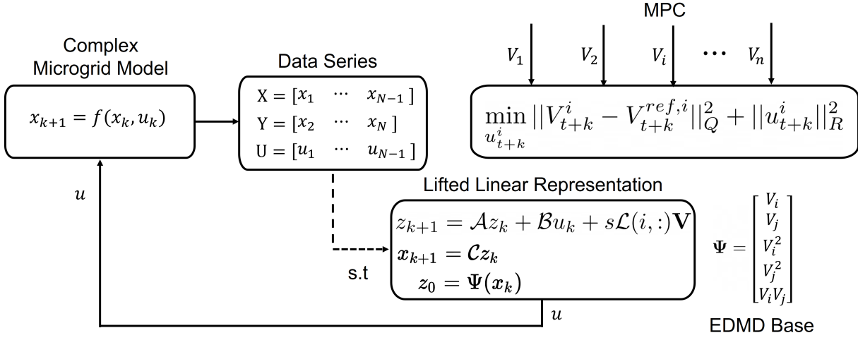
Figure 3.1 – The Koopman-based linear predictor of each agent is used to set a Non-Cooperative MPC by including a consensus term.
