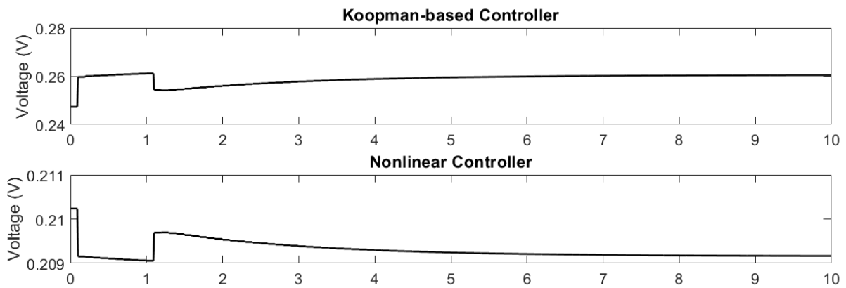
Figure 2.17 – Output Comparison between the MPC signals generated by the Koopman-based and the nonlinear-based approaches.
