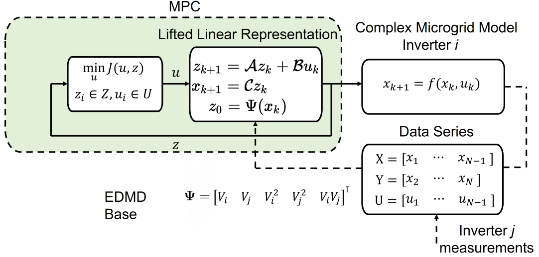
Figure 2.3 – Decentralized Koopman MPC scheme with a linear predictor using EDMD.
