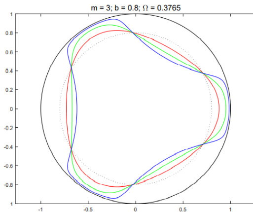
Figure 7: 3-fold V-states for Euler equations in the unit disc [86].
