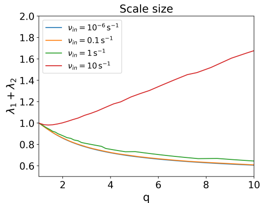
Figure 4.14: Scale size \lambda_1 + \lambda_2 in function of the effective wavelength ratio q = \lambda_1/\lambda_2 in a box of length L = 1 m with g = 1 \text{ m}\cdot\text{s}^{-2} and different value of \nu_{in} .
