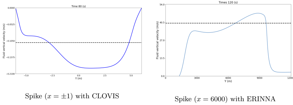
Figure 3.13: On left panel, fluid vertical velocity (solid blue) at x = \pm 1 on Y-axis and analytical terminal velocity of the spike (dashed black). Simulation perform with CLOVIS, with a grid 200 \times 1200 and parameter g = 1 \text{ m.s}^{-2} , r = 2 and \nu_{in} = 2 \text{ s}^{-1} . On right panel, fluid vertical velocity (solid blue) at x = 6000 \text{ m} on Y-axis for spike and analytical terminal velocity (dashed black). Simulation perform with ERINNA, with U_0 = 100 \text{ m.s}^{-1} and r = 3 .
