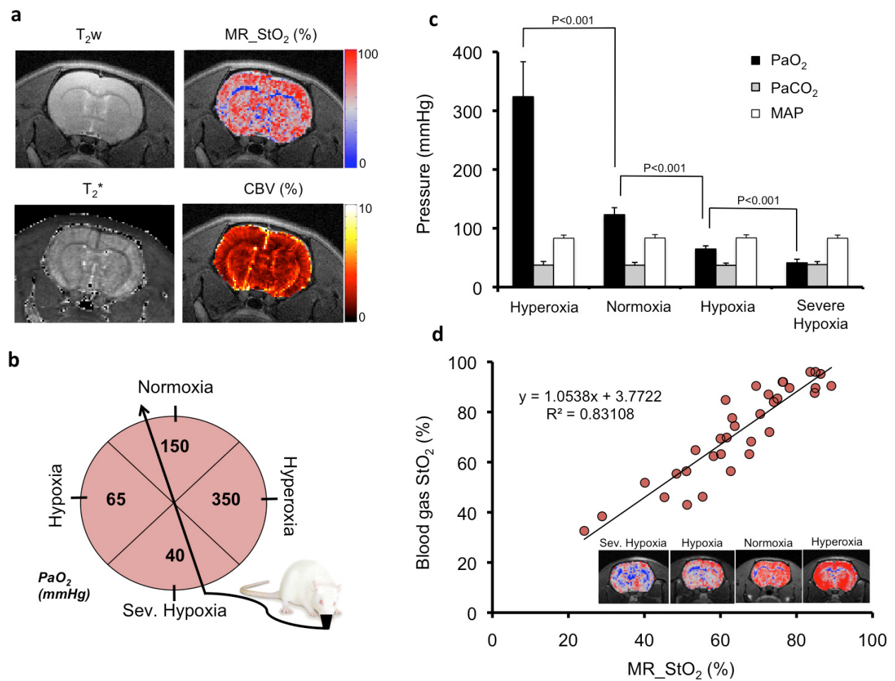
Figure I.3.10: SO_2 measurements during a gas challenge, from Christen et al. 2014a. 17 animals were imaged to measure T_2^* and BVf (CBV in the figure), the latter requiring the injection of a steady-state contrast agent (see Christen et al. 2011). a shows an anatomical scan as well as measured T_2^* , BVf, and SO_2 on one animal under normoxic conditions. b and c show the arterial pO 2 measured from blood sample analysis when varying the amount fraction of inspired O 2 (FiO 2 ). The influence of FiO 2 on the arterial pO 2 during the MR acquisition is clear in c. d shows the correlation between the SO_2 measured on blood samples and with the proposed qBOLD method in a cortical ROI on 17 animals.
