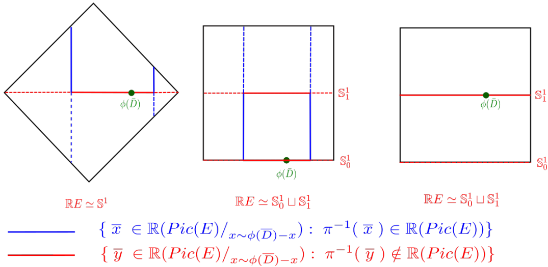
Figure 3.1 – Real divisors in the Picard group \mathbb{R}(Pic(E)/_{x \sim \phi(\bar{D})-x}) of a real elliptic curve with non-empty real part.
