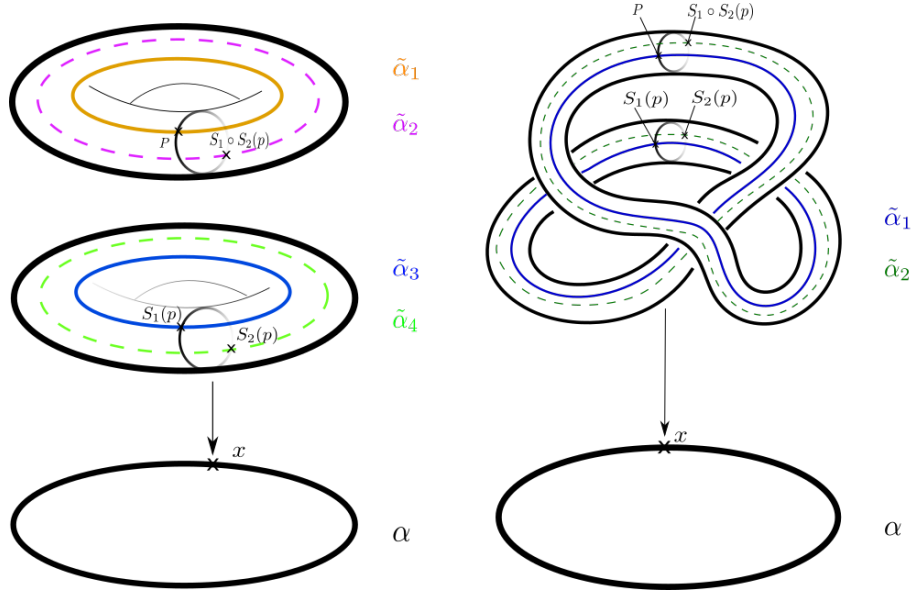
Figure 1.4 – Liftings of an immersed circle C = \text{Im}(\alpha) \subset F to the principal O_2 -bundle O(TF) in two cases: \mathcal{N}_\alpha is orientable (LHS) and \mathcal{N}_\alpha is non-orientable (RHS).
