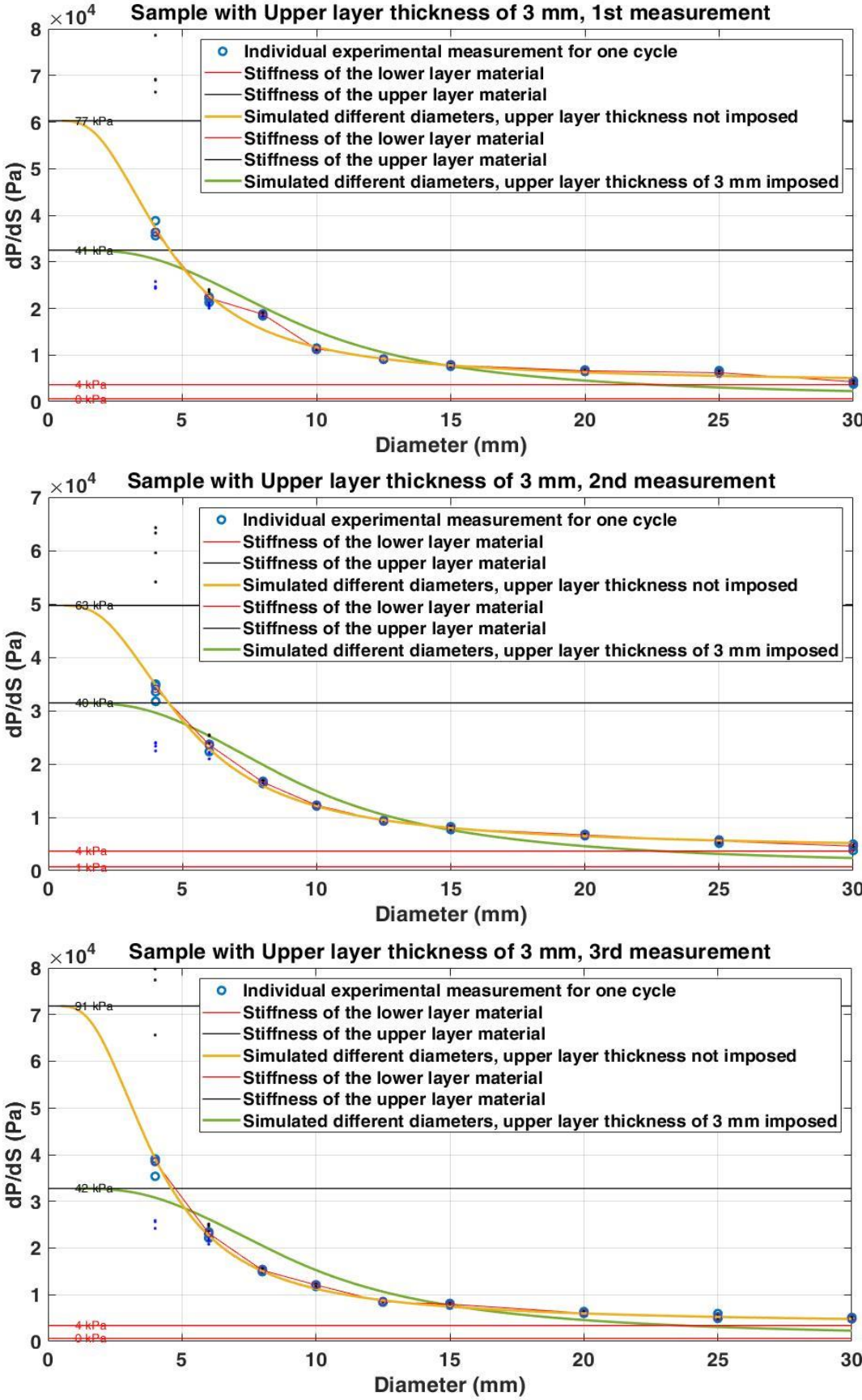
Figure 4 Estimated stiffness of the skin and the adipose tissues for fitting optimisation with and without imposing the skin thickness. Three measurements for subject 2.
