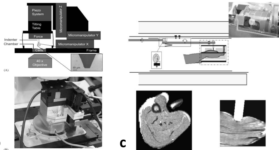
b Figure 5: a ) Experiment on tissue engineered muscle (Gefen et al. 2008) b ) Schematic representation (A) and actual realization (B) of the single cell loading device. The inset shows a close-up of the glass indenter. Adapted from (Peeters et al. 2005) c ) Schematic drawing of experimental set-up (a) Cross sectional T1-Image of the loaded lower leg of a rat (b) Lateral view of the loaded lower leg of a rat (c); adapted from (A. Stekelenburg et al. 2006; Cees W.J. Oomens et al. 2015)
