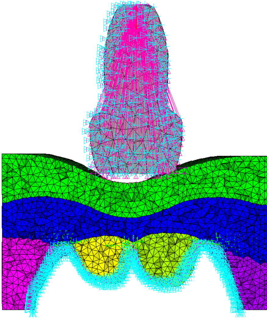
Figure 18: Boundary conditions shown on a transverse cut through the FE model
