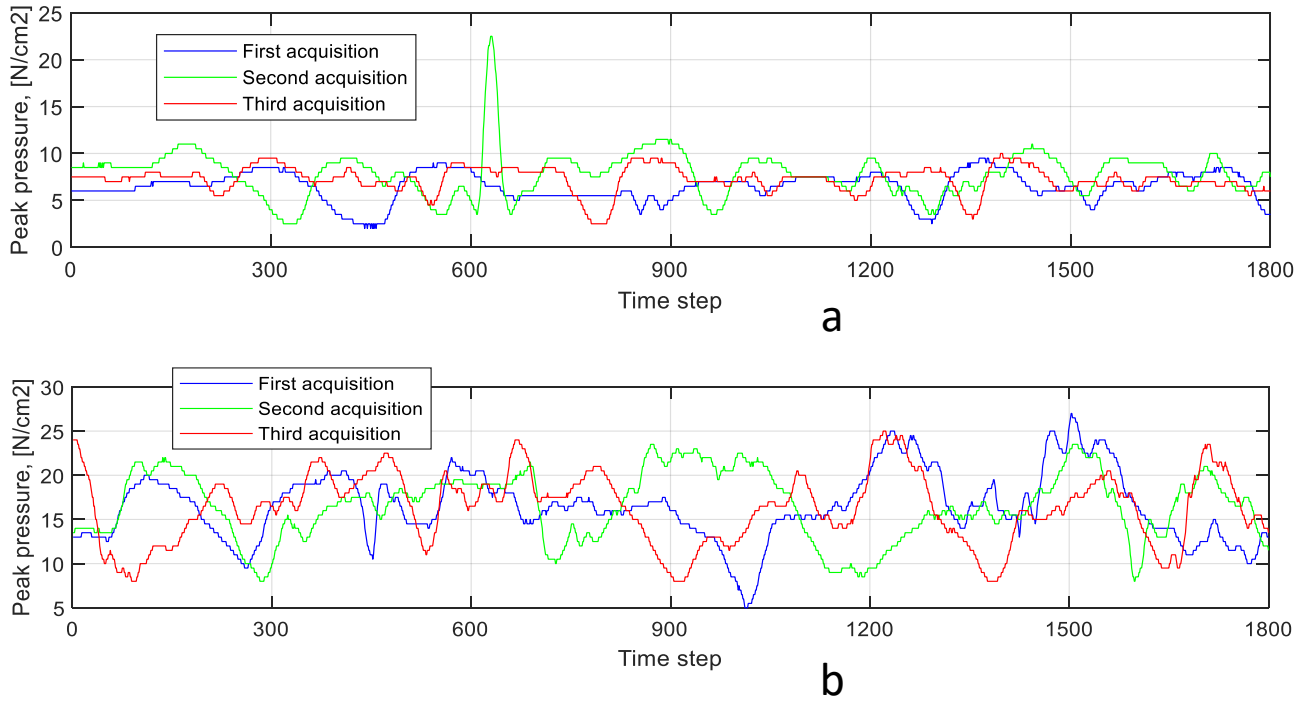
Figure 6 Evolution of the peak pressure for each of 3 acquisitions. a) Subject 1 b) Subject 2
