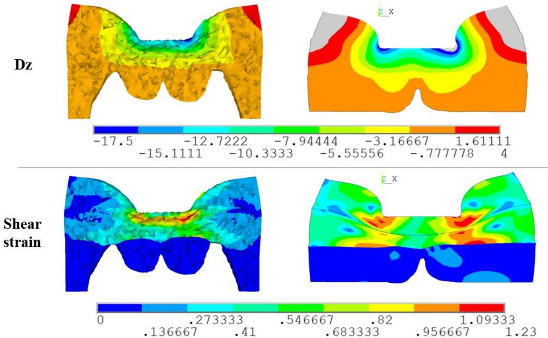
Figure 30: Vertical displacement (top row) and shear strain (bottom row) for 2D model (right) and 3D model (left), Load case I (~1200 g)
