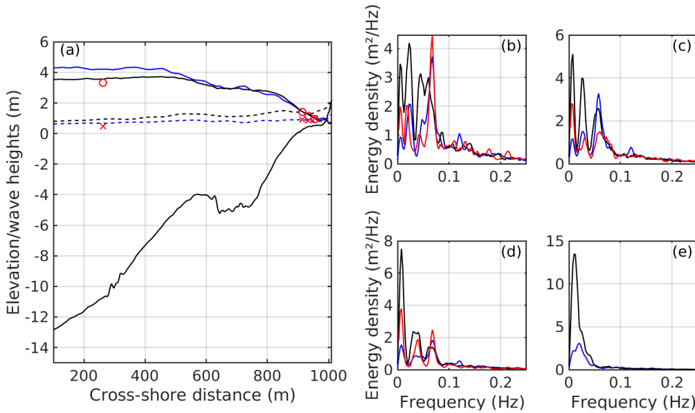
Figure 4.4: (a) : Significant wave heights H_{SW} (solid line, circles) and H_{IG} (dashed line, crosses) for the observations (red) the 1D (black) and 2D (blue) configuration. (b) , (c) , (d) wave spectra at the deepest to shallowest pressure sensors locations (CP07, CP06, CP05) and (e) at the shallowest submerged location of the observations (red), 1D (black) and 2D (blue) configurations.
