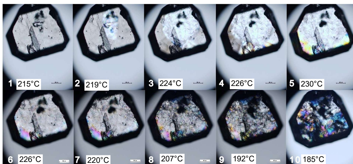
Figure A-1-EDS crystals seen under polarized light microscope (NIKON Eclipse LV100) upon heating (1-5) and upon cooling (6-10)
