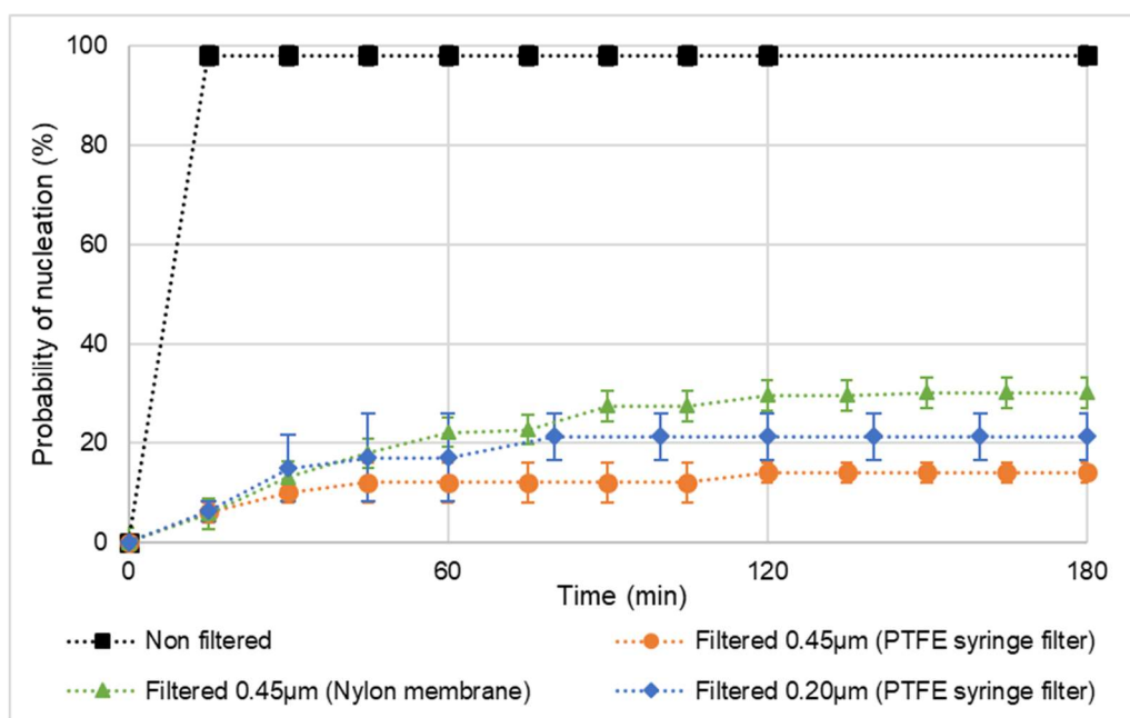
Figure 5-8-Evolution of the probability of nucleation versus time of irradiated aqueous EDS solutions ( \beta=1.10 ) filtered by different methods (filtered with nylon membrane 0.45 \mu m; PTFE syringe filter of 0.45 \mu m and 0.2 \mu m). (For non-filtered solution error bars are smaller than the size of the squares)
