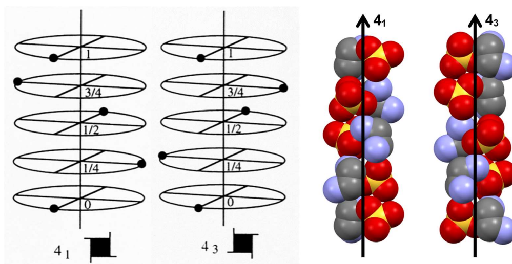
Figure 5-1-Representation of helical axes 4_1 and 4_3 in schematic (left) and in the EDS structure (hydrogen atoms omitted for clarity, right)
