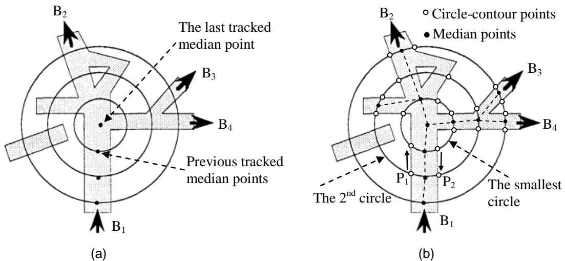
Figure 1.29: The branch construction process: (a) circle following; (b) branch construction; (reproduced from [Van Nieuwenhuizen and Bronsvoort, 1994]).
