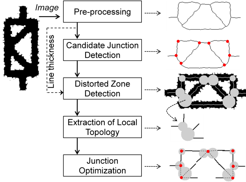
Figure 2.1: Overview of the proposed approach.
