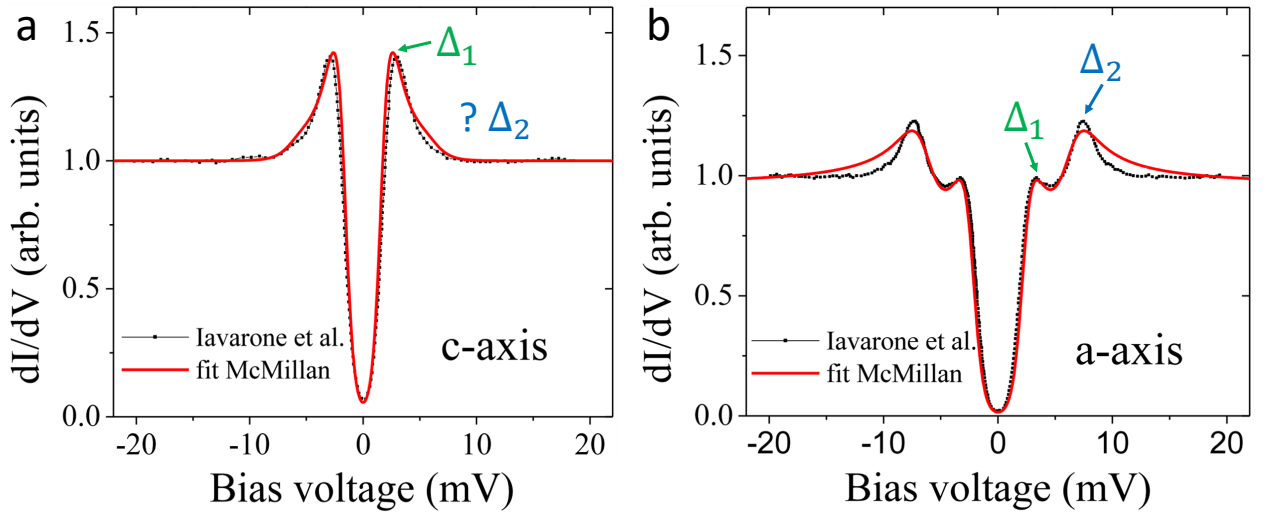
Figure 2.5: a. dI/dV spectrum taken on \text{MgB}_2 with the tip aligned along the c -axis. b. dI/dV spectrum taken on \text{MgB}_2 with the tip aligned along the a -axis. Figure taken from [70].
