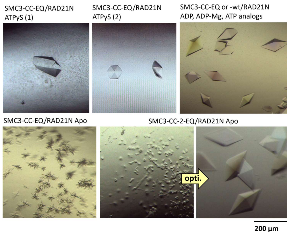
Figure 30: SMC3-CC-EQ/RAD21N and SMC3-CC-2-EQ/RAD21N crystals. Typical crystal shapes obtained for the SMC3-CC-EQ/RAD21N constructs in the presence of ADP, ATPγS, and the intermediate ATPase cycle analogs (ADP.BeF 3 , ADP.VO 4 and ADP.AlF 3 ) (top and bottom left panels). SMC3-CC-2-EQ/RAD21N crystals were obtained in absence of ligand, and optimized into large 3D and X-ray diffracting crystals (bottom right).
