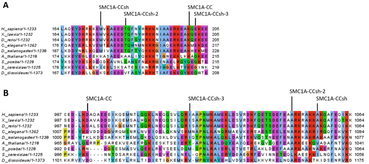
Appendix 1: Sequence alignment of the SMC1A from different organisms. The sequence boundaries of the human SMC1A ATPase head constructs are indicated, at (A) their N-terminal end and at (B) their C-terminal end.
