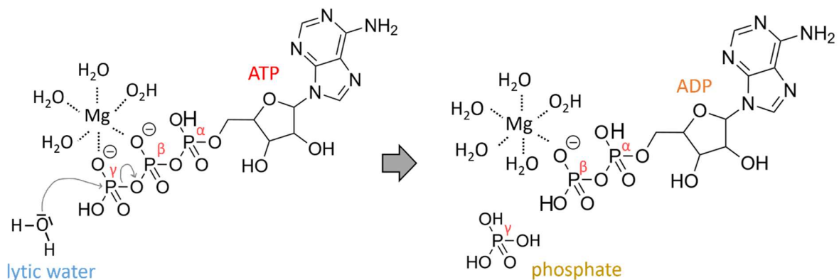
Figure 14: Mechanism of ATP hydrolysis into ADP and P_i . The gamma phosphate of the ATP molecule is attacked by an activated water molecule, which promotes debracketage of the gamma phosphate-beta oxygen bond and the release of phosphate. The cofactor Mg^{2+} ion assists and promotes the hydrolysis reaction. In ATPase proteins, the lytic water molecule is activated by a catalytic residue, usually a glutamate, and some of the hydrogen bonds formed by the water molecules coordinating the Mg^{2+} are replaced by the protein's residues to stabilize the ATP- Mg^{2+} inside the active site.
