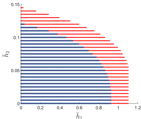
Figure 2.9: Feasible values of \bar{h}_1 and \bar{h}_2 , when \bar{\eta}_1 = \bar{\eta}_2 = 0.075 , for the large-delay case (in blue) and the small-delay case (in red). For the small-delay case, the bounds \bar{h}_1 < 0.075 and \bar{h}_2 < 0.075 are applicable only if the condition (2.114) is satisfied.
