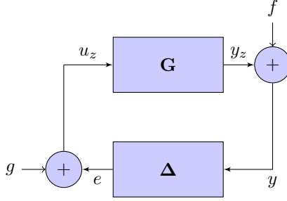
Figure 2.5: Standard feedback interconnection of two exemplary operators \mathbf{G} and \mathbf{\Delta} , which will be used to represent the decentralized system (2.30)-(2.33).
