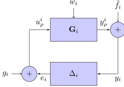
Figure 2.6: The feedback interconnection of \mathbf{G}_i and \Delta_i , representing the i^{th} closed-loop \Sigma_i - K_i .
