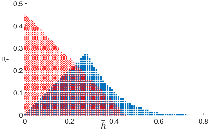
Figure 3.1: Feasible values of \bar{h} and \bar{\tau} for the nonlinear system (3.41) with \alpha = 0.1 , in the large-delay case (in red), and in the small-delay case (in blue).
