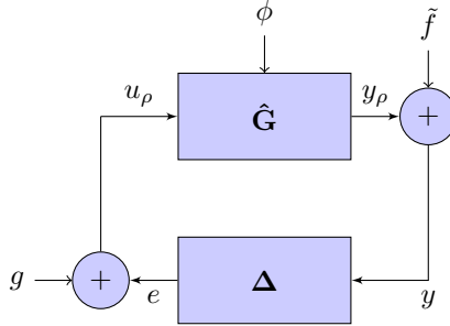
Figure 2.7: The feedback interconnection of \hat{\mathbf{G}} and \Delta , representing the decentralized system (2.30)-(2.33).
