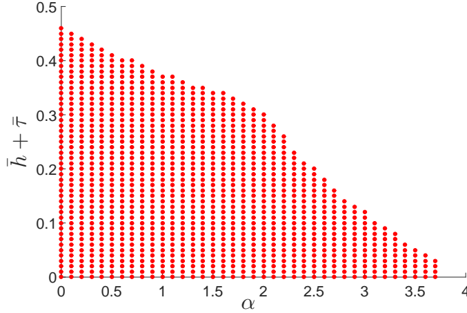
Figure 3.2: Trade-off between desired decay-rate \alpha and \bar{h} + \bar{\tau} for the nonlinear system (3.41), in the large-delay case.
