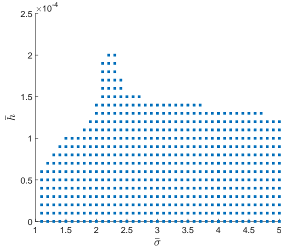
Figure 4.3: Trade-off between coupling strength \sigma and maximum sampling interval \bar{h}_1 = \bar{h}_2 = \bar{h}_3 = \bar{h} , for the three-agent Fitzhugh-Nagumo system, with \alpha = 0.01 .
