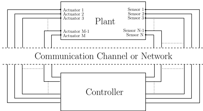
Figure 1.2: A generic representation of networked sensing and actuation in single plant-controller setup with N sensors and M actuators. The plant-controller, and controller-plant information transmission is via a communication channel. In the scope of Figure 1.1, the individual sub-systems could have such a configuration and the communication channel could be shared with other subsystems with similar configuration.
