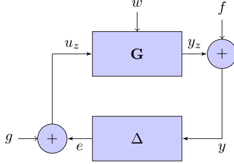
Figure 2.2: The feedback interconnection of \mathbf{G} and \Delta
