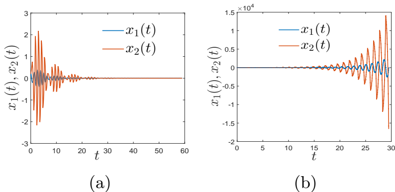
Figure 2.1: (a) The decentralized LTI system (2.1) is stable for synchronous sampling with T = 0.59 . (b) Stability is lost when x_2(t) is sampled asynchronously with respect to x_1(t) with a shift of \delta = 0.2 .
