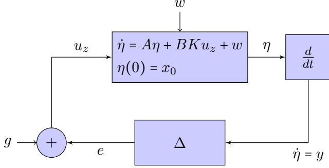
Figure 2.3: The feedback-interconnection used as an intermediate while transitioning from system (2.2),(2.3) to system (2.7)-(2.10), as shown in proof of Theorem 2.1.
