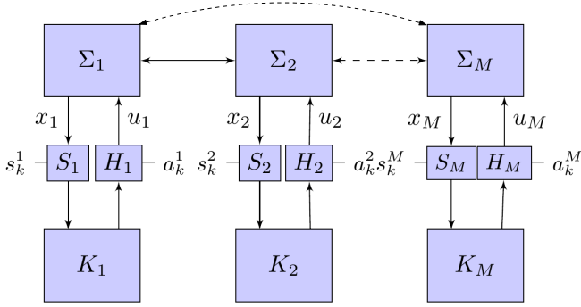
Figure 2.4: A decentralized controller setup example. S_i and H_i , for all i \in \{1, 2, \dots, M\} , denotes the sample and hold components, respectively, for the i^{\text{th}} closed-loop.
