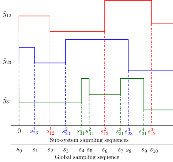
Figure 4.1: At the global level, between any two sampling instants s^k , all the transmitted signals over the network are constant. This is illustrated using exemplary transmitted signals \hat{y}_{12} , \hat{y}_{23} and \hat{y}_{31} in a three-agent network connected via a ring topology.
