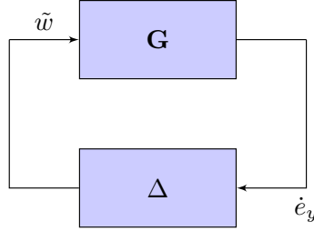
Figure 4.2: The feedback interconnection of \mathbf{G} and \Delta , representing the synchronization error dynamics of system (4.42), (4.4).
