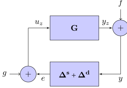
Figure 2.8: The feedback interconnection of \mathbf{G} and \Delta^s + \Delta^d , representing the decentralized system (2.30)-(2.33).
