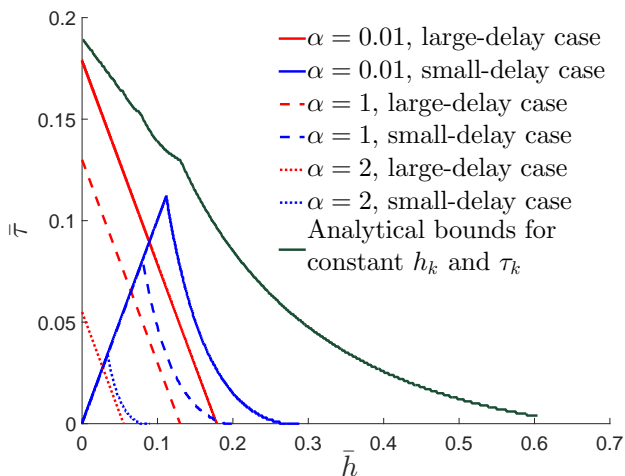
Figure 3.3: Bounds on \bar{h} and \bar{\tau} for the LTI system (3.51) in the large-delay case (in red), and in the small-delay case (in blue), for \alpha = 0.01 (solid line), \alpha = 1 (dashed line) and \alpha = 2 (dotted line). The analytical stability bounds on constant h_k and \tau_k are given by the green line [134].
