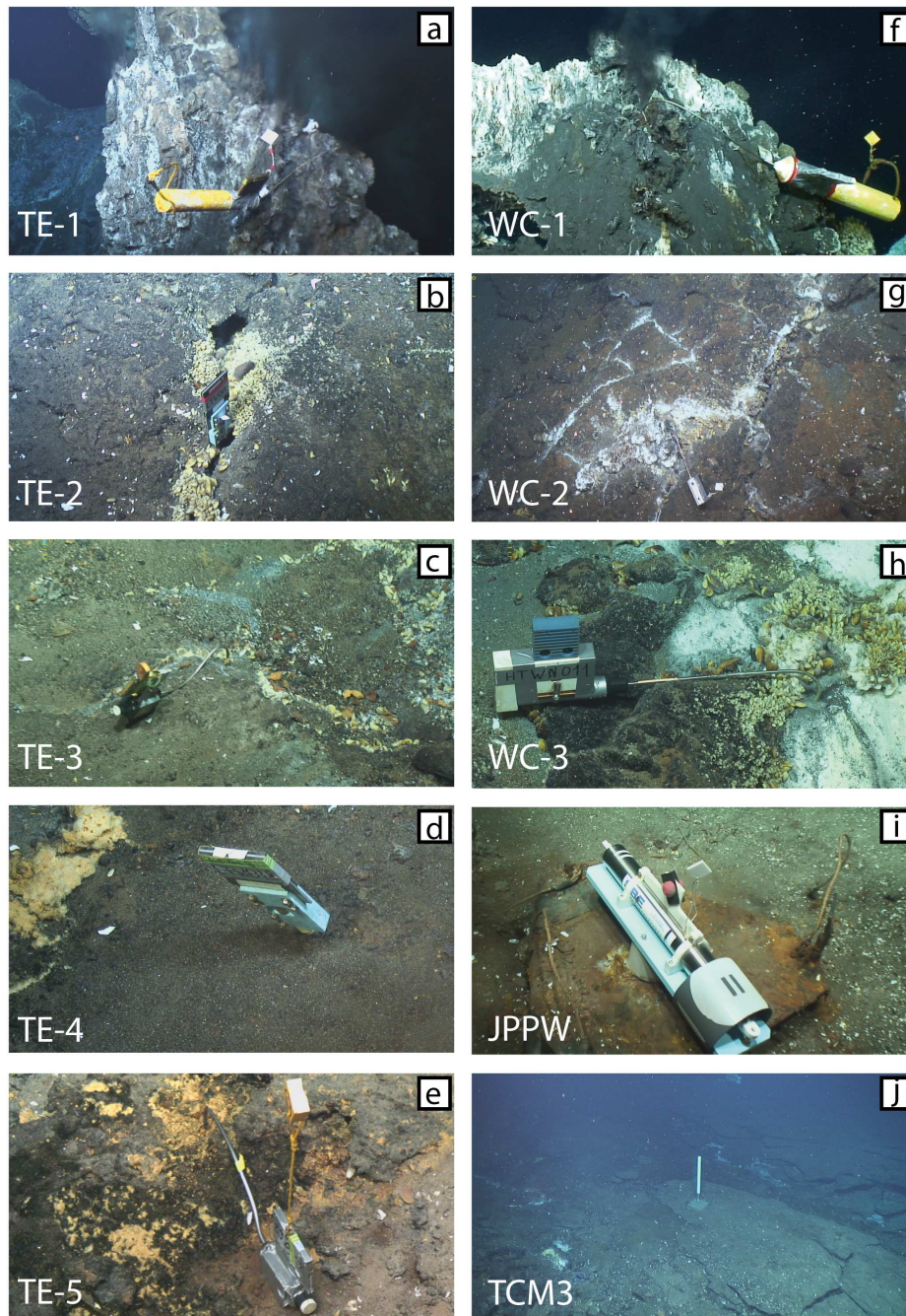
Figure 4-3 – ROV video snapshots showing examples of the temperature probes (a to h; see location in the Tour Eiffel and White Castle maps of Figure 4-4), pressure probes (i), and currentmeters (j) deployed at the LSHF as part of our monitoring experiment. (a) high-temperature WHOI (HTW) probe deployed in 2017 at focused vent (monitoring location TE-1). (b) low-temperature WHOI (LTW) probe deployed in 2017 in crack of sulfide-indurated slab (monitoring location TE-2); note bacterial mats and mussel assemblage. (c) high-temperature NKE (HTNKE) probe deployed in 2018 in mussel-lined crack of non-indurated slab (monitoring location TE-3). (d) LTW probe deployed in 2017 in brownish sandy area next to yellow iron-oxidizing bacterial mats (monitoring location TE-4). (e) LTW probe deployed in 2018 in vent nested in yellow iron-oxidizing bacterial mats (monitoring location TE-5). (f) HTW probe deployed in 2017 at focused vent (monitoring location WC-1). (g) HTNKE probe deployed in 2016 in crack in sulfide-indurated slab (monitoring location WC-2). (h) new high-temperature WHOI (HTWN) probe deployed in 2017 in sandy area next to sulfide-indurated slab (monitoring location WC-3); note mussels on slab material and white barite precipitates and bacterial mats in sandy diffuse venting area. (i) SBE53 pressure probe deployed in 2018 at the JPPW benchmark (Figure 4-1). (j) TCM3 currentmeter deployed in 2016 on non-indurated layered volcanoclastics (slab) to the south of Tour Eiffel (Figure 4-1).
