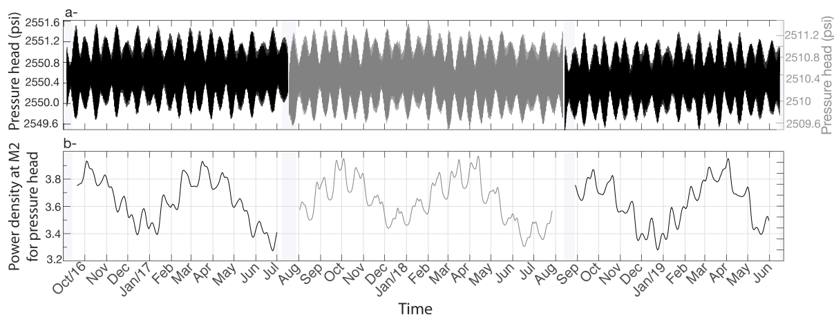
Figure S4-3 – Time variation of seafloor pressure (a) and of the power spectrum density (PSD) of seafloor pressure at the M2 frequency (b) over the 3 years of the experiment. Values for deployment years 2016-2017 and 2018-2019 are shown in black, values for deployment year 2017-2018 in grey (different location; see Figure 4-1). PSD values in b are calculated for a 30 days sliding window, 1 day sliding time.
