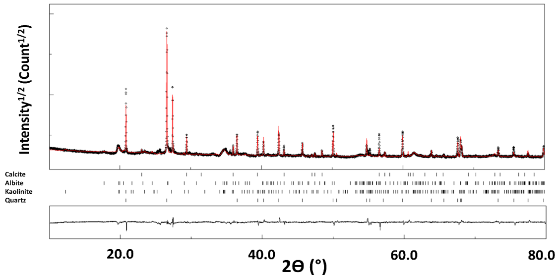
Figure 3-12 XRD pattern of structural soil. On top of the observed profile, the computed pattern (red line) is superimposed (black dots). At the bottom is the difference curve ( I_{\text{obs}} - I_{\text{calc}} ).
