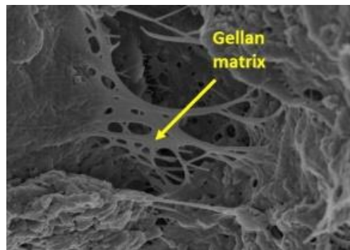
Figure 1-11 Scanning electron microscope (SEM) of stabilized soil by gellan gum
