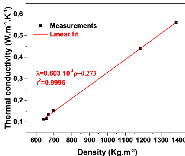
Figure 3-20 Density of the cob specimens versus thermal conductivity
