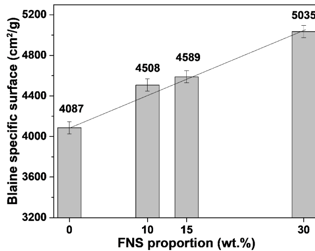
Figure 2-5 Evolution of the Blaine specific surface area (SSA) of the cements elaborated with FNS.
