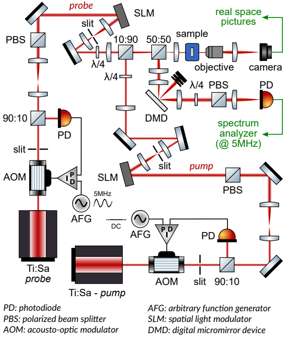
Figure 3.2: Pump-probe spectroscopy. Experimental setup. The sample is placed in a helium cryostat cooled down to 3.8K. Two cw Ti:Sa lasers illuminate it, with the same circular polarization to excite a single spin state. The pump injects a high density fluid in the area of its 100\mu\text{m} diameter waist in the plane of the sample. Its intensity I_P is controlled by mean of a proportional-integral-derivative loop (PID) which feedbacks on the RF amplitude of an acousto-optic modulator (AOM). Its phase and intensity profiles can be reshaped with a spatial light modulator (SLM), imaged in the sample plane. The probe is recombined with the pump beam thanks to a 90:10 beam splitter. Its waist in the sample plane has a diameter of about 50\mu\text{m} and an intensity of about 0.1% of I_P . Its wavevector \mathbf{k} is monitored with an SLM, also imaged in the cavity plane, displaying a blazed grating of controllable step size, to change the angle of the first diffraction order, filtered by means of an automatically tunable position slit in the reciprocal space. Its amplitude is modulated with an AOM at f_{mod} = 5 MHz, also slaved with a PID loop. The reflection of the cavity is recovered using a 50:50 beam splitter, placed just before the cavity. A DMD in the reciprocal space displays a pinhole of configurable position and size selecting the wavevectors of the signal sent to the detection. In addition, a quarter-wave plate and a PBS operate a polarization selection, to recover only the same polarization state as the pump and the probe. The signal is then focused on a photodiode (PD) and demodulated at f_{mod} with a spectrum analyzer to isolate the probe signal from the pump signal. The transmission of the probe can be easily deduced from this scheme. (a) Principle of pump-probe spectroscopy: the pump (yellow square), creates a high density fluid, of dispersion relation depicted by the black lines. The probe scans the resonances of the fluid (red squares), at a fixed \mathbf{k} , over an energy range of 150 GHz (red vertical arrow). (b) When the probe resonates with the positive branch, a Lorentzian reflectivity dip appears in the reflection signal. The position of the minimum and the full width at the half height of the dip give the real and imaginary parts of the energy of the Bogoliubov mode respectively. In transmission, the signal trace features a Lorentzian peak instead of a dip.
