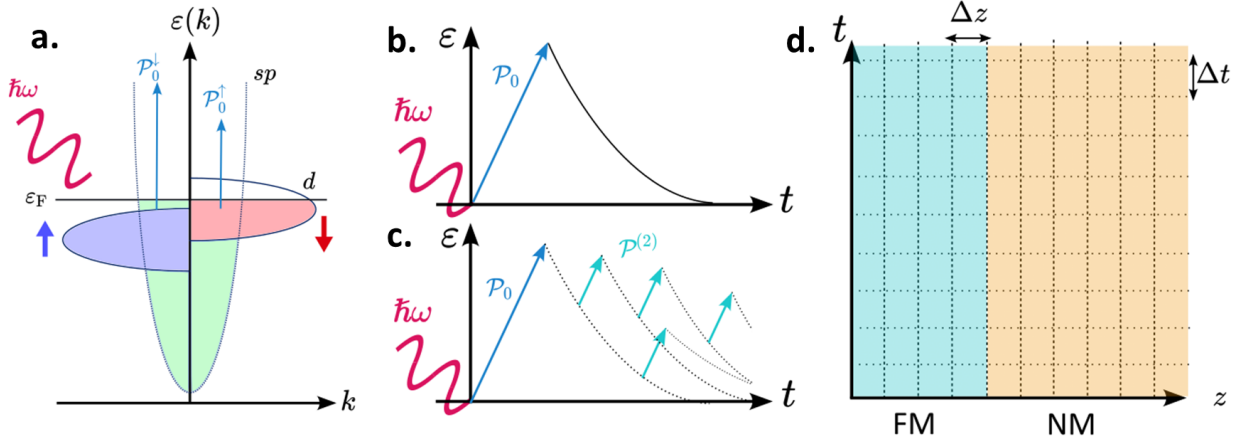
Figure 3.1: Illustration of the excitation and relaxation mechanisms. (a) Representation of the photoexcitation of hot spin electrons via the d \rightarrow sp transition. Scheme of the electronic energy vs. time for (b) the diffusive relaxation processes and (c) the superdiffusive relaxation processes. (d) Representation of the finite difference time domain resolution principle.
