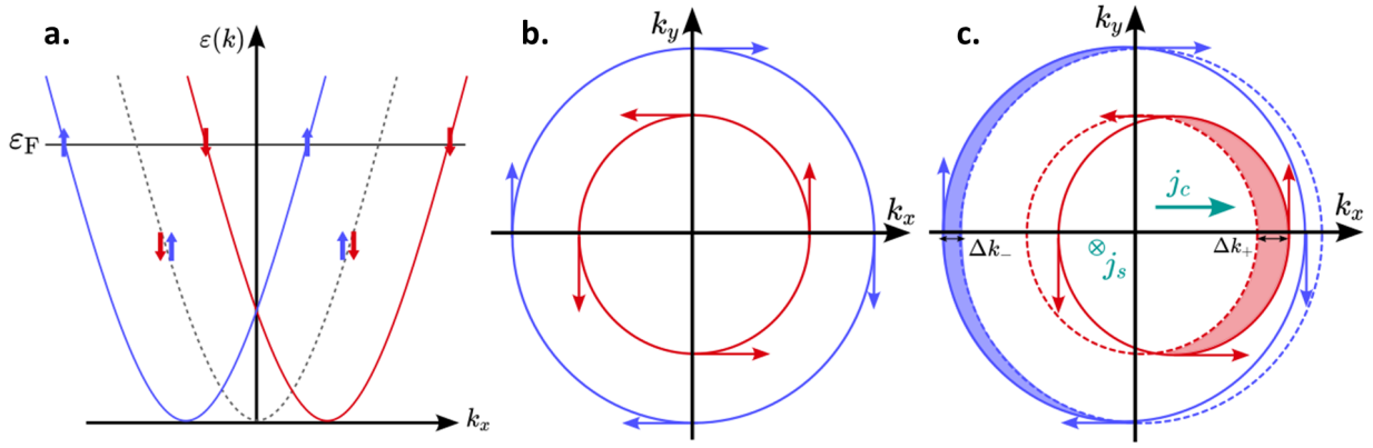
Figure 1.9: Inverse Rashba-Edelstein conversion for a 2DEG system. (a) Degenerated (dotted line) and lifted degeneracy for the free electron dispersion relation, with the Fermi level noted as \epsilon_F . (b) Fermi contour presented in k_x, k_y space with textured opposed bands. (c) Under the application of a spin-current propagating along e_z and polarized along e_y , the Fermi contour shifts from \Delta k_x .
