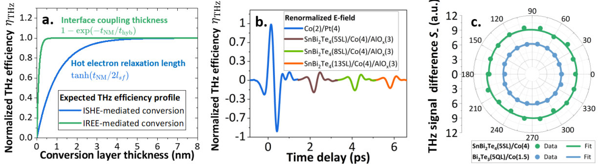
Figure 4.13: Interfacially-mediated interconversion. (a) Expected THz efficiency thickness profile for ISHE (bulk) interconversion (blue) vs. IREE (interface) interconversion. (b) Experimental thickness dependence of the THz efficiency on SnBi 2 Te 4 ( t_{\text{TI}} )/Co(4) for t_{\text{TI}} ranging from 5, 8 and 13 SLs, compared to Co(2)/Pt(4). (c) Angular conversion profile of the magnetic component in SnBi 2 Te 4 /Co (green) and Bi 2 Te 3 /Co (light blue).
