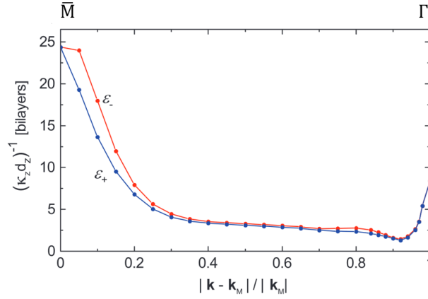
Figure 4.4: Evanescence of the topological surface states. Decay length of the two TSS (blue and red) of \text{Bi}(111) along the \Gamma\bar{M} direction. Adapted from Ref. [283].
