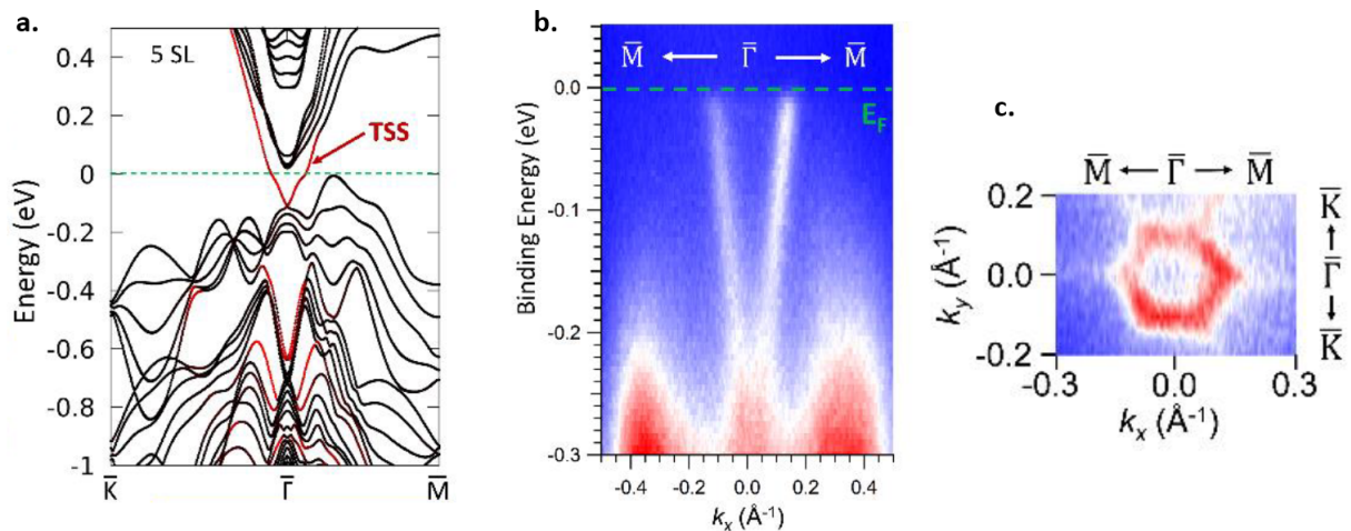
Figure 4.6: Band structure of SnBi 2 Te 4 . (a) Calculated band structure for SnBi 2 Te 4 (5SL) presenting the topological surface states crossing (red) at the Fermi level (dotted green line). (b) Band dispersion along the \bar{\Gamma} - \bar{M} direction in SnBi 2 Te 4 (5SL). (c) Experimental Fermi surface presenting an hexagonal shape in SnBi 2 Te 4 (5SL).
