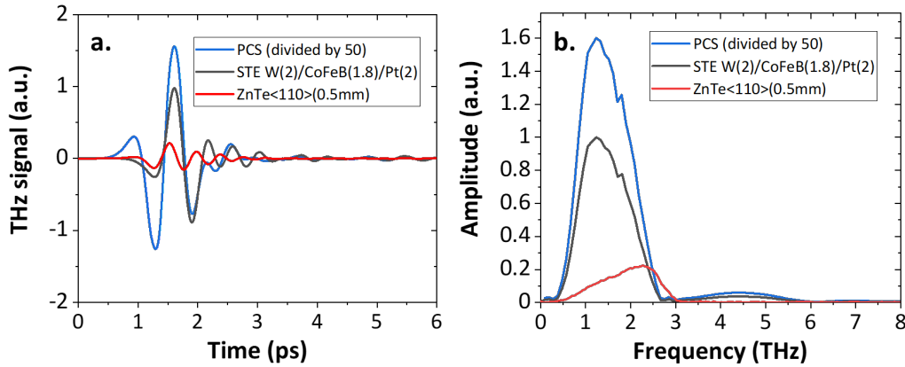
Figure 3.18: Comparing STE with actual pulsed THz technologies. (a) THz emission from a ZnTe(110)(500 \mu m), a photoconductive switch (PCS) and the reference spintronic trilayer W(2nm)/CoFeB(1.8nm)/Pt(2nm). (b) Measured bandwidth for the three systems. The amplitudes are normalized with respect to the spintronic emitter. Note that the THz amplitude of the PCS is divided by a factor \times 50 .
