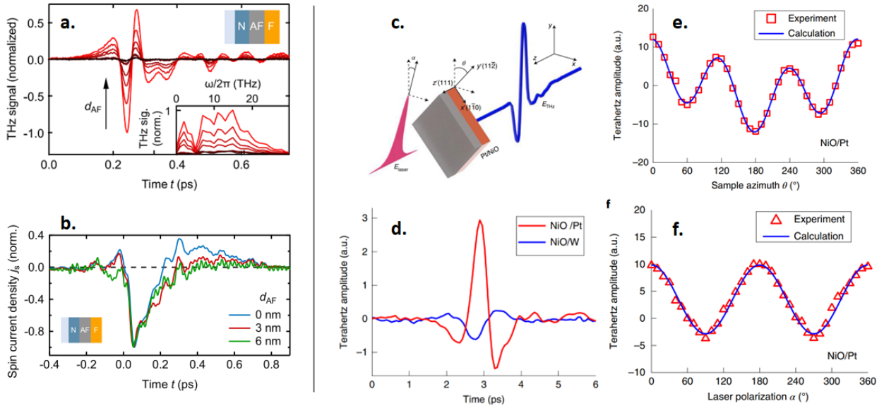
Figure 2.12: Antiferromagnetic-based THz heterostructures. (a). THz signal from Pt/IrMn( d_{AF} )/NiFe structures with d_{AF} ranging from 0 to 12 nm, and (b) derived ultrafast spin current for d_{AF} = \{0, 3, 6\} nm. (c) THz emission spectroscopy of NiO/Pt bilayers in transmission geometry. (d) THz signals from NiO/Pt and NiO/W. (e) THz amplitude as a function of the sample azimuthal angle and (f) pump polarization angle from NiO/Pt bilayers. Left and right panels are respectively adapted from Refs. [191, 194].
