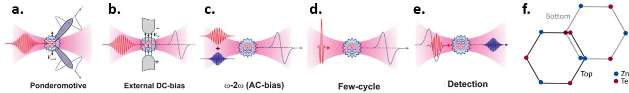
Figure 2.7: Air-plasma and non-linear crystal THz emission. (a-e) Representation of the different THz generation and detection schemes using femtosecond laser plasma filaments. (f) Surface of a zinc-blende non-linear crystal (e.g. ZnTe) who presents a distortion of the top unit cell which reinforces the bulk optical rectification upon ultrashort pumping. Left panels adapted from Ref. [129].
