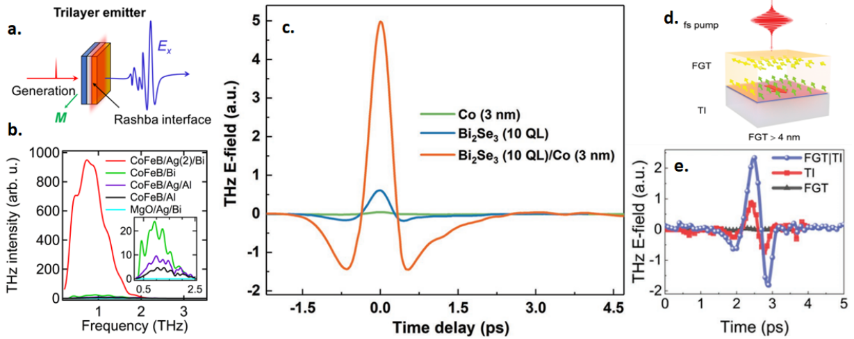
Figure 2.10: Interfacially-based spintronic THz emitters. (a) Schematics of interfacial THz emitter based on Rashba interface. (b) THz emission from CoFeB/Ag/Bi compared to CoFeB/Bi, CoFeB/Ag/Al, CoFeB/Al and Ag/Bi control samples. A strong amplification by a factor \times 50 is measured experimentally. (c) THz emission based on topological insulator \text{Bi}_2\text{Se}_3/\text{Co} compared to \text{Bi}_2\text{Se}_3 and Co control samples. (d) Schematics of topological insulator/2D ferromagnet THz structure. (e) THz emission from \text{Fe}_3\text{GeTe}_2/\text{Bi}_2\text{Te}_3 compared to THz emission from pure \text{Bi}_2\text{Te}_3 and \text{Fe}_3\text{GeTe}_2 . Left, middle and left panels are respectively adapted from Refs. [161, 163, 169].
