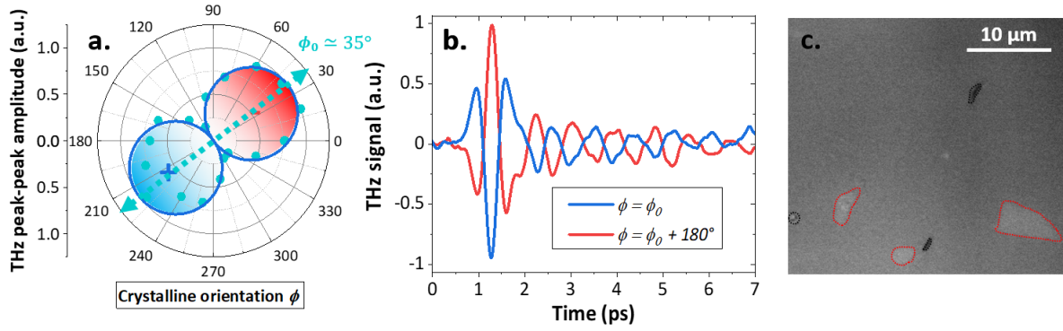
Figure 5.6: Crystallographic dependence of the THz emission in NiO(001)(10nm)/Pt(2nm). (a) THz peak-peak amplitude as a function of \phi ranging from 0^\circ to 360^\circ . (b) Time traces of the THz phase reversal taken at \phi = \phi_0 and \phi = \phi_0 + 180^\circ . (c) Kerr imagery of the large AFM quasi-mono domain states. The small white domains, of different orientation compared to the large mono grey domain, are highlighted in red. Defects appear in black.
