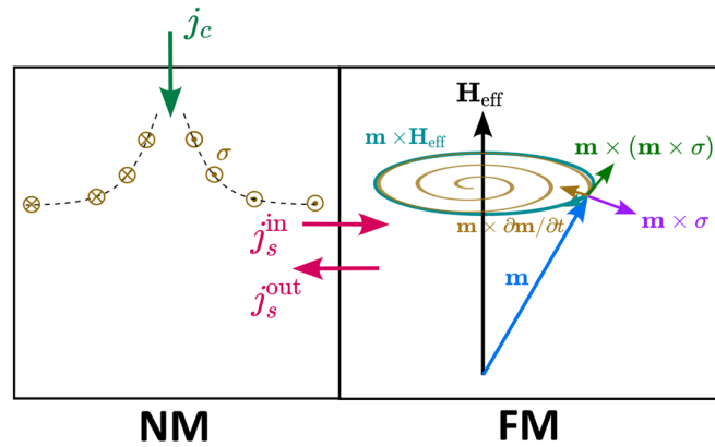
Figure A12.1: Spin-orbit torque. An injected charge current j_c is converted in a strong SOC material into a spin-polarized current j_s^{\text{in}} injected into a neighbouring ferromagnet. The spin current transfers part of its angular momentum to the magnetization \mathbf{m} via the action of the damping-like torque \mathbf{m} \times (\mathbf{m} \times \sigma) and field-like torque \mathbf{m} \times \sigma , inducing magnetization precession and concurrent spin pumping j_s^{\text{out}} .
