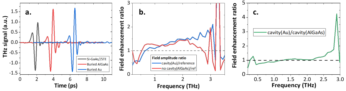
Figure 6.4: Experimental buried cavity-based STEs. (a) Measured THz emission from AlGaAs (red) and Au (blue) based buried THz cavities. The reference sample is SI-GaAs//STE (black). (b) Enhancement ratio (electric field) presented in the frequency domain. An enhancement around +30% is reported experimentally. (c) Experimentally measured ratio between the two enhancements from Au based cavity and AlGaAs based cavity demonstrating specifically an enhancement at higher frequencies (from 2 to 3 THz) of +50% on Au based buried cavity compared AlGaAs based cavity.
