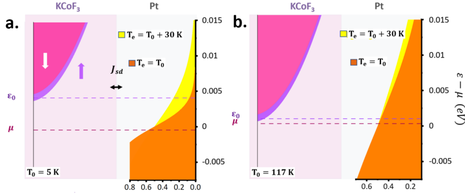
Figure 5.21: Addressing the sub-picosecond spin-Seebeck effects in antiferromagnets. (a-b) Scheme of the band diagram of \text{KCoF}_3/\text{Pt} bilayer, respectively below and close to the Néel transition T_N . The photo-excited electronic population (in yellow is the electronic population spreading in energy) induces an interfacial transfer of the energy via the exchange J_{sd} exciting the spin-split magnon population of \text{KCoF}_3 (pink and violet), only in the temperature region where \varepsilon_0 > \mu_e (where \mu_e is the chemical potential), either induced by the antiferromagnet temperature T or by the equivalent fluence-increased electron energy spreading. This model can be seen as the linear spin-Seebeck effect. Adapted from Ref. [366].
