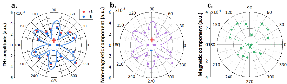
Figure 4.43: Reference THz emission symmetry measurements on \text{Bi}_2\text{Se}_3/\text{WSe}_2/\text{AlO}_x . (a) Measured THz emission from \text{Bi}_2\text{Se}_3(10\text{QL})/\text{WSe}_2(3\text{ML})/\text{AlO}_x(3\text{nm}) as a function of azimuthal angle \phi , for +B and -B with extracted (b) non-magnetic component and (c) magnetic component. The amplitude is presented as a fraction of \text{Co}(2\text{nm})/\text{Pt}(4\text{nm}) reference.
