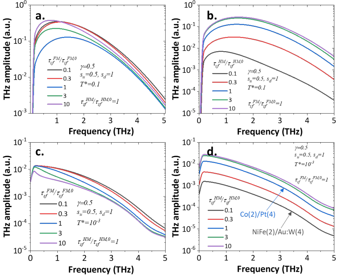
Figure 3.6: Impact of the spin scattering timescale. (a-b) Evolution of the THz amplitude as a function of (a) \alpha_{\text{FM}} and (b) \alpha_{\text{HM}} for the conventional case of Co/Pt interface with an interfacial transmission coefficient T^* = 0.1 . (c-d) Evolution of the THz amplitude as a function of (c) \alpha_{\text{FM}} and (d) \alpha_{\text{HM}} in the confined case defined for a transmission coefficient about T^* = 10^{-3} . The pump duration is \tau_p = 100 fs and the bilayer is Co(2)/Pt(4) and the spin-asymmetry is \gamma = +0.5 .
