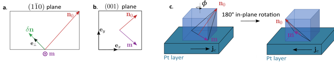
Figure 5.7: Projection of the initial Néel vector \mathbf{n}_0 , its dynamical variations \delta\mathbf{n} and the induced magnetization \mathbf{m} in the (a) (1\bar{1}0) and (b) (001) plane. (c) To understand the crystallographic dependence results, we represent the rotation of the Néel vector (thus induced magnetization) by \phi=180^\circ .
