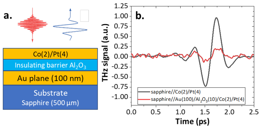
Figure A16.1: THz reflector using an insulating barrier and a metallic plane. (a) Schematics of the structure delimited by a \text{Al}_2\text{O}_3(10\text{nm}) insulating barrier and a \text{Au}(100\text{nm}) plane. (b) THz emission from sapphire//Au(100nm)/ \text{Al}_2\text{O}_3(10\text{nm}) /Co(2nm)/Pt(4nm) reflector compared to reference sapphire//Co(2nm)/Pt(4nm)
