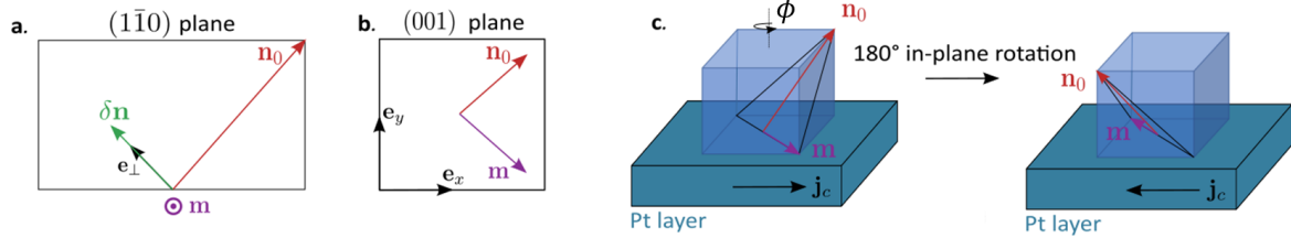
Figure 5.7: Projection of the initial Néel vector \mathbf{n}_0 , its dynamical variations \delta\mathbf{n} and the induced magnetization \mathbf{m} in the (a) (1\bar{1}0) and (b) (001) plane. (c) To understand the crystallographic dependence results, we represent the rotation of the Néel vector (thus induced magnetization) by \phi=180^\circ .
