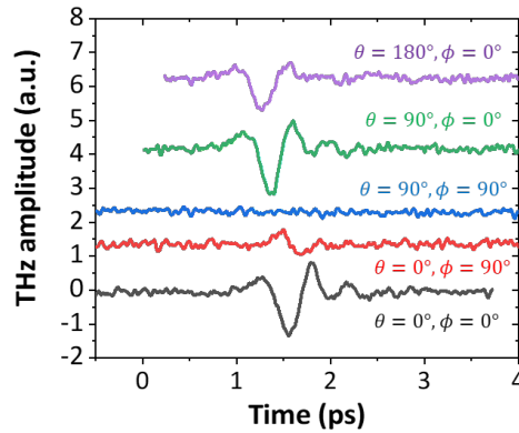
Figure 5.24: THz emission from \alpha -Fe 2 O 3 /Pt bilayer. THz emission from \alpha -Fe 2 O 3 (500 \mu m)/Pt(10nm) bilayer as a function of the magnetic field orientation ( \theta ) and crystalline orientation ( \phi ) from the initial magnetic moment direction.
