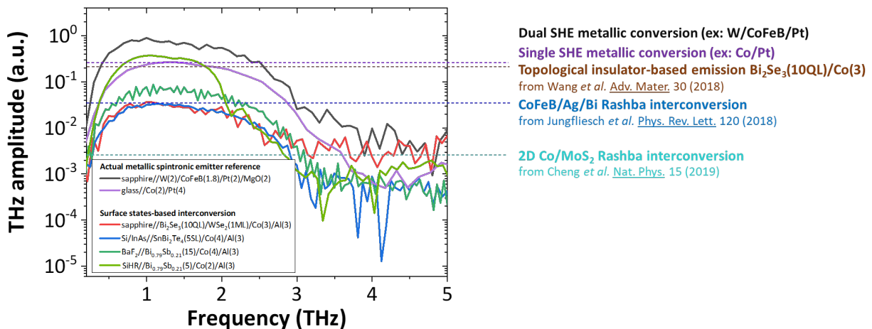
Figure 4.36: Comparison of the different topological insulators-based and 2D-based spintronic THz emitters studied in the frame of this thesis work. Emitted radiation presented in the spectral domain, from interfacially-mediated \text{Bi}_{1-x}\text{Sb}_x/\text{Co} , \text{Bi}_2\text{Se}_3/\text{Co} , \text{Bi}_2\text{Te}_3/\text{Co} and \text{SnBi}_2\text{Te}_4/\text{Co} compared to metallic spintronic THz emitters W/CoFeB/Pt and Co/Pt and sources developed in the literature.
