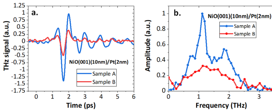
Figure 5.8: Impact of the magnetic quality on the THz emission. (a) THz signal in time-domain for sample A and sample B, grown respectively at low (0.7 sccm) and high (1.5 sccm) O_2 gas flow. (b) Spectra of the measured THz signal where the 1 THz oscillation mode could not be mapped in sample B.
