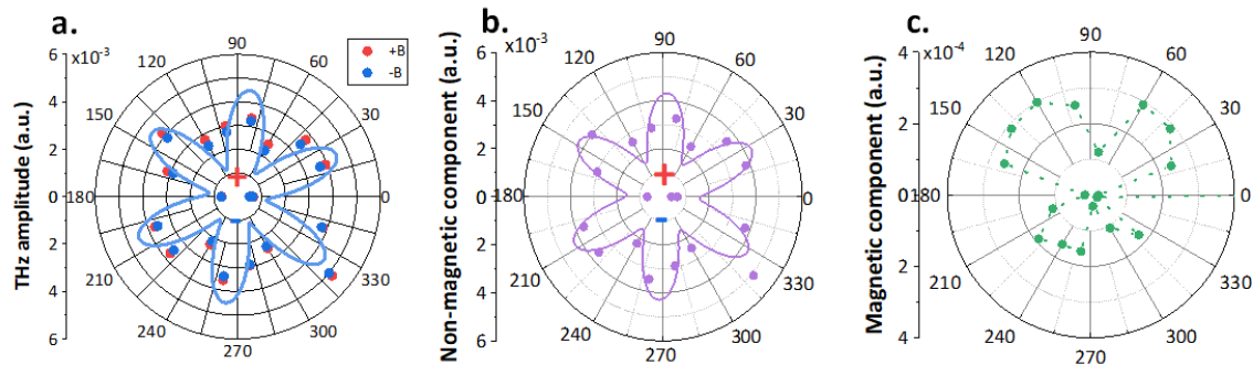
Figure 4.43: Reference THz emission symmetry measurements on \text{Bi}_2\text{Se}_3/\text{WSe}_2/\text{AlO}_x . (a) Measured THz emission from \text{Bi}_2\text{Se}_3(10\text{QL})/\text{WSe}_2(3\text{ML})/\text{AlO}_x(3\text{nm}) as a function of azimuthal angle \phi , for +B and -B with extracted (b) non-magnetic component and (c) magnetic component. The amplitude is presented as a fraction of \text{Co}(2\text{nm})/\text{Pt}(4\text{nm}) reference.
