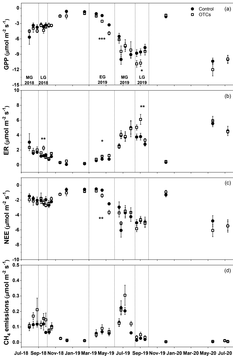
Figure IV-1 Measurements of gross primary production (GPP; a), ecosystem respiration (ER; b), net ecosystem exchange (NEE; c) and CH 4 emissions (d) in control and OTCs plots ( \pm SEM; n=6 ) from August 2018 to July 2020. Significant differences of repeated measure ANOVA in early (LG), middle (MG) and late growing season (LG) are expressed as * p < 0.05 , ** p < 0.01 , *** p < 0.001 .
