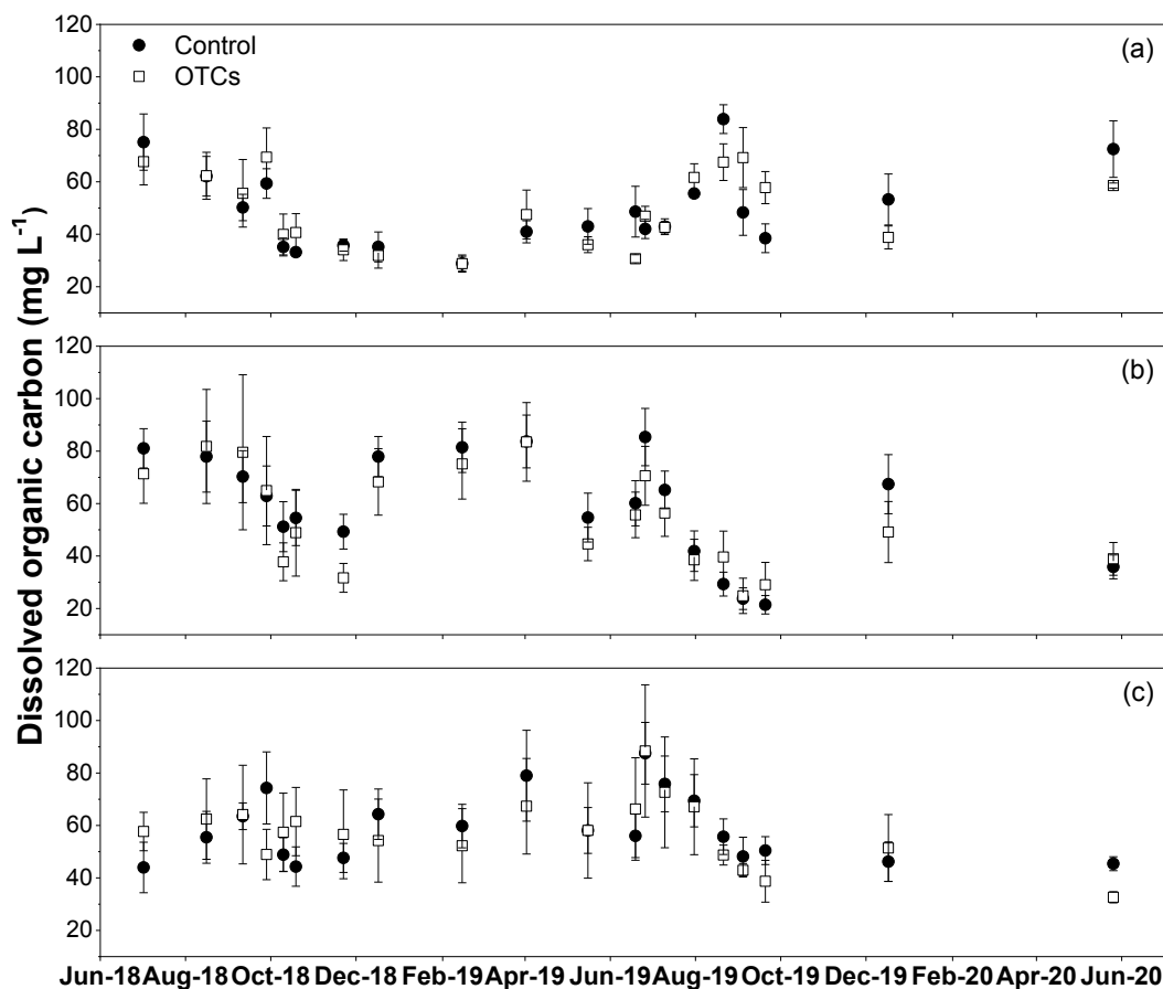
Figure V-2 Dissolved organic carbon (DOC) concentration ( \text{mg L}^{-1} ) at 5, 15 and 30 cm depth in mesocosms from July 2018 to June 2020 for control and OTCs plots. Error bar represents standard error mean (SEM).
