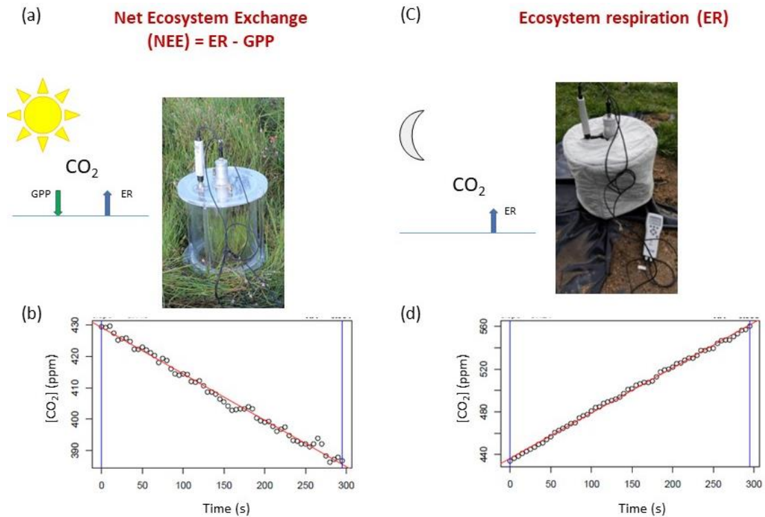
Figure II-3 Measurement of net ecosystem exchange (NEE) with transparent chamber (a) and the corresponding slope of decreasing \text{CO}_2 concentration against time which represents the absorption of \text{CO}_2 (ppm/s; b); Measurement of ecosystem respiration (ER) and the corresponding slope of increasing \text{CO}_2 concentration against time which represents the release of \text{CO}_2 (ppm/s; b).
