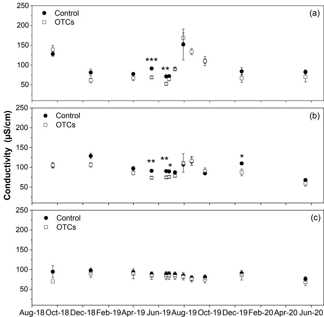
Figure III-7 Conductivity ( \mu\text{S}/\text{cm} ) of pore water from 5 (a), 15 (b) and 30 cm (c) of mesocosms under control and OTCs treatment. Error bar represents the standard error of the mean (SEM). Significant differences of one-way ANOVA are expressed as *p < 0.05 , **p < 0.01 , ***p < 0.001 .
