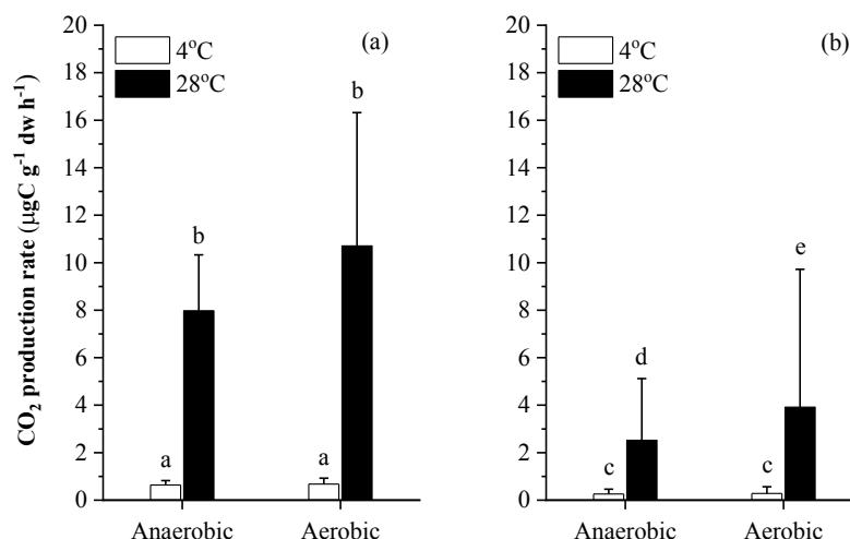
Figure VI-2 CO 2 production rate ( \mu\text{gC g}^{-1} \text{dw h}^{-1} ) of peat from (a) 5-10 cm layer and (b) 35-40 cm layer incubated at 4 and 28°C during 7 days incubation under anaerobic and aerobic conditions. Different letters represent significant differences by ANOVA in each panel and error bars represent the standard deviation (SD).
