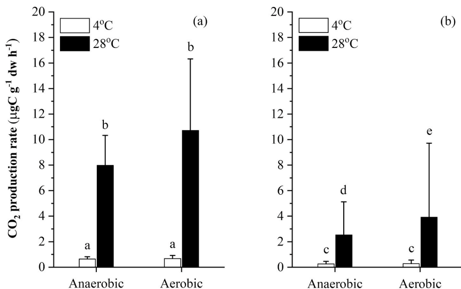
Fig. 2. CO 2 production rate ( \mu\text{gC g}^{-1} \text{dw h}^{-1} ) of peat from (a) 5–10 cm layer and (b) 35–40 cm layer incubated at 4 and 28 °C during 7 days incubation under anaerobic and aerobic conditions. Different letters represent significant differences by ANOVA in each panel and error bars represent the standard error.
