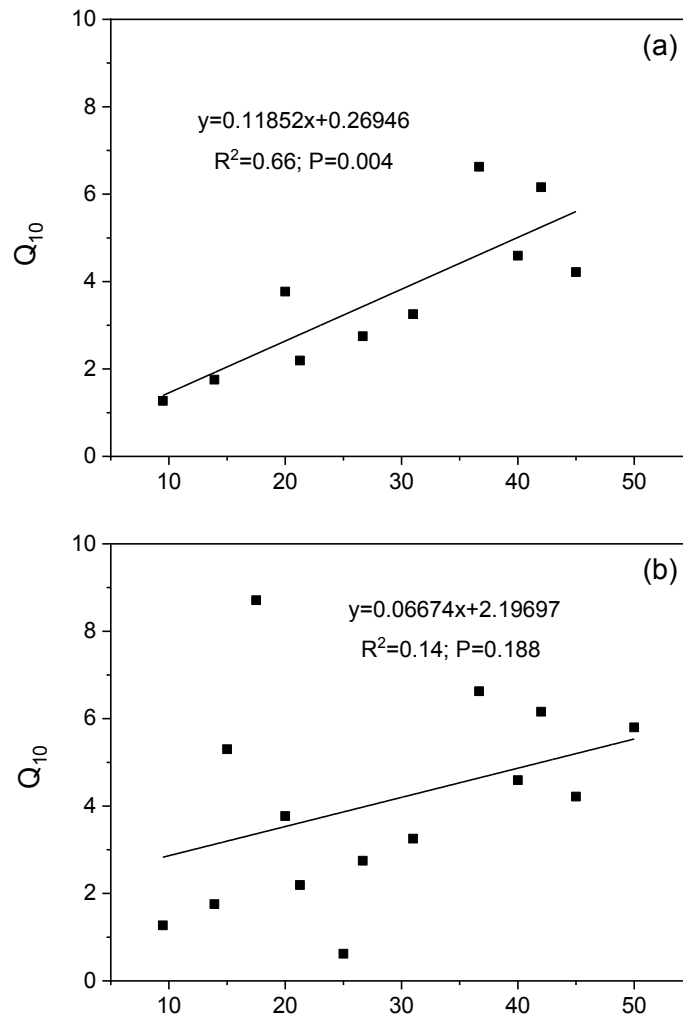
Supplementary Figure VI-2 Relationship between Q_{10} of CO_2 production rate and soil depth (cm) without (a) and with (b) outliers (frequency of occurrence < 2 %) based on data summarized in Supplementary Table VI-1.
