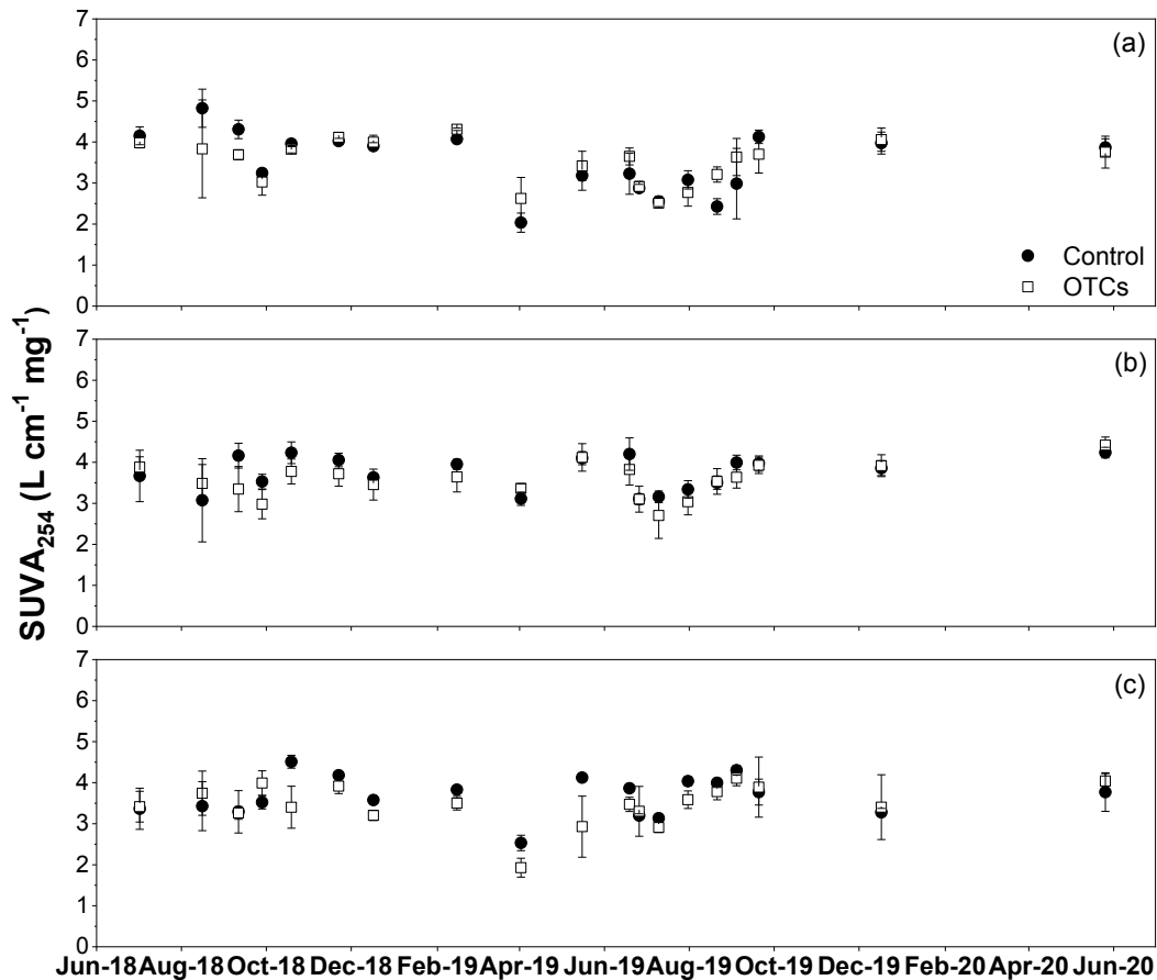
Figure V-4 Specific ultraviolet absorbance at the wavelength 254 nm SUVA 254 (L cm -1 mg -1 ) at 5, 15 and 30 cm depth in mesocosms from July 2018 to June 2020 in control and OTCs plots. Error bar represents standard error mean (SEM).
