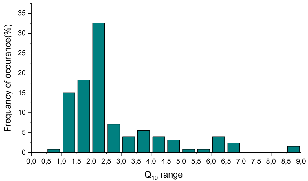
Supplementary Figure VI-1 Range of Q 10 summarized in Supplementary Table VI-1 and their frequency.
