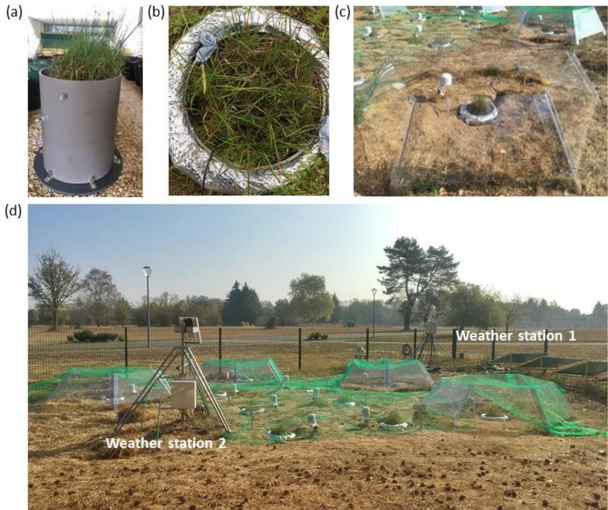
Figure II-2 Mesocosm of 40 cm in thickness and 30 cm in diameter collected from La Guette peatland (a); Mesocosms were buried in mineral soil and isolated by bubble wrap from surrounding environment; (b) Mesocosms subjected to warming treatment with Open-top chambers (OTCs); (c) The study site outside of laboratory ISTO for the mesocosms under two treatments (control and OTCs treatment) with two weather stations monitoring the environmental variables (d).
