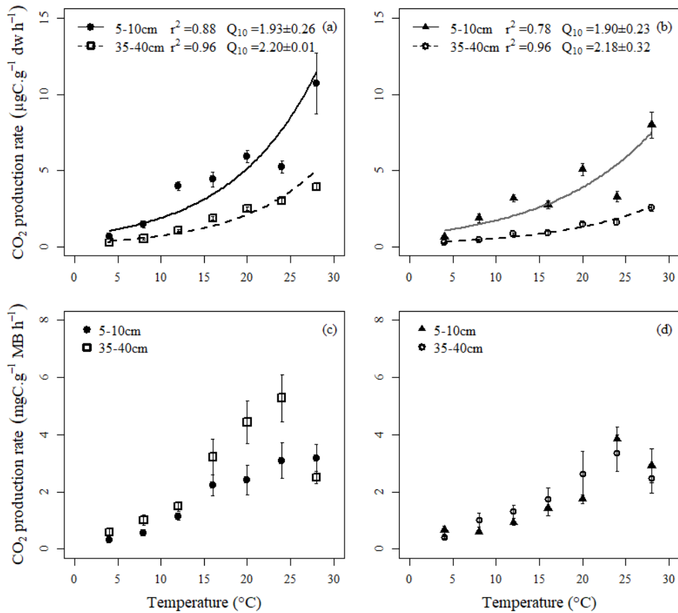
Figure VI-1 CO 2 production rate (µgC g -1 dw h -1 ) under (a) aerobic and (b) anaerobic conditions; and CO 2 production per gram microbial biomass (mgC g -1 MB h -1 ) under (c) aerobic and (d) anaerobic conditions as a function of temperature for peat from 5-10 cm and 35-40 cm layer. The lines in panels a and b correspond to the model fitted to the measurements. Error bars represent the standard deviation (SD).
