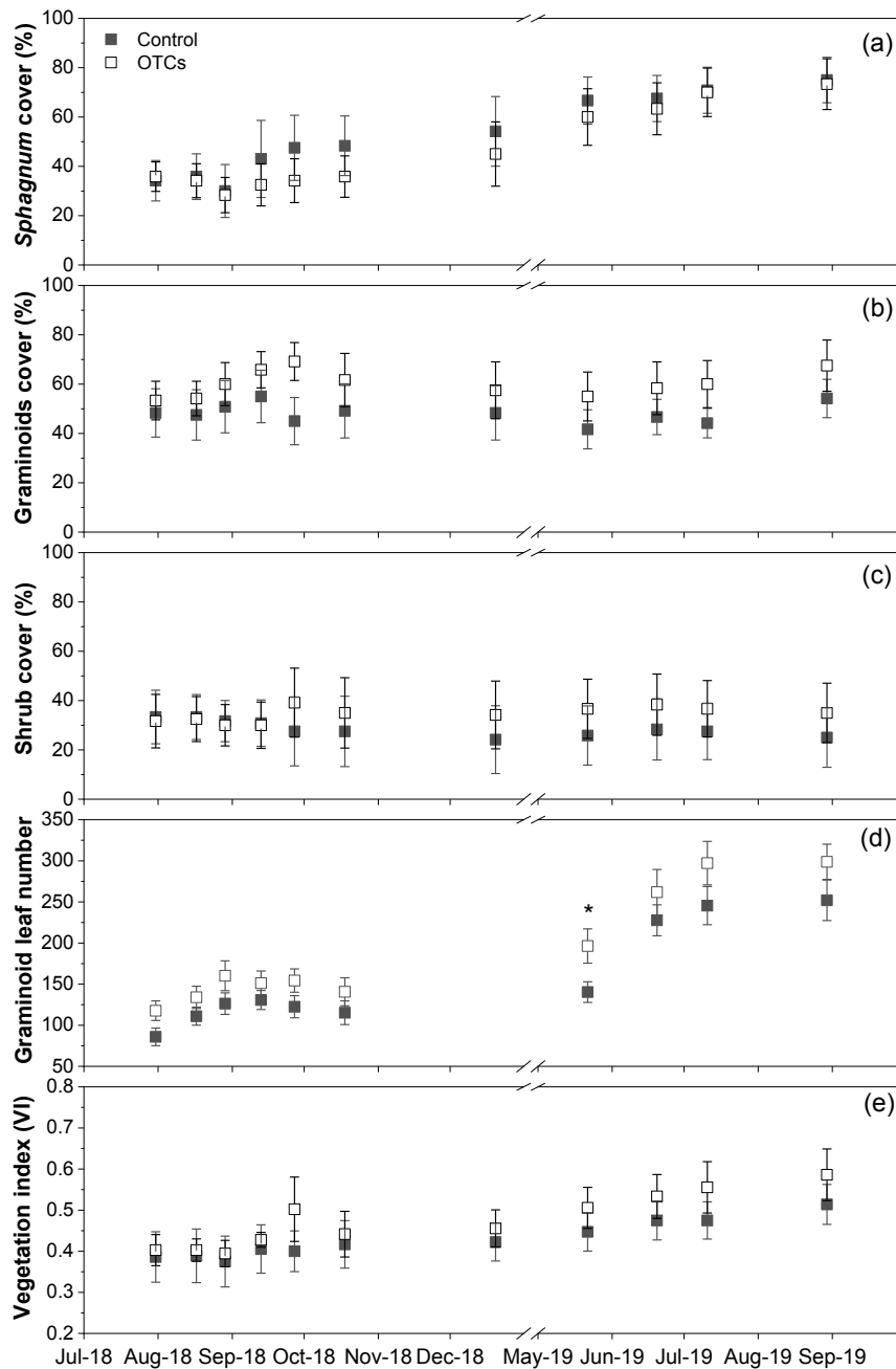
Figure III-5 Percentage cover (%) of bryophytes ( Sphagnum ; a), graminoids ( Molinia caerulea and Eriophorum augustifolium ; b) and ericaceous shrubs (c), leaf number of graminoids ( Erica tetralix and Calluna vulgaris ; d) and vegetation index (VI; e) from July 2018 to September 2019. Error bar represents the standard error of the mean (SEM). Significant differences of one-way ANOVA are expressed as * p < 0.05 , ** p < 0.01 , *** p < 0.001 .
