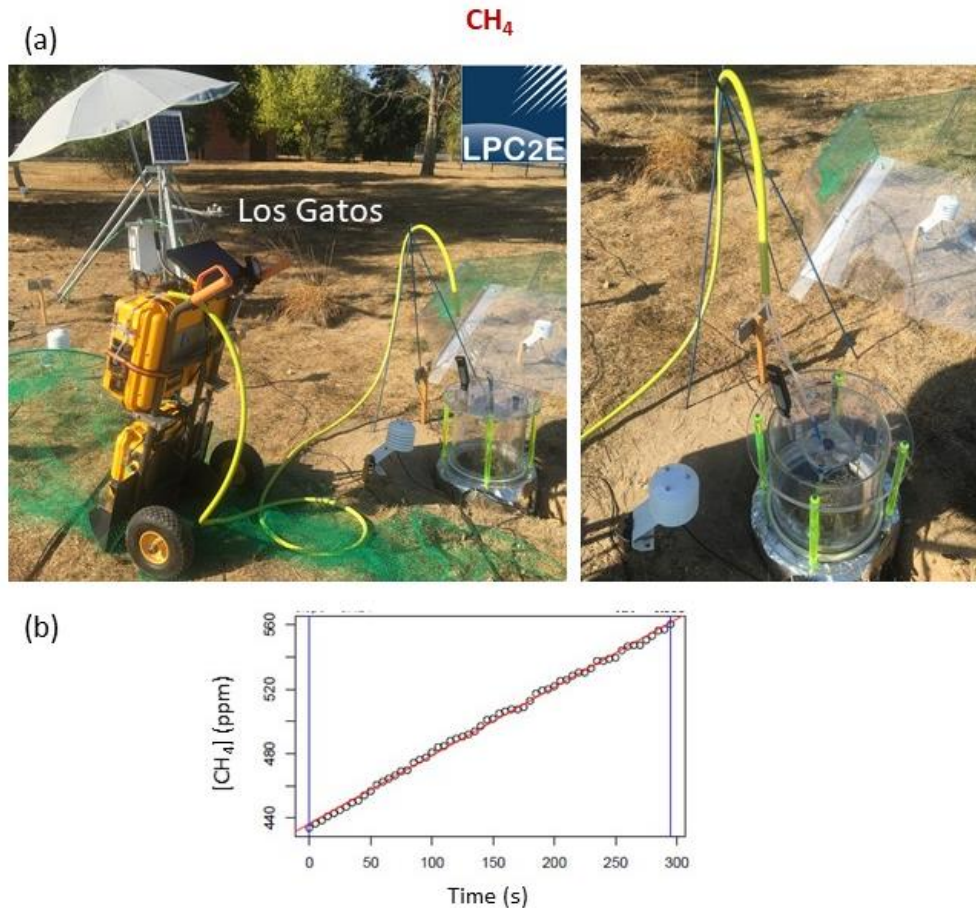
Figure II-5 Measurement of CH 4 was carried out by Los Gatos with a transparent sealed chamber and the slope of increasing CH 4 concentration against time was corresponding to the release of CH 4 (ppm/s).
