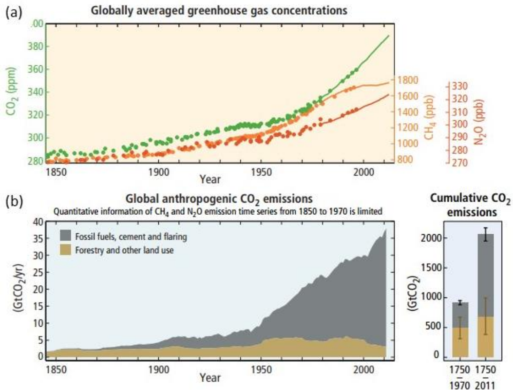
Figure I-4 Observed changes in atmospheric greenhouse gas concentrations (a) and global anthropogenic CO 2 emissions from different sources (b; IPCC, 2014).
