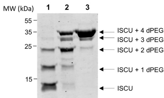
Figure S6: oxidation state of the cysteine residues in the H103A mutant.
