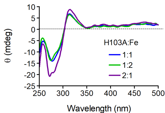
Figure S7: CD spectra of the H103A mutant at different protein to iron ratios.
