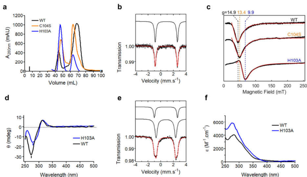
Figure 5: Characterization of the C104S and H103A mutants of Mm ISCU
