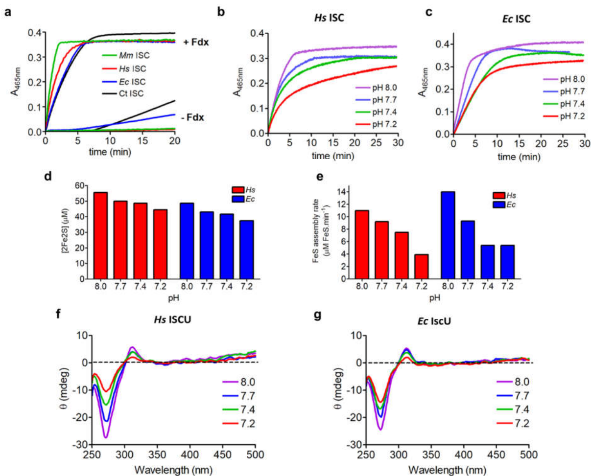
Figure 2: Effect of pH on Fe-S cluster assembly by selected ISC machineries
