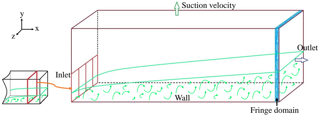
Fig. 3.2. Configuration of the simulation box.
