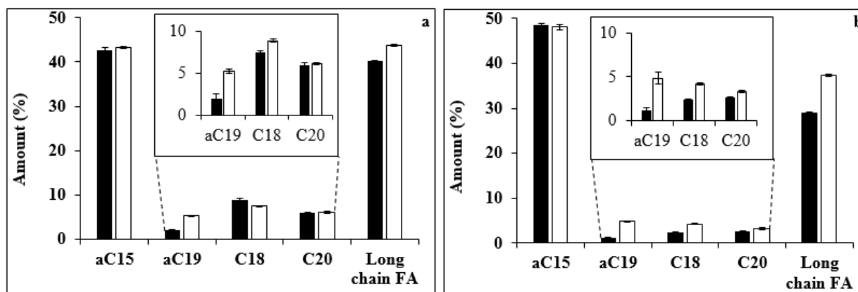
Figure 5 Fatty acid (FA) composition of Staphylococcus aureus biofilm-detached (a) and planktonic cells (b) cultivated at 20°C (black column) and 37°C (white column) for 24 h. a for anteiso
