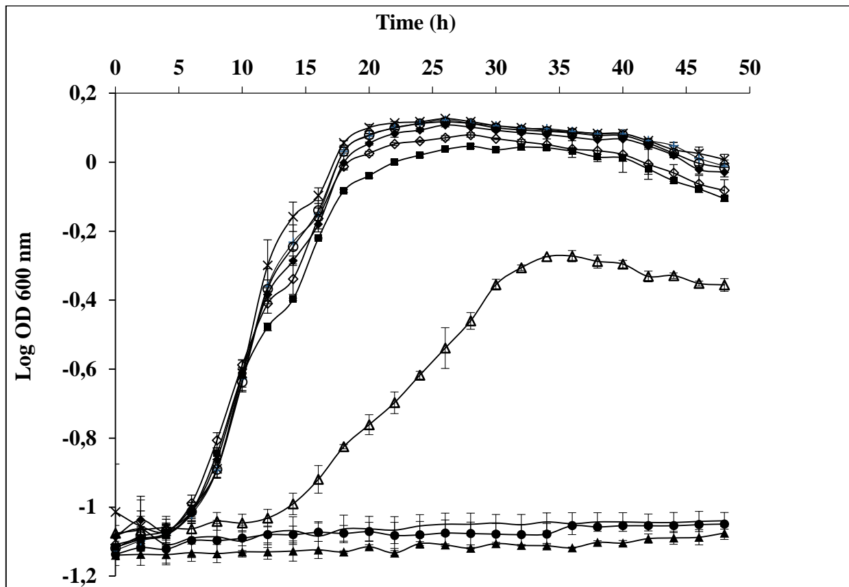
Figure 1 Growth curves of Pseudomonas aeruginosa in presence of BAC concentrations of 25 ( \blacktriangle ), 12.5 ( - ), 6.25 ( \Delta ), 3.12 ( \blacksquare ), 1.56 ( \diamond ), 0.8 ( \blacklozenge ), 0.4 ( \circ ), 0.2 ( + ) and 0 \text{ mg.l}^{-1} ( \times ). The concentration at which there was linear growth inhibition was considered the MIC. The bacterial growth in Mueller Hinton Broth without bacteria and benzalkonium chloride was measured to ensure the sterility of the growth medium (sterile control) ( \bullet ). The \pm SEM for three replicates are illustrated.
