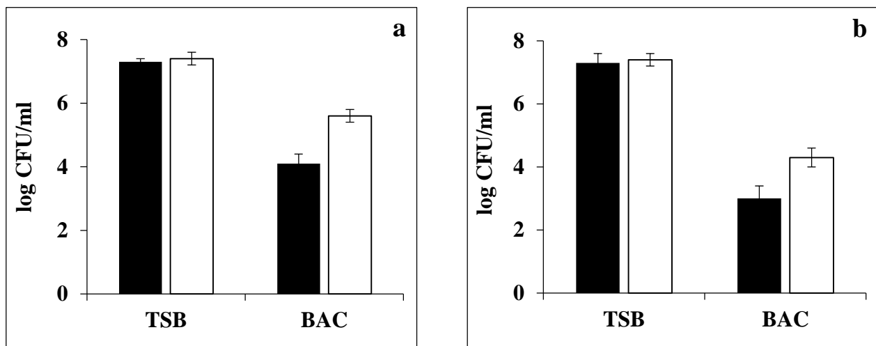
Figure 2 Effect of benzalkonium chloride (BAC) treatment on biofilm-detached (a) and planktonic (b) Staphylococcus aureus grown during 24 h at 20°C (black column) and 37°C (white column). The bacterial density is presented in log CFU/ml. The \pm SEM for three replicates are illustrated after treatments with TSB (control) and BAC.
