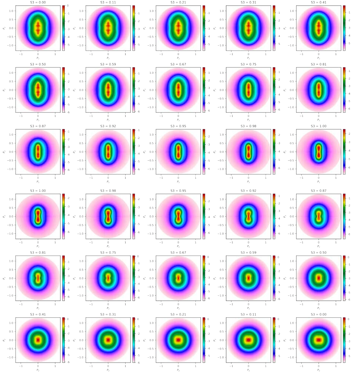
Figure 4.12 – 2-D projections of the 3-D photoelectron angular distribution acquired by the VMI, of Fenchone , in momentum co-ordinates for various ellipticities. Note that for a given orientation of the \lambda/4 waveplate a horizontal and vertical projection of the 3-D PAD is measured in the VMI.
