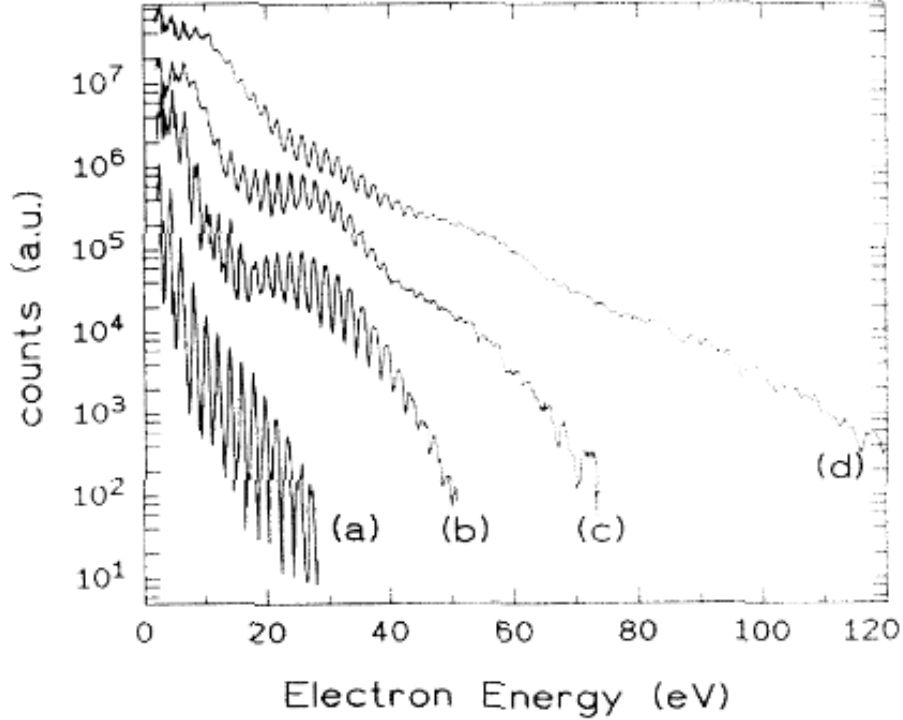
Figure 2.23 – Typical photoelectron spectrum of above threshold ionization. Extracted from [Paulus 00]
