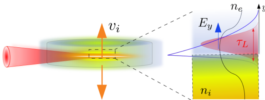
Fig. 4: Sketch of CE in a near-critical plasma slab while the laser pulse is still on.
