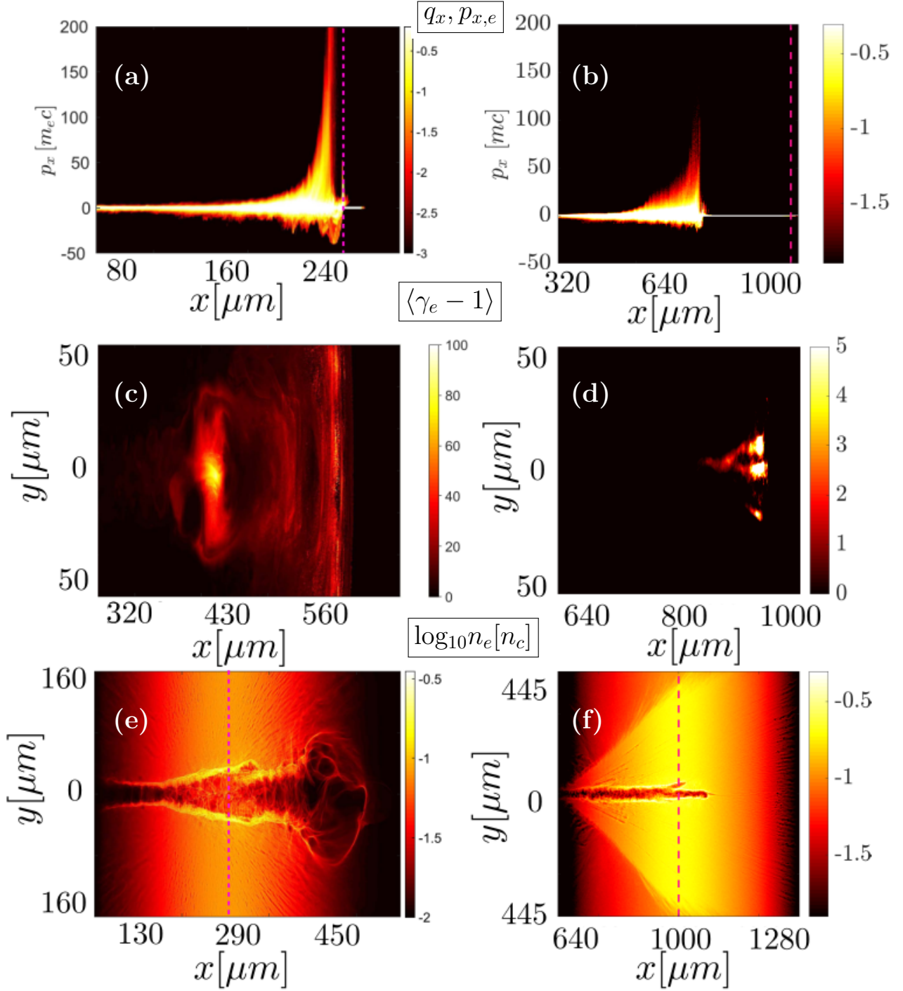
Fig. 5.28: (a-f) Comparison of the two simulations' results: the left column corresponds to results from Ref. [31] and the right column to results from this work. The locations of the density profiles' peaks are marked with pink vertical dashed lines (in the images where it is visible given the x -axis limits, x_{n_{max}} = 1500 c/\omega_0 in Ref. [31] and x_{n_{max}} = 6000 c/\omega_0 in this work). (a-b) Electron (x, p_x) phase spaces captured during the turbulent energization phase. (c-d) Mean electron kinetic energy \langle \gamma_e - 1 \rangle charts. (e-f) Electron density n_e charts taken at the last time step of each simulation.
