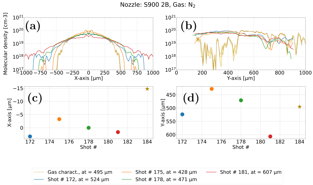
Fig. 2.31: (a-d) As labeled in Fig. 2.30 corresponding to the S900 2B nozzle & pure nitrogen.
