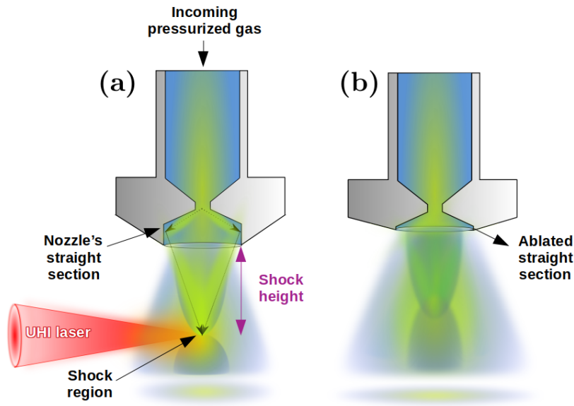
Fig. 2.25: Artist vision of the laser-induced nozzle damage (LIND), note that the size of the gas container has been artificially increased for artistic purposes. (a) Virgin nozzle and (b) same nozzle after the UHI laser interaction has ablated its last straight section.
