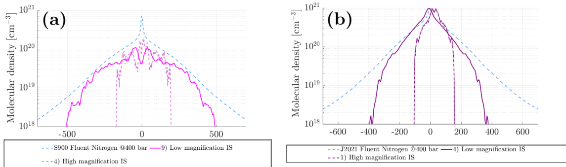
Fig. 2.24: Comparison of the transverse density profile obtained for the (a) S900 and (b) J2021 nozzles with the same gas and PCs (seen in the plot legend) as obtained with both the high magnification (HM) and low magnification (LM) optical lines. See setup of Fig. 2.17.
