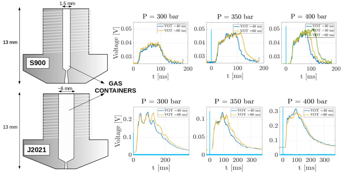
Fig. 2.19: (Top) From left to right: sketch of the S900 nozzle showing its gas container and time-dependent strioscopy signals corresponding to a mixture of 90% nitrogen and 10% helium and backing pressures of 300, 350 and 400 bar. (bottom) Same as top corresponding to the J2021 nozzle.
