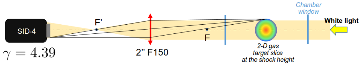
Fig. 2.11: Optical setup used to characterize the phase shifts of the probe beam through the dense gas during the rapid valve and microvalve characterization campaign.
