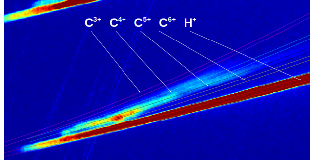
Fig. 4.24: Saturated zoom of Fig. 4.23a (IP of the 0^\circ three-pinhole TP corresponding to the solid target shots #15-19), where we can appreciate the C^{6+} , C^{5+} , C^{4+} , C^{3+} and H^+ parabolic traces. The zoom corresponds to the left trace of Fig. 4.23a i.e., to the 1.71^\circ spectrum trace.
