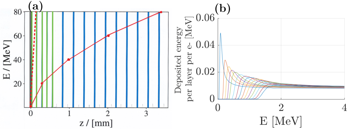
Fig. 4.30: (a) Output of a SRIM [164] simulation using the PySTarT runtime environment [110] of the stopping of \alpha particles (continuous line) and nitrogen ions (dashed line) in an RCF stack composed of a 10 \mu m layer of aluminum (grey layer) followed by five layers of unlaminated EBT-3 RCF film (green layers) and 10 layers of EBT-3 film (blue layers). (b) Result of a Geant-4 simulation of electrons traversing the same RCF stack. Each curve corresponds to one stack layer, from the 1st to the 15th (from left to right). The abscissa is the energy of the incoming electron and the ordinate the deposit energy per layer and per electron.
