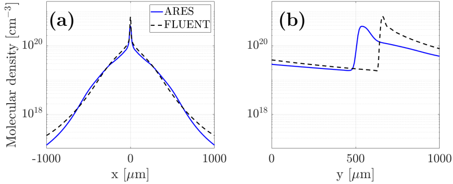
Fig. 2.6: (a) Transverse and (b) longitudinal density profiles obtained after simulating the S900 nozzle using the Fluent [118] and ARES [119] codes inputting a pressure reservoir of 400 bar of nitrogen.
