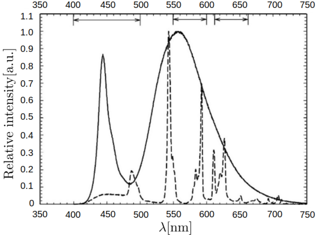
Fig. A.28: Emission spectrum of the EPSON EXPRESSION11000XL flat-bed scanner in dashed line. The detection bands of the RGB color channels are indicated with arrows. Extracted from Ref. [223].
