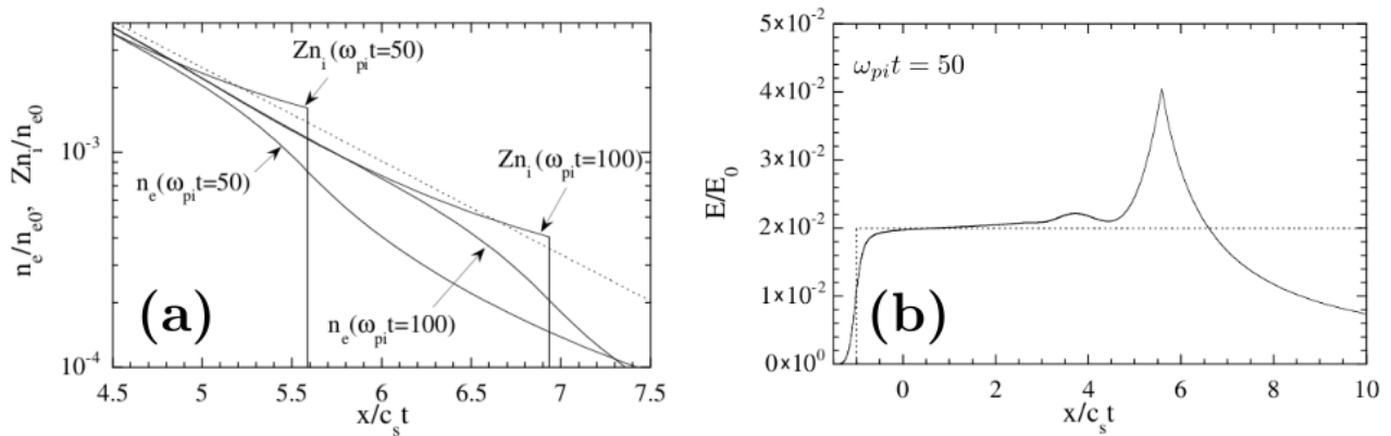
Fig. 3: (a) Structure of the ion front at times \omega_{pi}t = 50 and \omega_{pi}t = 100 according to Mora [41]. The dotted line is the usual self-similar solution obtained using Eqs. 0.2. (b) Electric field at \omega_{pi}t = 50 , the ion front is located at x/C_s t \approx 5.59 . Figures extracted from Ref. [41].
