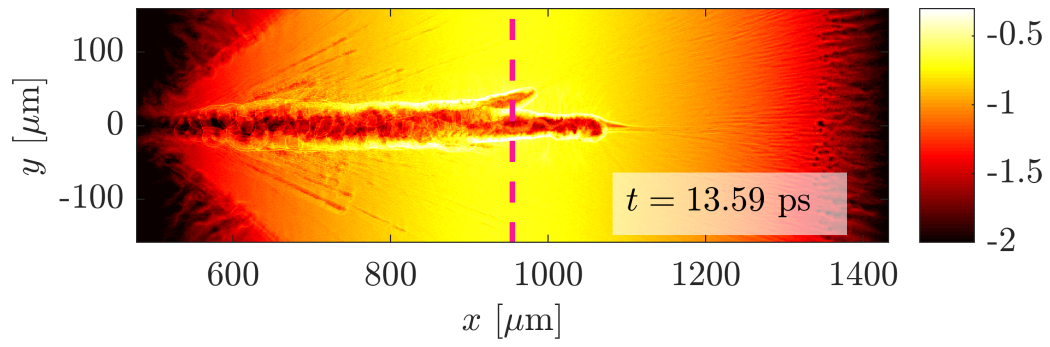
Fig. 5.29: Electron density n_e chart taken at t = 13.59 ps corresponding to the simulation presented in this chapter.
