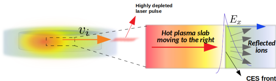
Fig. 6: Sketch of CSA in a near-critical plasma slab.
