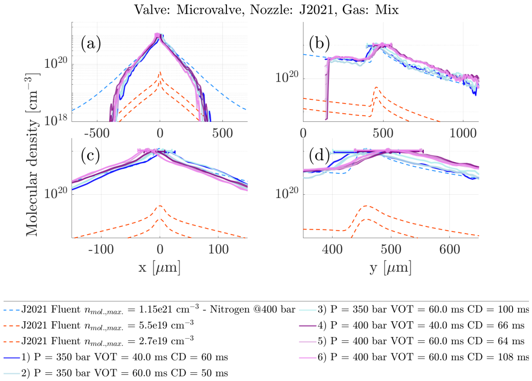
Fig. 2.22: (a-d) As labeled in Fig. 2.14 corresponding to the microvalve coupled with the J2021 nozzle and a 9/1 He/N 2 gas mixture.
