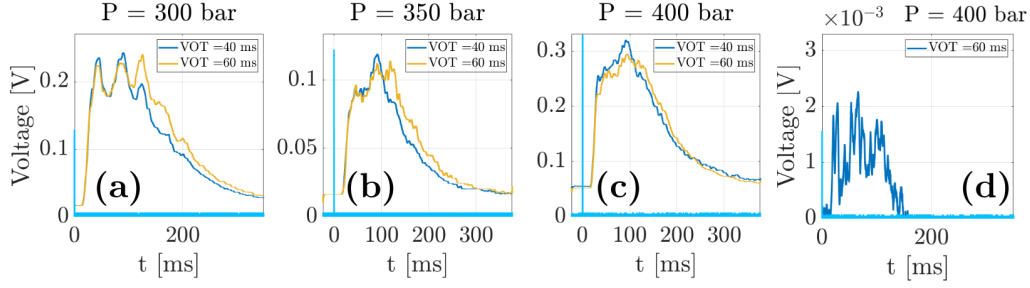
Fig. 2.18: Time-dependent strioscopy voltage signal at the shock height, acquired using a digital oscilloscope, corresponding to the J2021 nozzle and gas mixture (a-c) or helium (d). The voltage level is proportional to the gas density. The different measurements correspond to different P values from 300 bar to 400 bar and VOTs, either 40 ms or 60 ms. The light blue peak corresponds to the oscilloscope's trigger signal.
