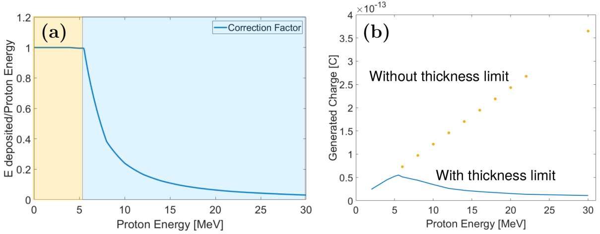
Fig. A.15: (a) Energy dependent charge correction factor CF , extracted from Ref. [192], and (b) its effect on the calculation of the accumulated charge in the detector's electrodes. Image courtesy of M. Salvadori.
