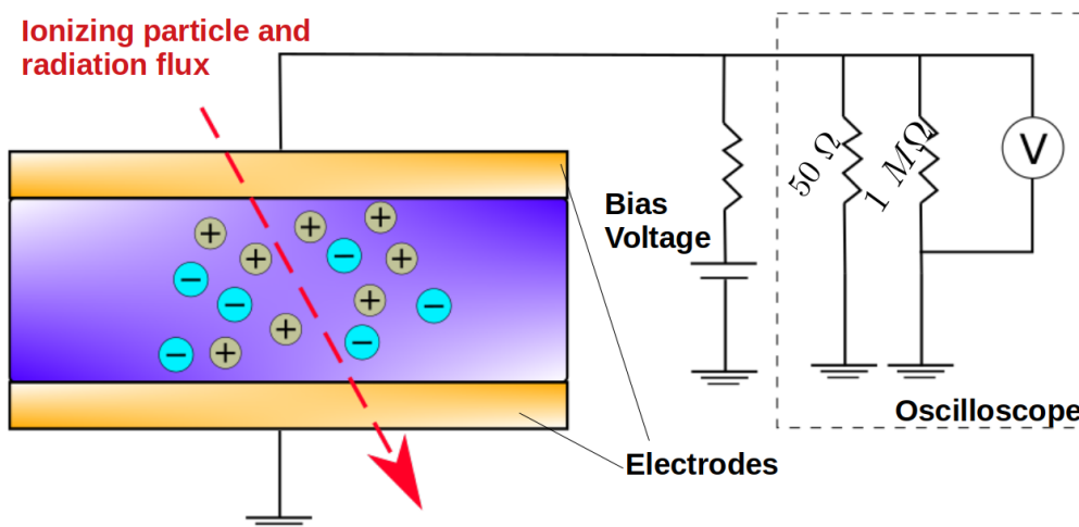
Fig. A.13: Schematic representation of a ToF detector and acquisition circuit.
