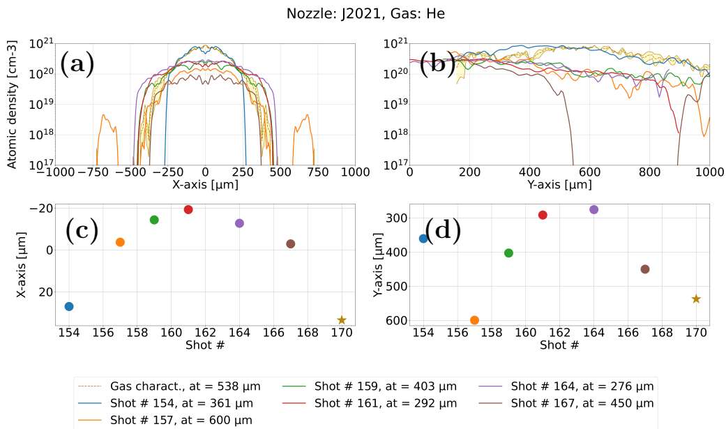
Fig. 2.33: (a-d) As labeled in Fig. 2.30 corresponding to the J2021 nozzle & pure He.
