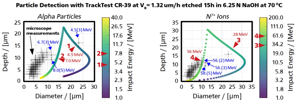
Fig. 4.8: Retrieved depth-diameter measured points in black and calibration curves in false colors linked to the particle energy for \alpha particles (left figure) and N^{7+} ions (right figure).
