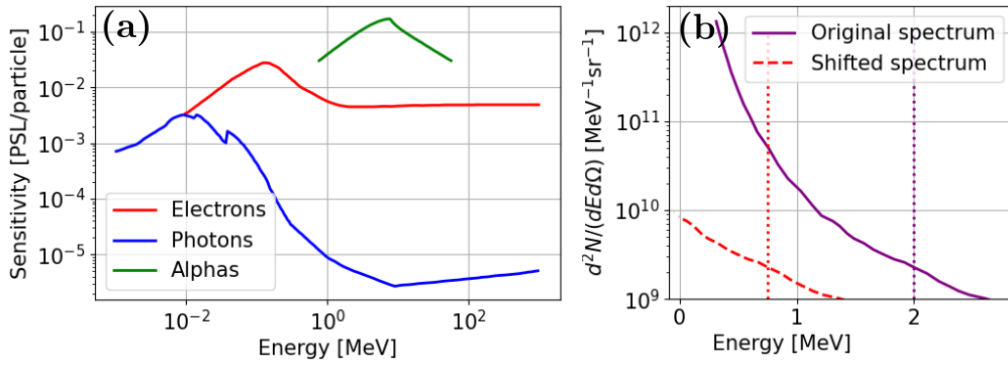
Fig. 4.29: (a) Sensitivity of IPs of the type TR to electrons [161], photons [162] and \alpha particles [163]. (b) \alpha particles spectrum obtained using the ToF A detector, corresponding to shot #140 in pure He.
