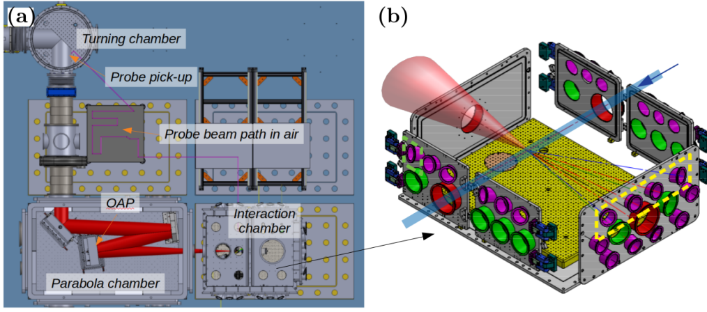
Fig. 4.10: (a) VEGA-3 target area (TA) layout. The main beam enters the interaction chamber (IC) as it is focused using an f/12 off-axis parabola (OAP). (b) 3-D CAD render of the VEGA-3 IC. The focused main VEGA-3 pulse is drawn in red and the probe beam in blue. The IC has 1.1 \times 1.4 \times 0.8 \text{ m}^3 (width \times large \times height) dimensions. Images printed with permission of the CLPU.
