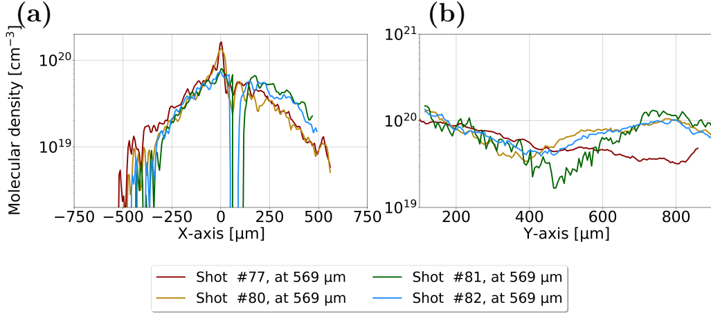
Fig. 2.27: (a) Transverse and (b) longitudinal lineouts of shots #77, #80, #81 and #82 of the VEGA-2 campaign.
