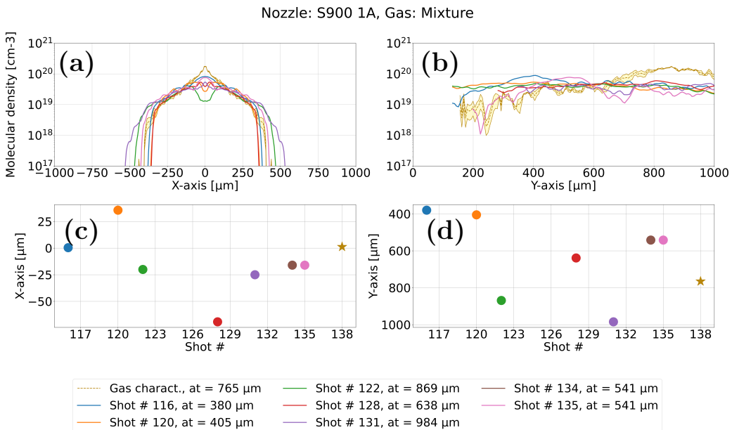
Fig. 2.32: (a-d) As labeled in Fig. 2.30 corresponding to the S900 1A nozzle & gas mixture.
