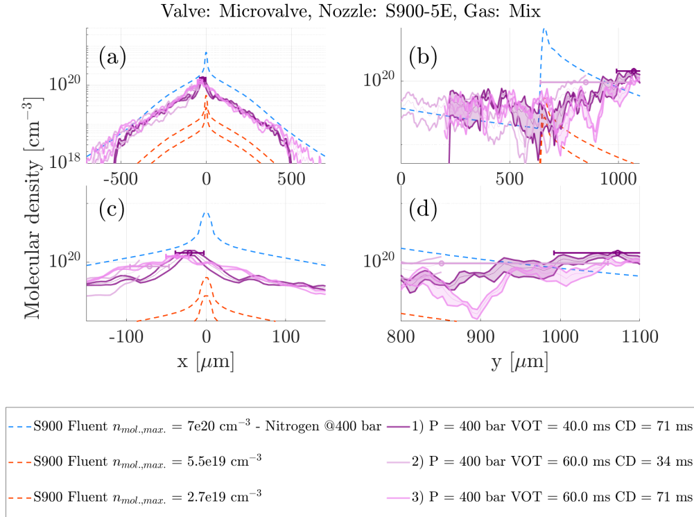
Fig. 2.20: (a-d) As labeled in Fig. 2.14 corresponding to the microvalve coupled with the S900-5E nozzle and a 9/1 He/N 2 gas mixture.
