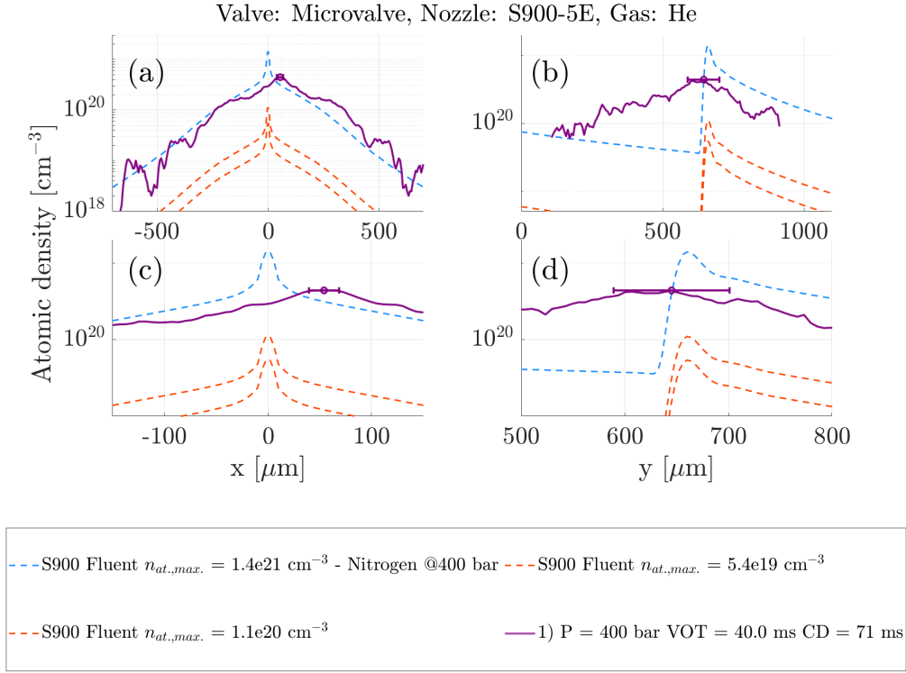
Fig. 2.21: (a-d) As labeled in Fig. 2.14 corresponding to the S900-5E nozzle and He.
