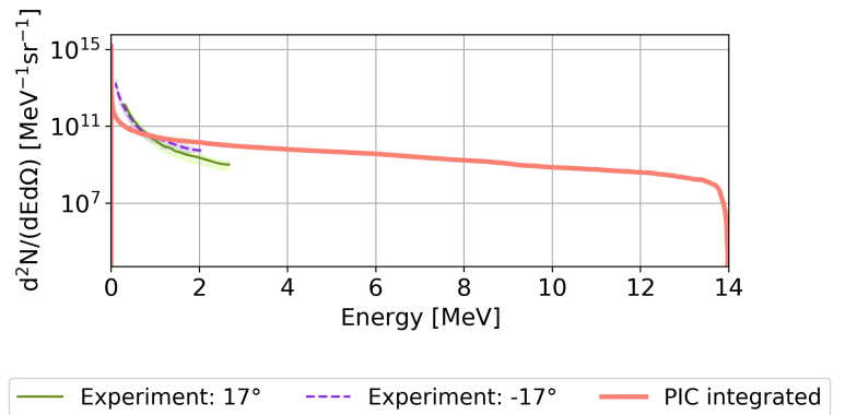
Fig. 5.22: Comparison of the experimental and numerical ion spectra at different azimuthal angles. The experimental ion spectra were acquired at \pm 17^\circ from the laser axis (see green and violet spectra). Numerical ion spectra are obtained by integrating the x, p_x ion phase space of Fig. 5.19. Note that the numerical spectrum has been multiplied by a coefficient in order to plot it side-by-side with the absolute experimental energy spectra.
