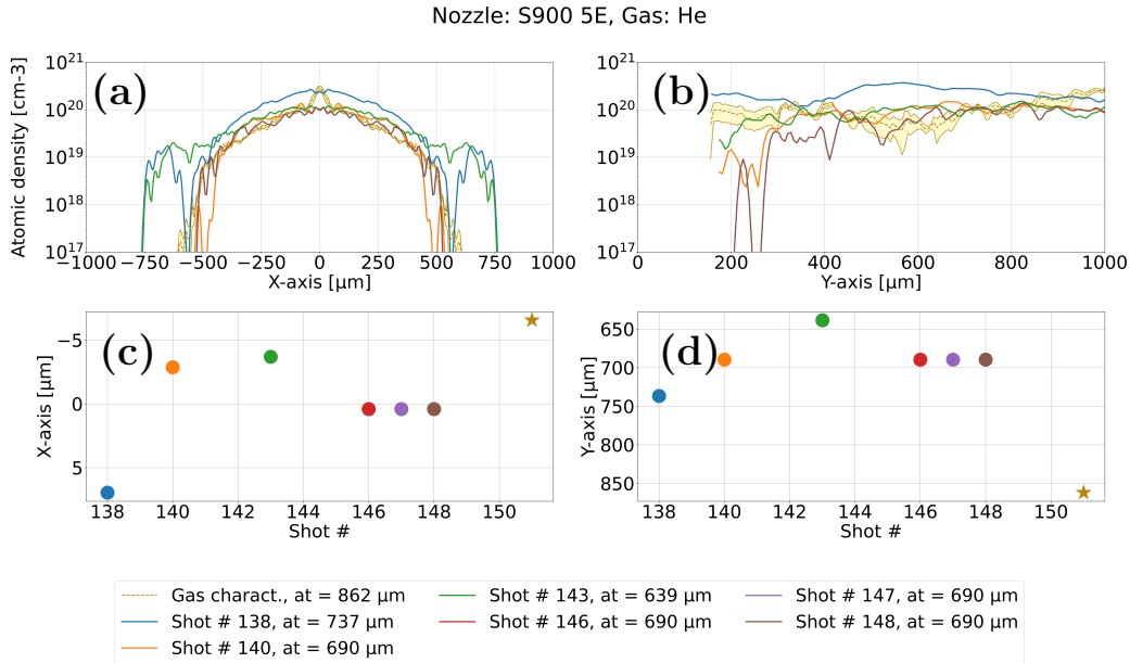
Fig. 2.30: On-shot (a) transverse and (b) longitudinal density lineouts obtained using the S900 5E nozzle & pure He during the VEGA-3 experiment. The dark yellow transverse and longitudinal lineouts in (a) and (b) correspond to measurements obtained during the microvalve -only characterization campaign. Shot-to-shot (c) horizontal and (d) vertical shock coordinates, the microvalve -only characterization horizontal shock coordinate is plotted as dark yellow stars.
