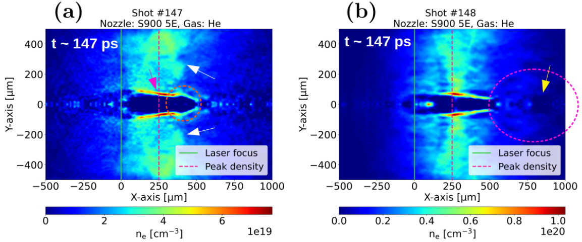
Fig. 4.40: Density charts obtained by deconvolving the raw interferograms at t \approx 147 \text{ ps} of (a) shot #147 and (b) shot #148 corresponding to the S900 5E nozzle & He. The laser propagates from left to right.
