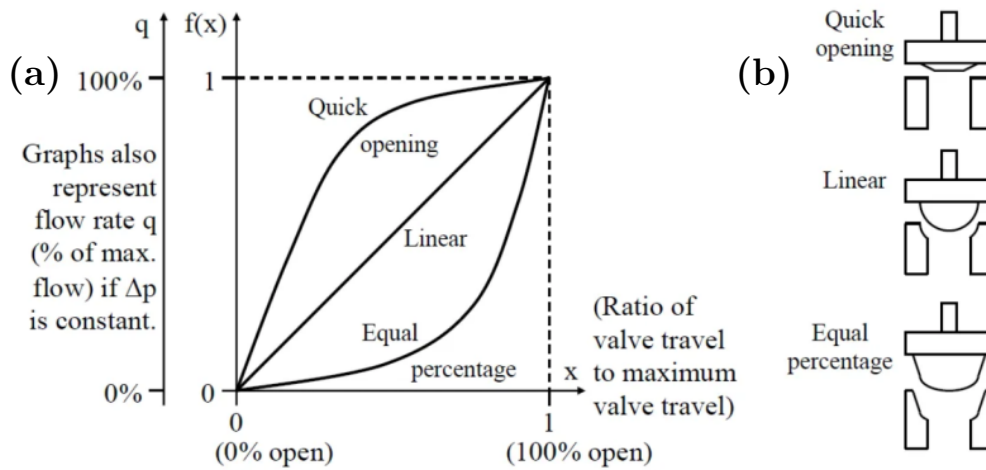
Fig. 2.10: (a) Quick-opening, linear and equal-percentage flow vs. stem position valve opening curves and (b) their respective valve seat and closure member designs. Extracted from Ref. [125].
