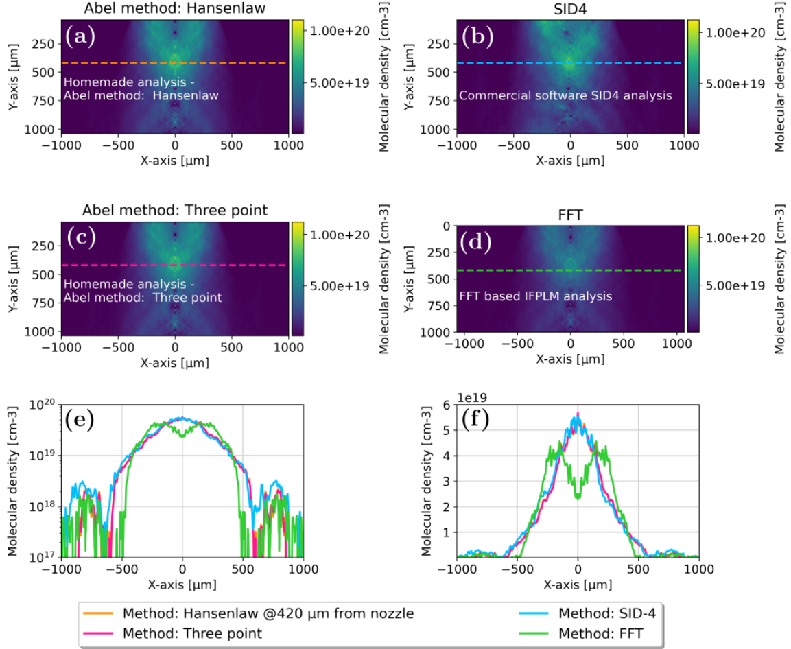
Fig. 2.3: (a) Density map obtained using the homemade routine and the Hansenlaw [112] method, (b) the SID-4 density module, (c) the homemade Python routine and the three-point [112] method and (d) the FFT method to solve the Abel equation. (e) Transverse lineouts at the shock height (plotted in logarithmic scale) extracted from the density charts plotted in (a-d) and (f) same curves as (e) plotted in linear scale.
