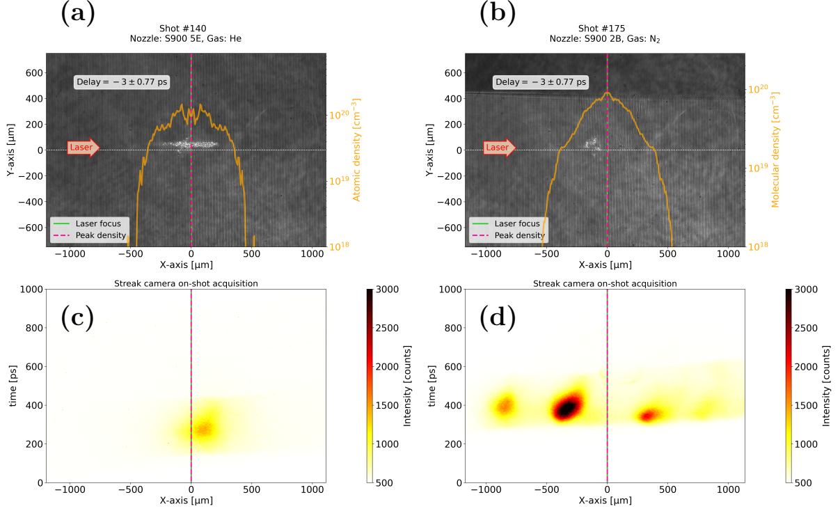
Fig. 4.42: (a) On-shot raw interferogram for the S900 5E nozzle & He and for the (b) S900 2B nozzle & N 2 . (c) Corresponding on-shot streak camera acquisition for the S900 5E nozzle & He and for the (d) S900 2B nozzle & N 2 .
