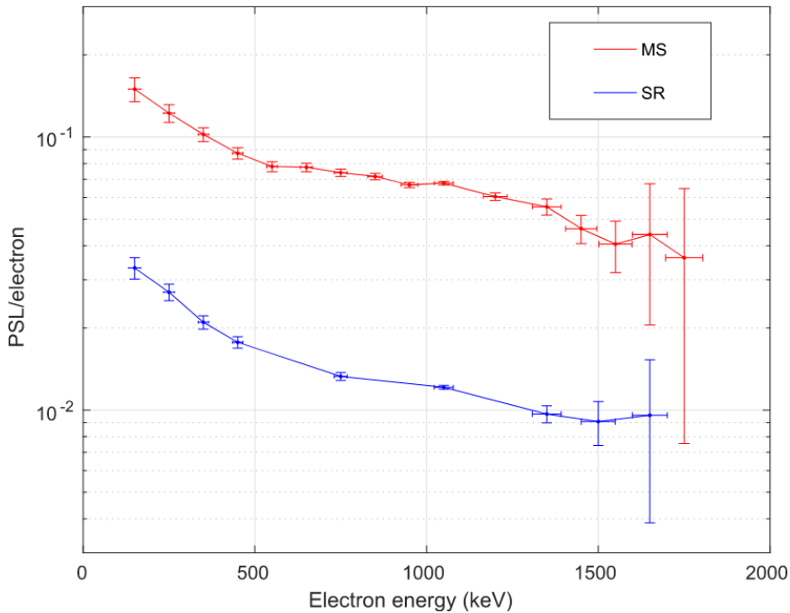
Fig. A.21: Sensitivity curve for IPs of the type MS and SR to electrons. Extracted from Ref. [200].
