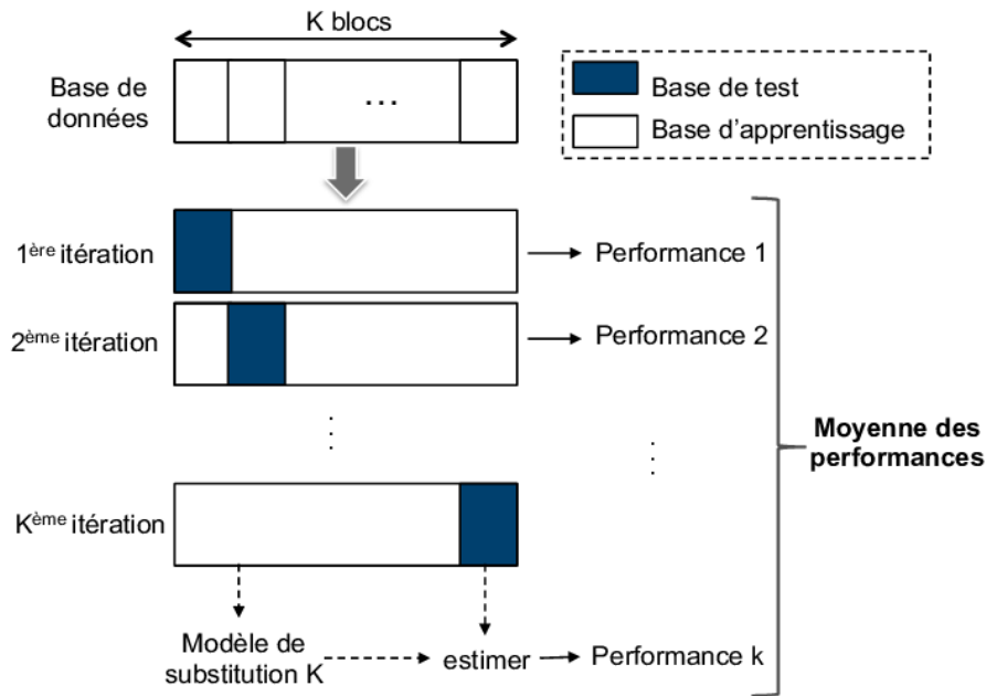
Figure 2.5 Principe de la validation croisée [Laqrichi, 2015]
