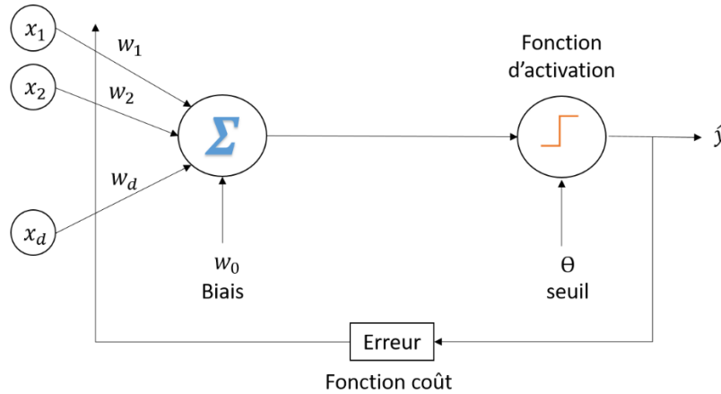
Figure 2.6 Illustration de l'algorithme perceptron
