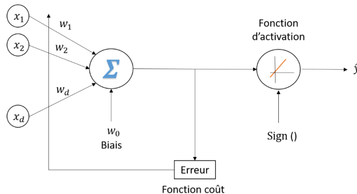
Figure 2.7 Illustration de l'algorithme adaline
