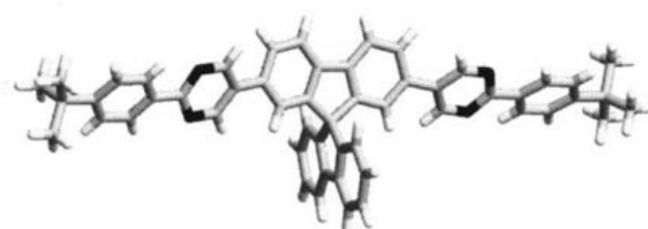
Figure 26 : Structure RX du spirocycle TBPSF
