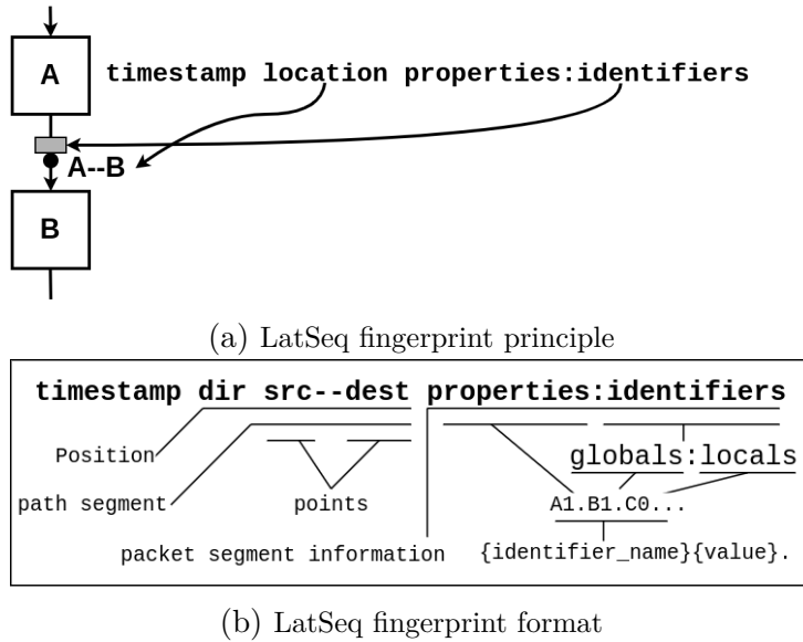
Figure 3.2 – LatSeq fingerprint.
