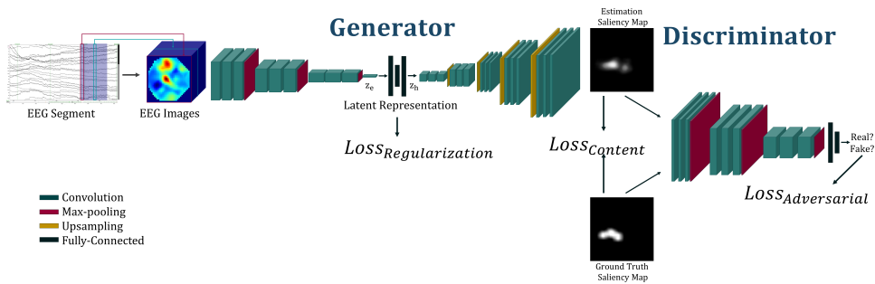
Figure 5.4. VAE architecture overview. At the left the encoding of the EEGs, to its mapping with the embedding of the saliency maps with the decoder. And The discriminator fulling the generator (composed by the encoder and decoder) at the right.
