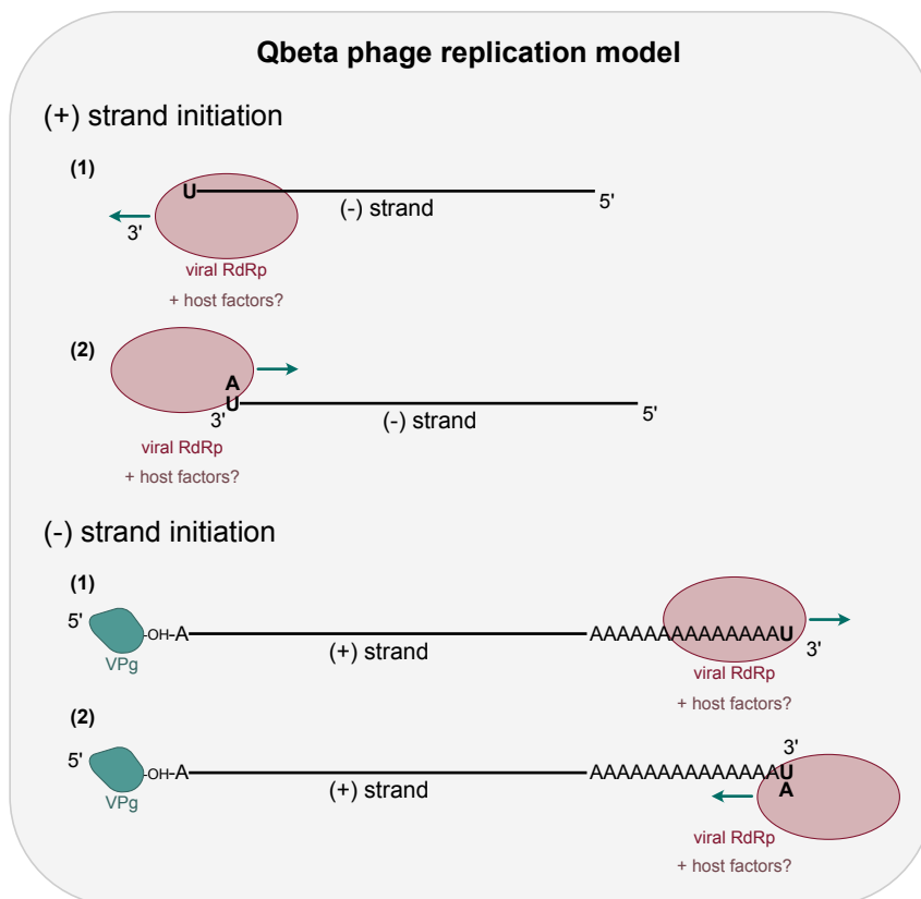
Figure 37: Models for GFLV RNA replication based on our data and published data on poliovirus and Qbeta phage replication. (A) Application of the poliovirus replication model to GFLV RNA. The VPg (green) is adenylated by the viral RdRp (red) and used to initiate the synthesis of (+) or (-) strand. Host factors could potentially be involved. In this model, both strands start with an A and end with an U. (B) Application of the Qbeta phage replication model to GFLV RNA. (1) After the completion of the template strand synthesis, (2) the viral polymerase adds a 3' terminal U to the strand and starts to replicate it. Host factors could potentially be involved. In this model, both strands start with an A and end with an U.
