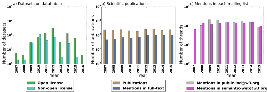
Figure 6.1: Data collection overview
