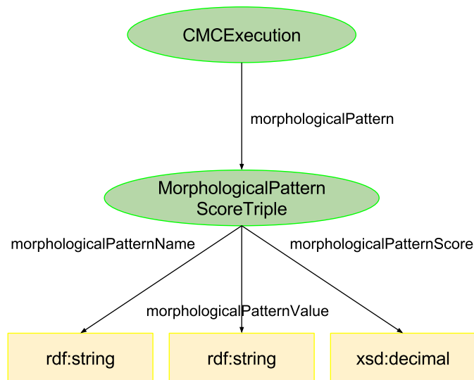
Figure 7.3: CMC metadata ontology
