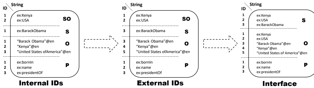
Figure 9.2: HDT Dictionary
