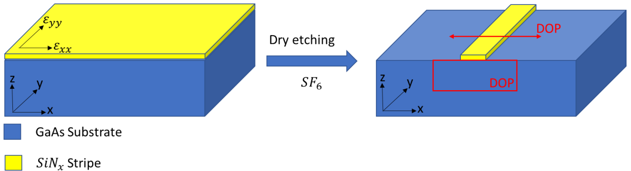
Figure 47: \text{SiN}_x stripe patterned by photolithography and etched by reactive ion etching using an \text{SF}_6 plasma on a GaAs (100) substrate. Scan-line for the DOP measurement from the surface and square for the cross-section measurement area.
