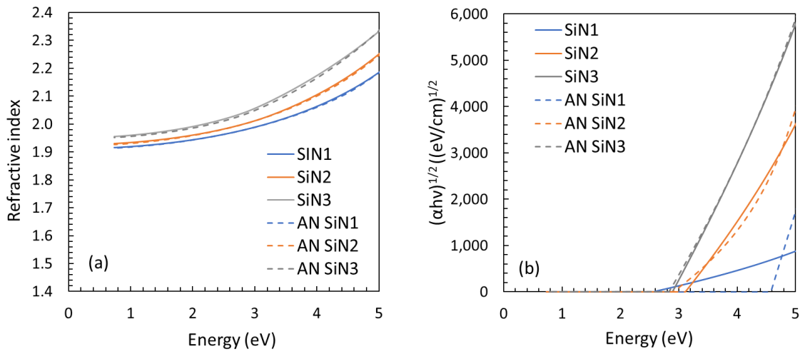
Figure 13: Refractive index (a) and Tauc plots (b) derived from the VASE measurements of \text{SiN}_x films deposited at three different pressures before and after annealing. “AN” indicates samples after annealing at 400\text{ }^\circ\text{C} .
