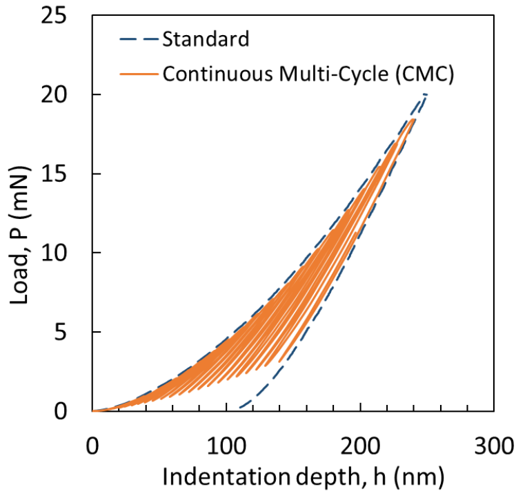
Figure 26: Single nanoindentation measurements with two different modes: standard and continuous multi-cycle mode.
