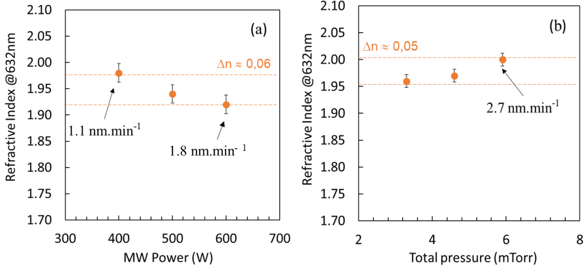
Figure 12: Refractive index at 632 nm of 500 nm \text{SiN}_x films deposited within the ECR reactor at three different deposition powers (a) and pressures (b). The samples (a) correspond to Set 1 from Table 2 and samples (b) correspond to Set 2 from Table 3.
