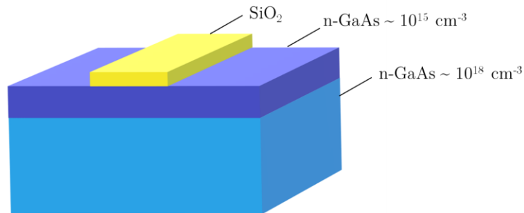
Figure 1: Photoelastic waveguides using a compressive \text{SiO}_2 stressor stripe deposited onto a surface planar waveguide in a GaAs-based structure [15].
