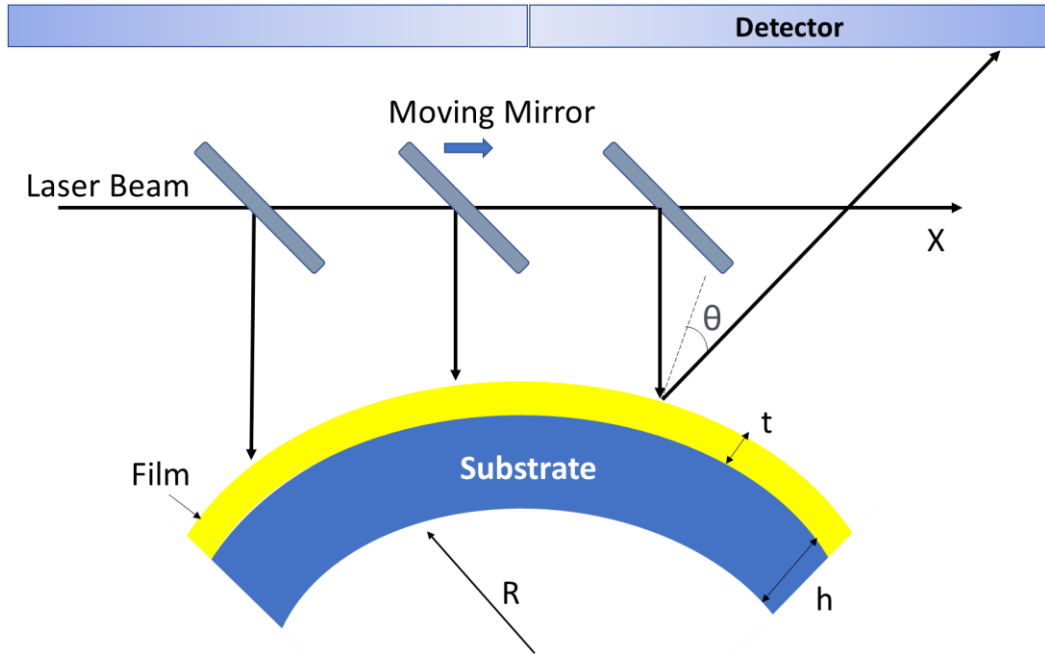
Figure 22: Principle of measuring the radius of curvature by reflectometry.
