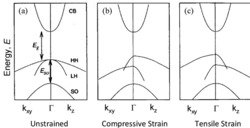
Figure 5: In direct bandgap bulk unstrained semiconductors (a), the HH and LH bands degenerate at the valence band maximum at the Brillouin zone center \Gamma . Compressive strain splits the degeneracy so that the highest band is light in the x-y plane of the layer but
