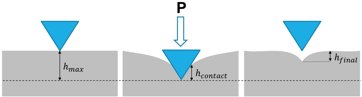
Figure 23: Indentation of a surface.
