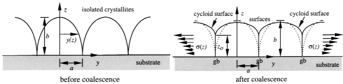
Figure 7: Crystallite coalescence process, showing the elastic displacements and stresses associated with forming a continuous film [56].
