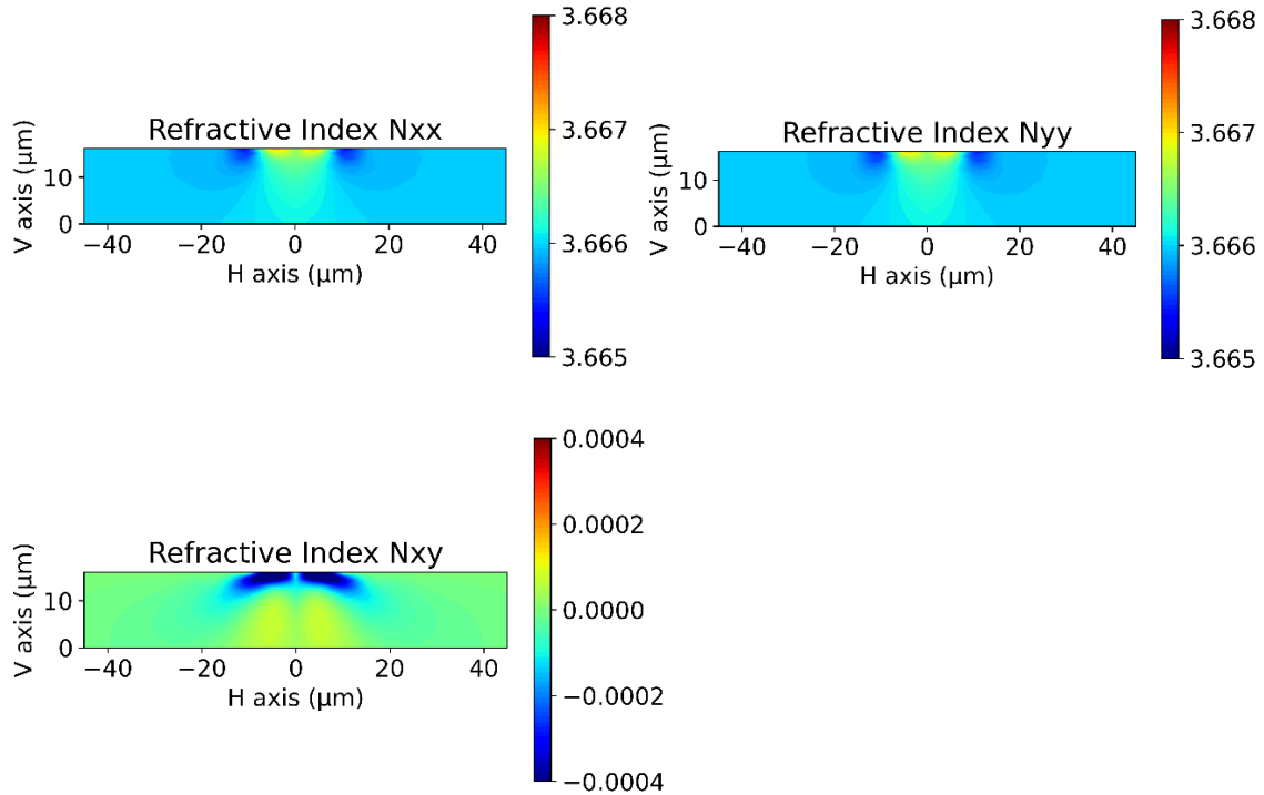
Figure 54: Simulation of refractive index distribution in the cross-section of GaAs under a 20 \mu\text{m} wide \text{SiN}_x stripe in compression at -280 MPa.
