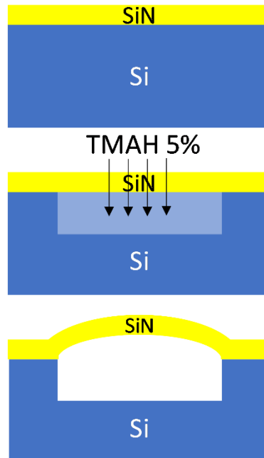
Figure 27: Cross-sectional schematic view of the process steps for fabricating a SiN x microbeam on top of a Si substrate using SiN x compressively strained films. [33]
