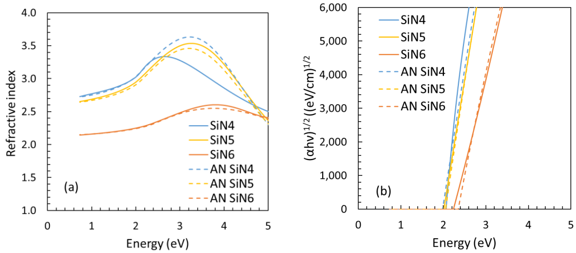
Figure 14: Refractive index (a) and Tauc plots (b) derived from the VASE measurements of \text{SiN}_x films deposited with different \text{N}_2 flows before and after a 400 °C annealing. “AN” indicates samples after annealing at 400 °C.
