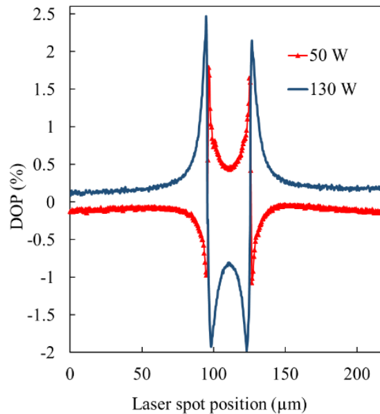
Figure 49: DOP-PL top surface GaAs for two different \text{SiN}_x 20 \mu\text{m} stripes (initial residual stress before etching: 285 MPa tensile in red (50 W) and -293 MPa compressive in blue (130 W)) deposited by a CCP reactor on GaAs substrate. [33]
