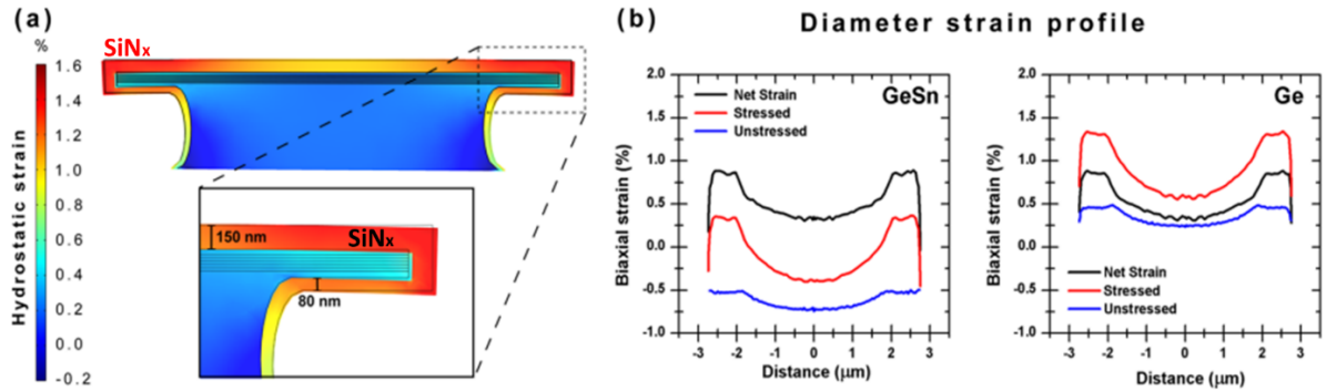
Figure 4: (a) Cross-section of the 3D finite element model showing the hydrostatic strain of a microdisk induced by the \text{SiN}_x stressor layer; the initial epitaxial strains are not included.
