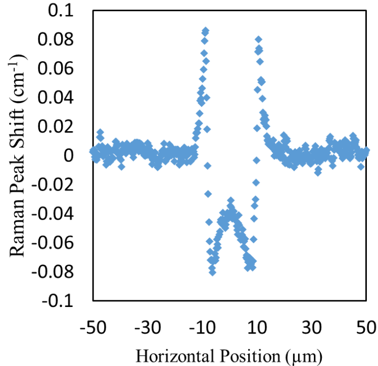
Figure 50: Raman shift profile measured from the surface across a \text{SiN}_x stripe deposited by PECVD on Si (stripe width 20 \mu\text{m} / built-in stress – 280 MPa).
