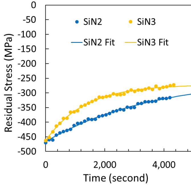
Figure 37: Stress-time curve of the samples SiN2 and SiN3 annealed at 400 °C for 1 hour and 10 minutes. The solid lines are the best fits of the experimental data using an exponential (Equation 15).
