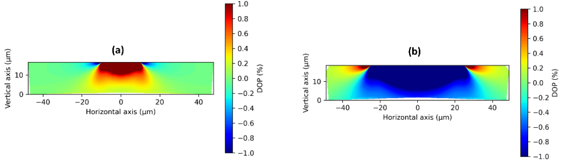
Figure 53: DOP-PL simulations for two different \text{SiN}_x stripes, a 20 \mu\text{m} stripe in tension 164\text{MPa} (a), and a 50 \mu\text{m} stripe in compression -280\text{MPa} (b), on GaAs substrates. [33]
