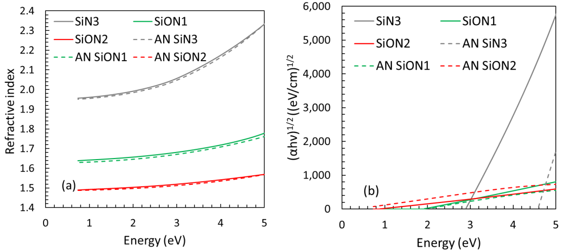
Figure 15: Refractive index (a) and Tauc plots (b) derived from the VASE measurements of \text{SiO}_y\text{N}_x films deposited with different \text{O}_2 flows before and after a 400 °C annealing. “AN” indicates samples after annealing at 400 °C.
