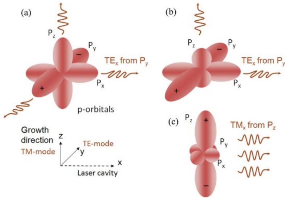
Figure 6: A qualitative illustration showing three p -orbitals P_x , P_y , and P_z of equal size for an unstrained bulk semiconductor (a). The variation of the p -orbitals size under biaxial compression is shown in (b), and under biaxial tension in (c). [16]
