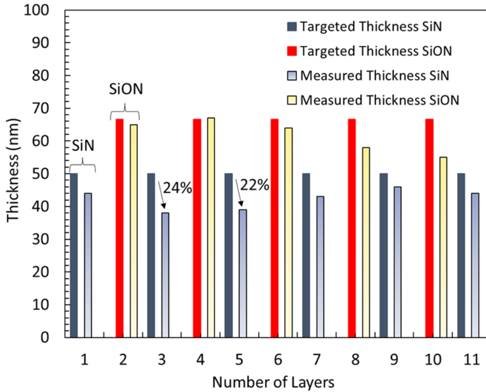
Figure 17: 11-layer notch filter structure with a quarter-wave thickness. The odd layers are \text{SiN}_x layers, and the even layers are \text{SiO}_y\text{N}_x layers. The targeted thickness values are in solid colors and the fitted thicknesses from the ellipsometry data are in grading colors.
