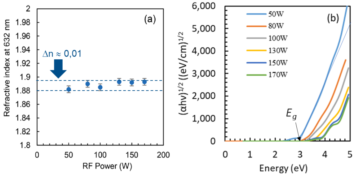
Figure 11: Refractive index at 632 nm (a) and Tauc plots derived from the optical absorption measurements (b) of the 500 nm \text{SiN}_x films deposited within the CCP reactor. [33]
