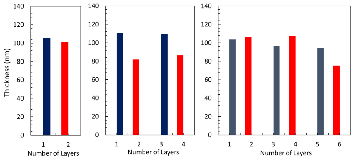
Figure 16: Three multilayer structures with 2, 4, and 6 layers of 100 nm each deposited on a Si substrate. The odd layers in blue are \text{SiN}_x layers, and the even layers in red are \text{SiO}_y\text{N}_x layers. The thickness values are estimations made by fitting ellipsometry data.
