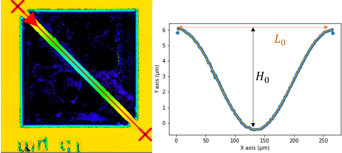
Figure 31: Confocal measurement of a 15 \mu\text{m} wide microbeam buckling downward (left) and the best fits of the experimental deformation profile using Equation 11 (right).
