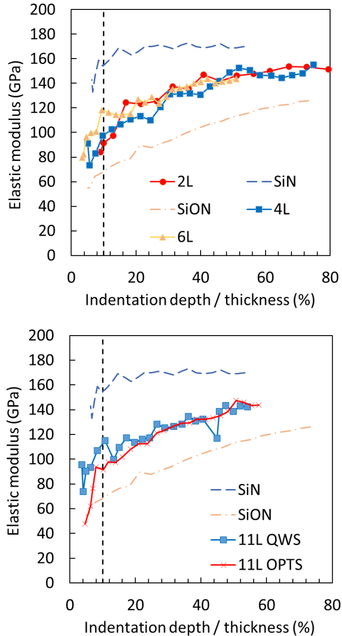
Figure 45: Elastic modulus of \text{SiN}_x -based monolayers and multilayers on Si substrate versus normalized indentation depth.
