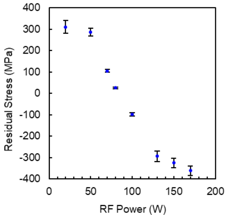
Figure 32: Residual stress vs. excitation power for 500 nm \text{SiN}_x films deposited within the CCP reactor. [33]
