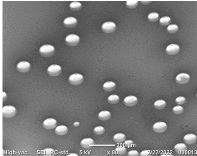
Figure 38: Scanning electron microscopy image of post-thermal-cycling delamination on sample SiN1 tilted at a 45-degree angle.
