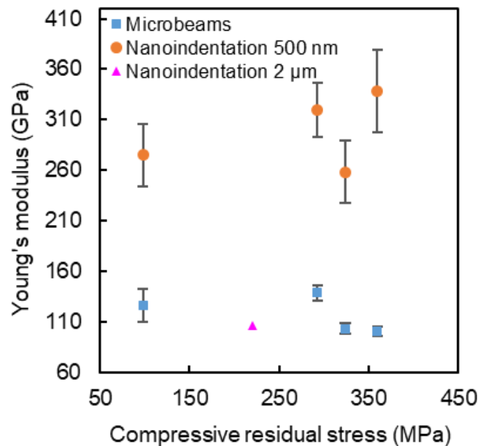
Figure 42: Elastic modulus of SiN x films with compressive built-in stress deposited on Si using a CCP reactor. [33]
