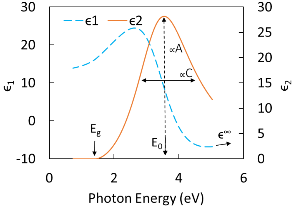
Figure 10: Tauc-Lorentz model. The real (blue dashed line) and imaginary (orange solid line) components are plotted for a model material with A = 170 eV, C = 2.2 eV, E_g = 1.39 eV, E_0 = 3.5 eV, and \epsilon^\infty = 0.6 . Produced using CompleteEASE software of the VASE.
