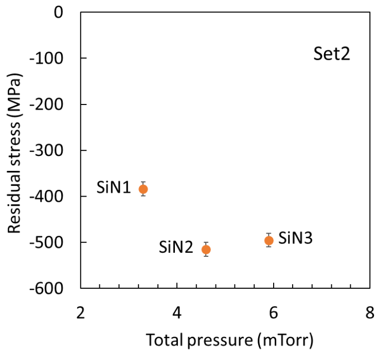
Figure 35: Residual mechanical stress vs. total deposition pressure for SiN_x films deposited within the ECR reactor. The samples correspond to Set 2 from Table 3.
