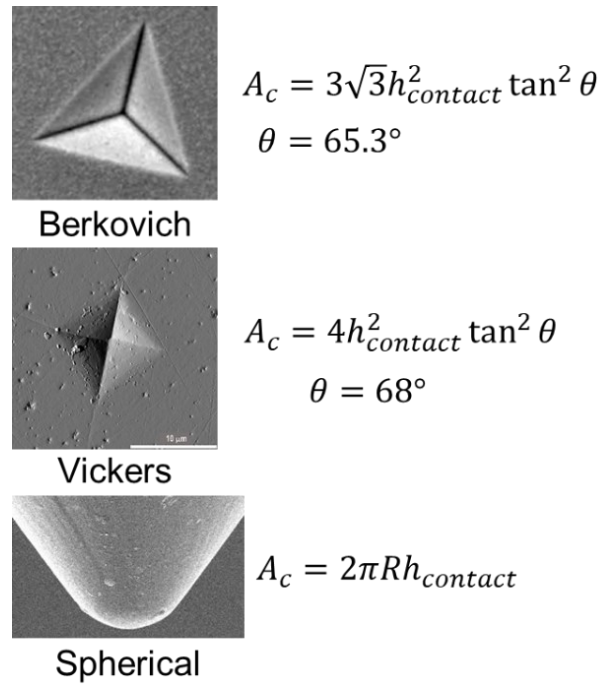
Figure 24: Examples from different geometries of indenter tips.[72]
