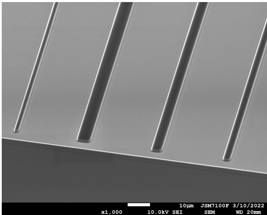
Figure 48: \text{SiN}_x stripes on GaAs obtained after deposition with the CCP reactor and a dry etching process using an \text{SF}_6 plasma.
