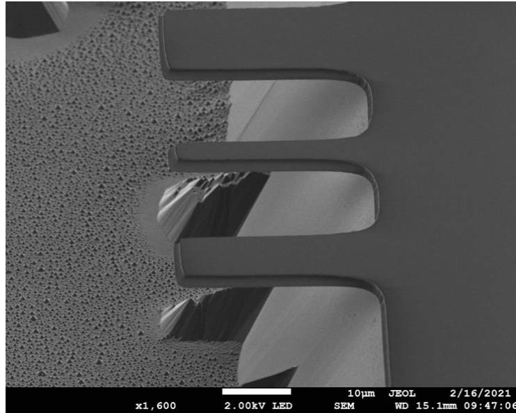
Figure 29: SEM image of cantilevers fabricated from a \text{SiN}_x film deposited on a Si substrate using a CCP reactor with 130 W RF power (compressive built-in stress: -300 MPa).
