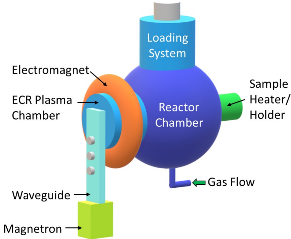
Figure 8: Schematic drawing of the interconnection of the main sub-systems of the ECR-PECVD reactor.
