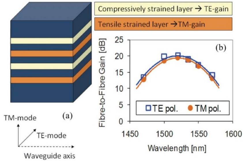
Figure 2: A series of compressive and tensile films can be designed to be mechanically stable (a) and equally amplify both TE and TM modes to produce polarization-insensitive semiconductor optical amplifiers as shown in (b) [16–18]
