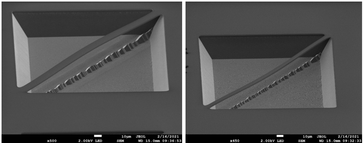
Figure 30: SEM image of microbeams buckling upward (left) and downward (right) fabricated from a \text{SiN}_x film deposited on Si by PECVD with 130 W RF power (compressive built-in stress: -300 MPa).
