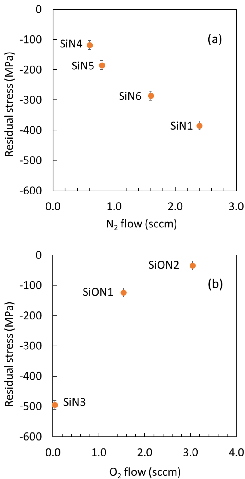
Figure 34: Residual mechanical stress vs. N 2 or O 2 flows for Si x N y films deposited within the ECR reactor. The samples correspond to Sets 3 and 4 from Table 3.
