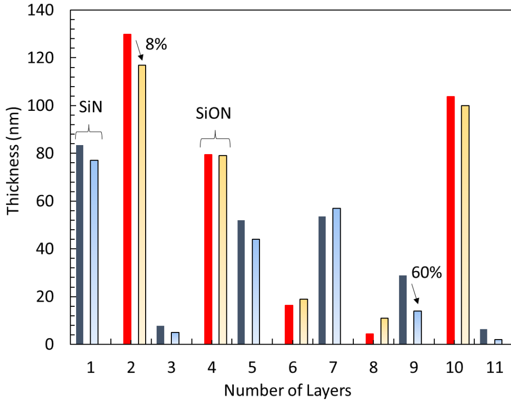
Figure 19: 11-layer notch filter structure with an optimized thickness profile. The odd layers are SiN x layers, and the even layers are SiO y N x layers. The targeted thickness values are in solid colors, and the fitted thicknesses from the ellipsometry data are in grading colors.
