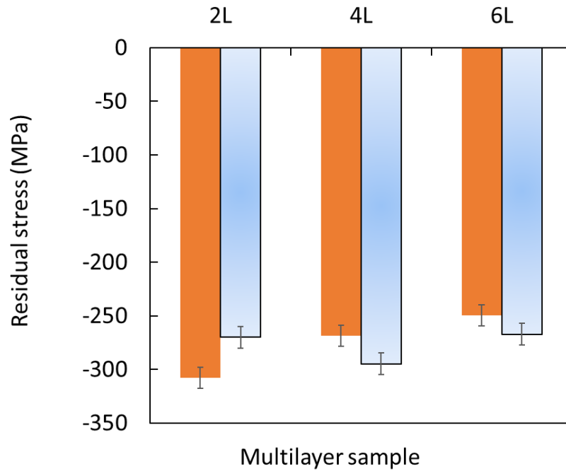
Figure 43: Three multilayer structures with 2, 4, and 6 layers of 100 nm each deposited on a Si substrate. The measured residual stress values are in solid orange color, and the predicted residual stress values are in a grading blue color.
