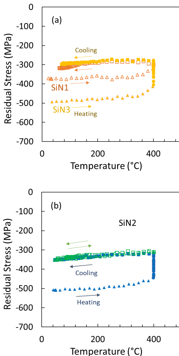
Figure 36: (a) Stress-temperature curves of the sample SiN1 plotted in open orange symbols and SiN3 plotted in solid yellow symbols. (b) Stress-temperature curve of the sample SiN2 doubly-thermally-cycled. Data points collected during the first thermal cycle are in solid
