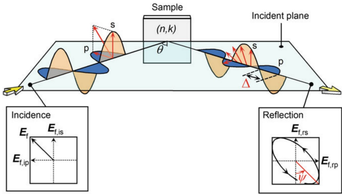
Figure 9: Basic principle of ellipsometry from Fujiwara [61]. The light polarization is categorized into p - and s -polarizations depending on the oscillatory direction of the electric field ( E_f ). The p -polarization is parallel to the incident plane, while the s -polarization is perpendicular. The E_f shows the electric field vector, and the subscripts “i”, “r”, “s”, and “p” for E_f denote the incidence, reflection, s -polarization, and p -polarization, respectively.
