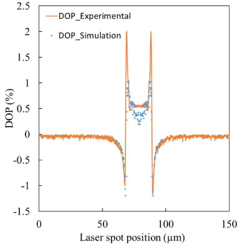
Figure 52: A comparison of DOP-PL simulations with DOP-PL line scans on the top surface of a 20 \mu\text{m} \text{SiN}_x stripe with 164 MPa tensile stress. [33]
