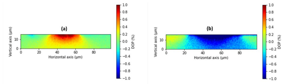
Figure 51: DOP-PL cross-section of GaAs for two different SiN x stripes (20 μm stripe in tension at 164 MPa (a) and 50 μm stripe in compression at -280 MPa (b)) deposited within the CCP reactor on GaAs substrates. [33]
