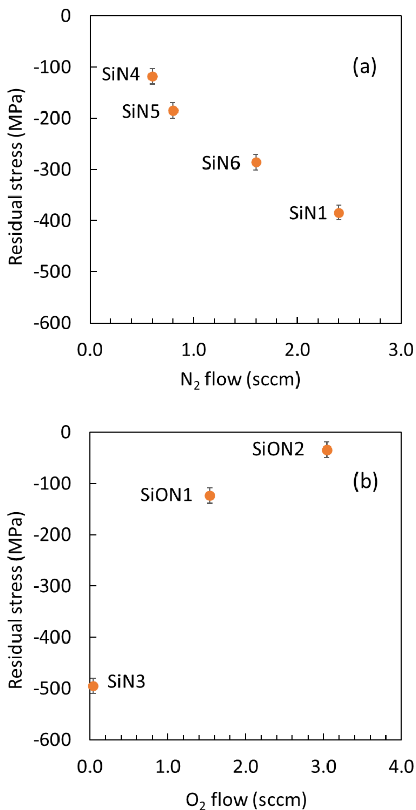
Figure 34: Residual mechanical stress vs. N 2 or O 2 flows for Si x N x films deposited within the ECR reactor. The samples correspond to Sets 3 and 4 from Table 3.
