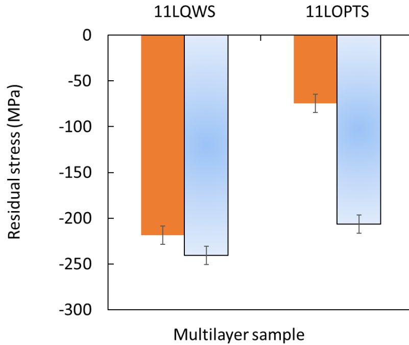
Figure 44: 11-layers notch filter structures with a QWS and an OPTS profiles. The measured residual stress values are in solid orange color and the predicted residual stress values are in grading blue color.
