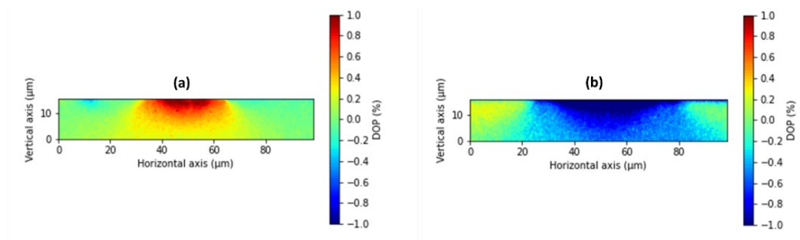
Figure 51: DOP-PL cross-section of GaAs for two different \text{SiN}_x stripes (20 \mu\text{m} stripe in tension at 164 MPa (a) and 50 \mu\text{m} stripe in compression at -280 MPa (b)) deposited within the
