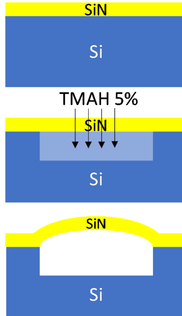
Figure 27: Cross-sectional schematic view of the process steps for fabricating a \text{SiN}_x microbeam on top of a Si substrate using \text{SiN}_x compressively strained films. [33]
