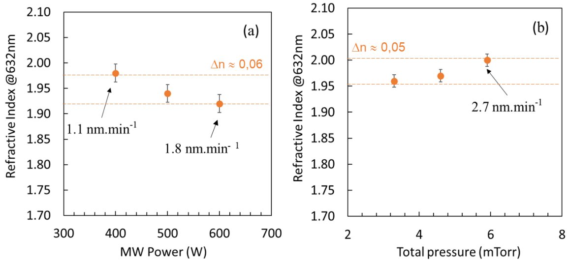
Figure 12: Refractive index at 632 nm of 500 nm SiN x films deposited within the ECR reactor at three different deposition powers (a) and pressures (b). The samples (a) correspond to Set 1 from Table 2 and samples (b) correspond to Set 2 from Table 3.
