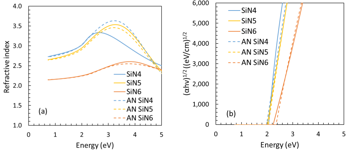
Figure 14: Refractive index (a) and Tauc plots (b) derived from the VASE measurements of \text{SiN}_x films deposited with different \text{N}_2 flows before and after a 400 °C annealing. “AN” indicates samples after annealing at 400 °C.
