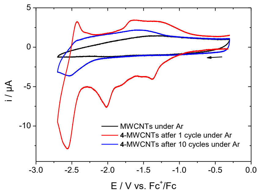
Figure IV.10. CV at a 4-MWCNTs modified glassy carbon electrode in THF/NBu 4 PF 6 0.1 M under Ar. Red: first cycle; Blue: after 10 cycles. The black line shows the CV of a bare MWCNTs glassy carbon electrode in the same conditions. Conditions: Ag/AgNO 3 (RE), 0.1 V s -1 .
