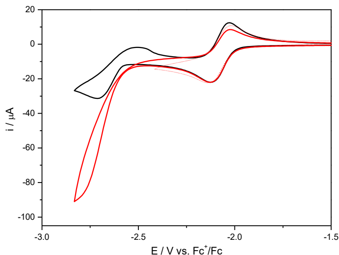
Figure II.23. CVs of complex \mathbf{1}^{\text{tBu}} in THF/ 0.1 M NBu 4 PF 6 under Ar (black) and CO 2 (red). Cyclic voltammetry of \mathbf{1}^{\text{H}} first reduction process was studied separately. The dashed curve corresponds to the CV for the first reduction process only under carbon dioxide. Conditions: 1 mM of complex, BDD working electrode, \nu = 0.1 \text{ V s}^{-1} .
