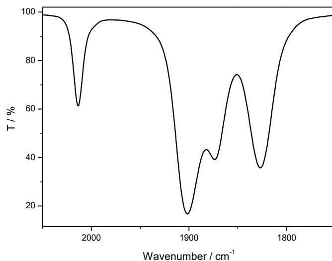
Figure IV.7. IR spectra of complex 4 in THF.
