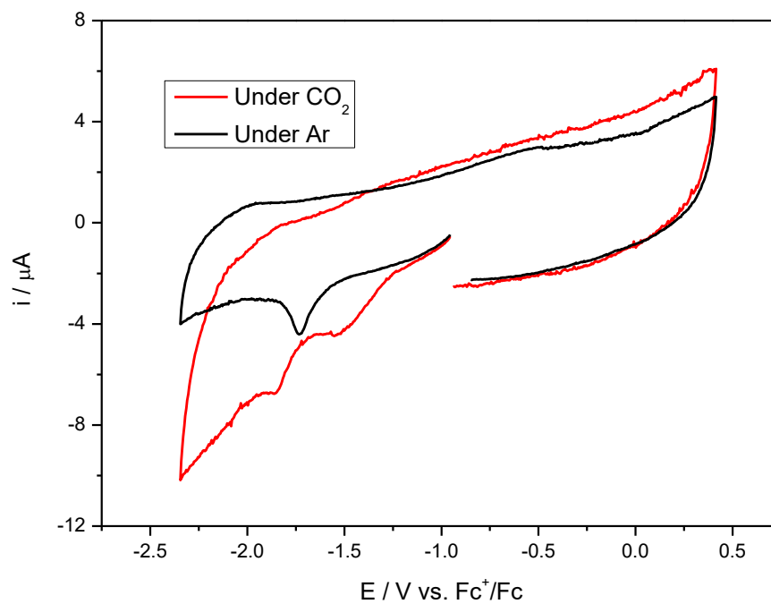
Figure IV.16. CV of a complex 5 -functionalized glassy carbon electrode in MeCN / NBu 4 PF 6 0.1 M under Ar (black) and under CO 2 (red) at \nu = 0.1 \text{ V s}^{-1} .
