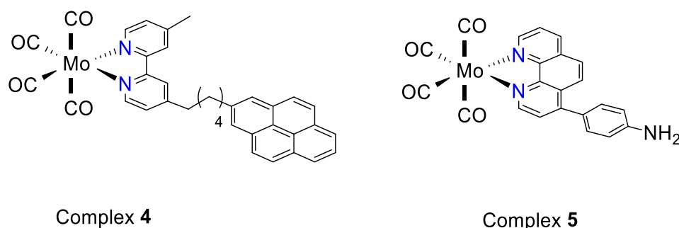
Figure IV.6. Schematic representation of complexes 4 and 5 investigated in this chapter.
