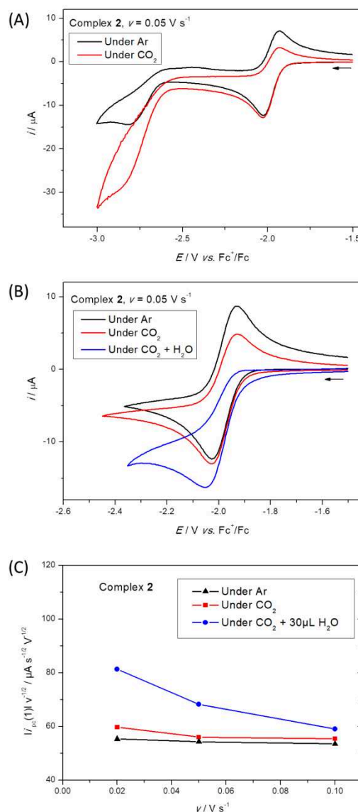
Figure 3. CVs ( E / \text{V vs. Fc}^+/\text{Fc} ) at a BDD working electrode of complex 2 (1 mM), in dry THF/NBu 4 PF 6 0.1 M; Panel A: For \nu = 0.05 \text{ V s}^{-1} under argon (black) and CO 2 (red); Panel B: For \nu = 0.05 \text{ V s}^{-1} under argon (black), under CO 2 (red), and under CO 2 + 0.1% H 2 O ( \nu ) (blue); Panel C: Plots of |i_{pc}(1)| \nu^{1/2} / \mu\text{A s}^{1/2} \text{V}^{1/2} against \nu under Ar (black), under CO 2 (red), and under CO 2 + 0.1% H 2 O (blue).
