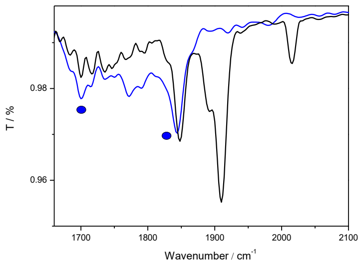
Figure II.21. Infrared spectra of the bis-reduced (blue) and neutral (black) species 1 CF 3 in THF/ 0.1 M NBu 4 PF 6 . Conditions: 5 mM of complex, GC working electrode, under Ar.
