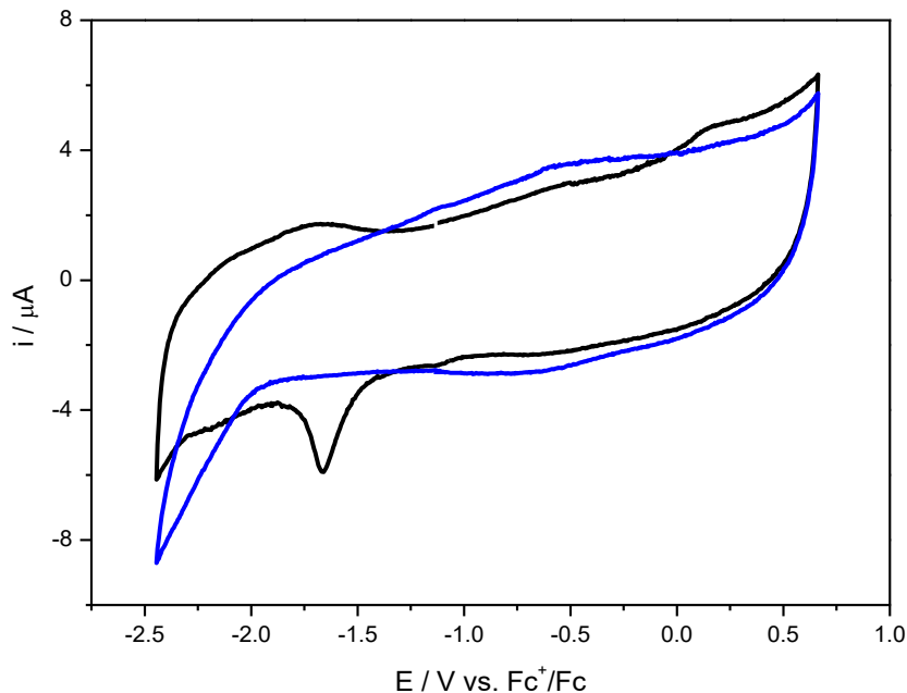
Figure IV.15. CV of bare (blue) and complex 5 -functionalized (black) glassy carbon electrodes in MeCN / NBu 4 PF 6 0.1 M under Ar at \nu = 0.1 \text{ V s}^{-1} .
