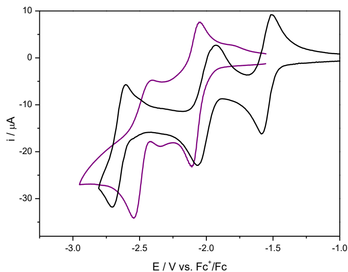
Figure II.8. CVs of A) 1 CO 2 Me (black) and B) bpy-(CO 2 Me) 2 ligand (purple) in THF / 0.1 M NBu 4 PF 6 under Ar. Conditions: 1 mM of complex, BDD working electrode, \nu = 0.1 \text{ V s}^{-1} .
