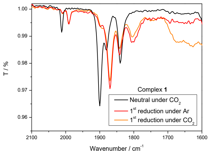
Figure III.29. IR-SEC spectra of complex 1 in THF under Ar at neutral state (black), after the first reduction under Ar (red) and under CO 2 (orange). Conditions: 5 mM of complex, 0.1 M NBu 4 PF 6 , GC working electrode.
