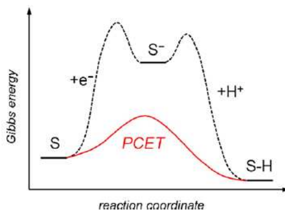
Figure I.17. General PCET energetic profile. Reproduced from Ref. [29].
