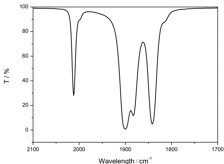
Figure II.3. Infrared spectrum of 1 H in MeCN.
