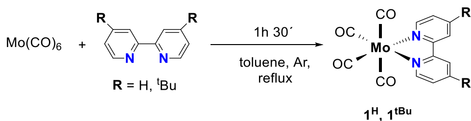
Scheme II.1. Synthetic pathway for 1 H and 1 tBu .
