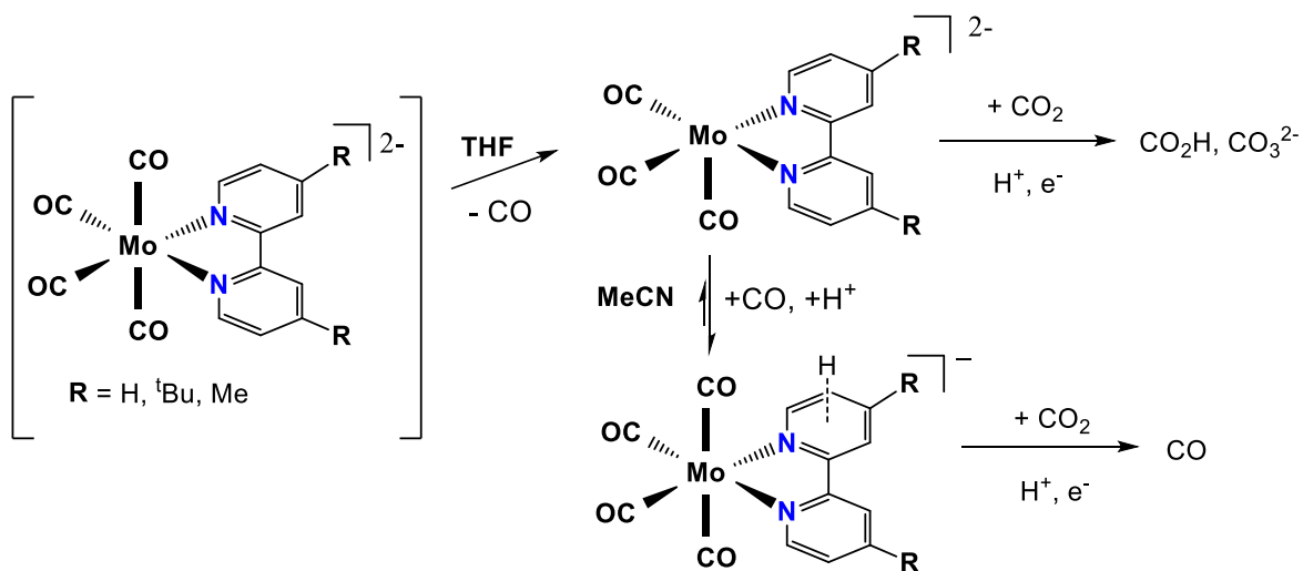
Scheme II.4. Reactivity of [\text{Mo}(\text{CO})_4(\text{bpy}-(\text{R})_2)]^{2-} with carbon dioxide in different solvents.
