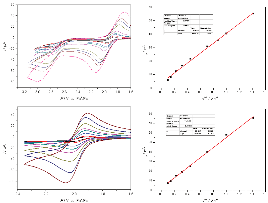
Figure III.8. CVs of complex 2 (top) and 1 (bottom) at 0.01 \text{ V s}^{-1} < \nu < 2 \text{ V s}^{-1} . Top right panels: plots of i_{pc} vs. \nu^{1/2} for the first reversible system. Conditions: 1 mM of complex, THF / NBu 4 PF 6 0.1 M, BDD WE, under argon.
