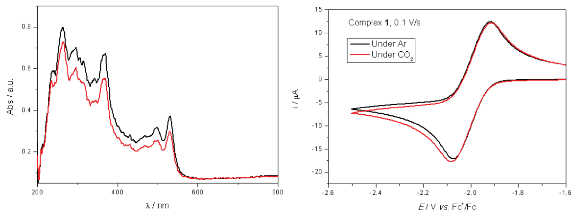
Figure II.25. [Mo(CO) 4 (bpy-(H) 2 )] •- absorption spectra (left) and cyclic voltammetry (right) under Ar (black) and CO 2 (red) atmosphere in THF/ 0.1 M NBu 4 PF 6 . Conditions: 1 mM of complex, BDD working electrode, \nu = 0.1 \text{ V s}^{-1} .
