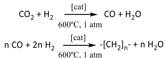
Scheme I.2. Reaction scheme of the modified Fischer-Tropsch process.
