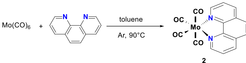
Scheme III.1. Synthetic pathway for complex 2 .
