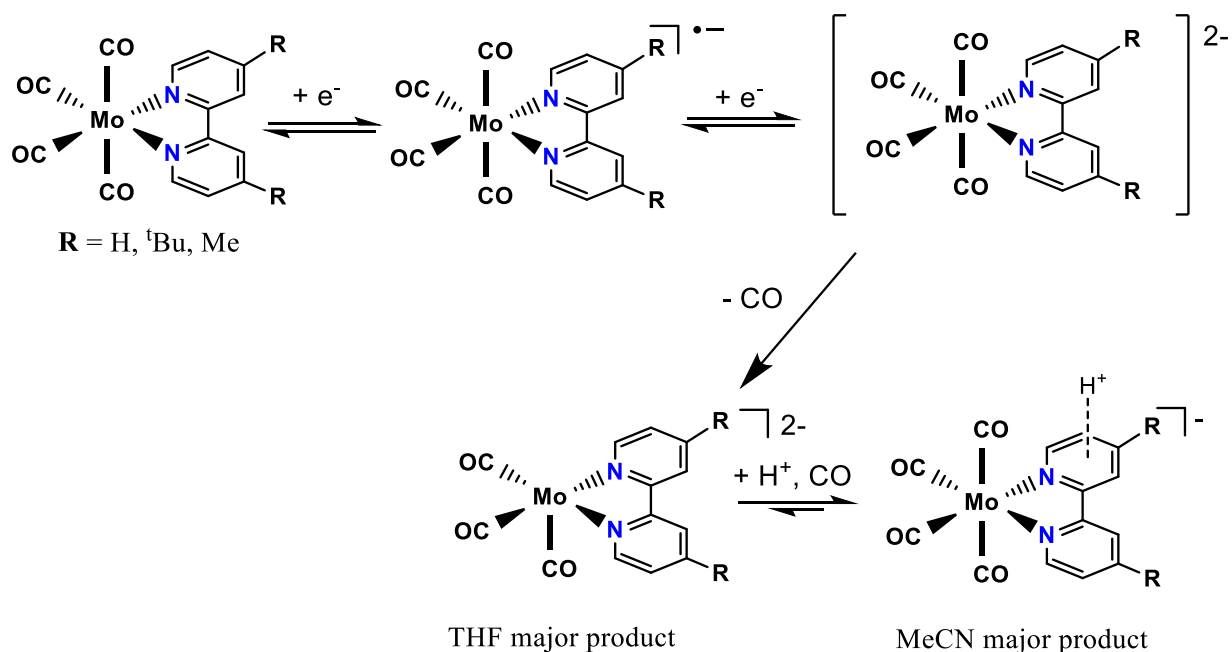
Scheme II.3. Reduction processes of 1 H , 1 tBu and 1 Me systems in MeCN and THF.
