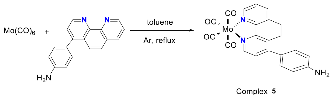
Scheme IV.2. Synthetic pathway for complex 5.
