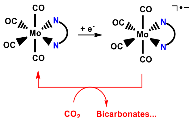
Figure V.2. Interaction of [Mo(CO) 4 (diimine)] mono-reduced species with carbon dioxide.
