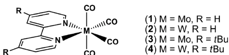
Figure II.1. Schematic representation of [M(CO) 4 (bpy-R 2 )] (M = W, Mo; R=H, t Bu) systems. Reproduced from Ref. [6].
