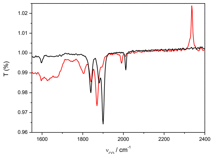
Figure II.28. IR-SEC spectra of complex 1 H in THF/ 0.1 M NBu 4 PF 6 at the neutral state (black) and after the first reduction (red) under CO 2 . Conditions: 5 mM of complex, GC working electrode.
