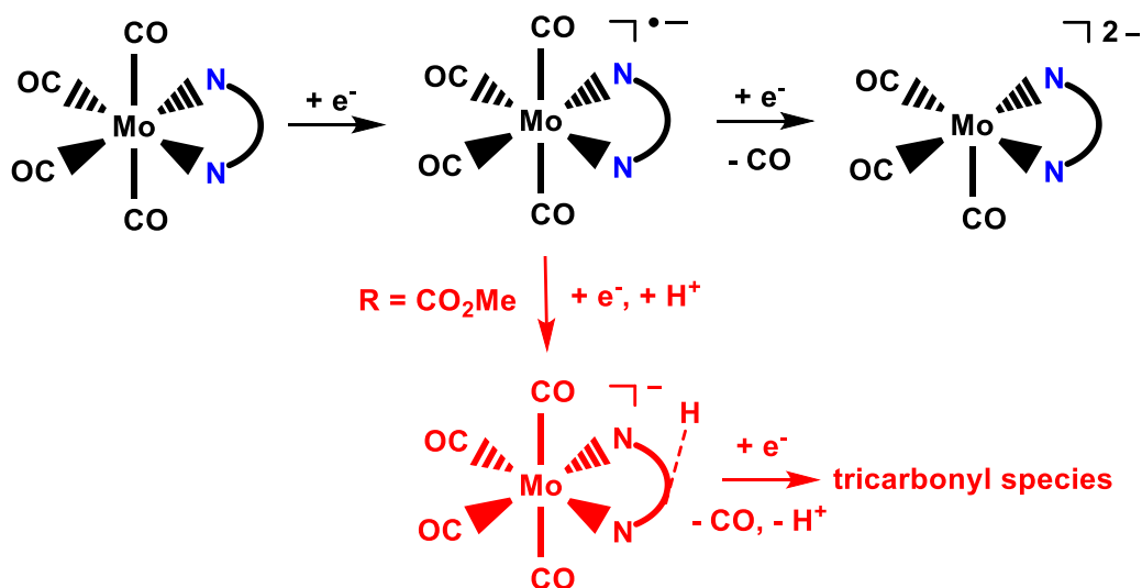
Figure V.1. Reduction pathways of [Mo(CO) 4 (bpy-(R) 2 )] complexes.
