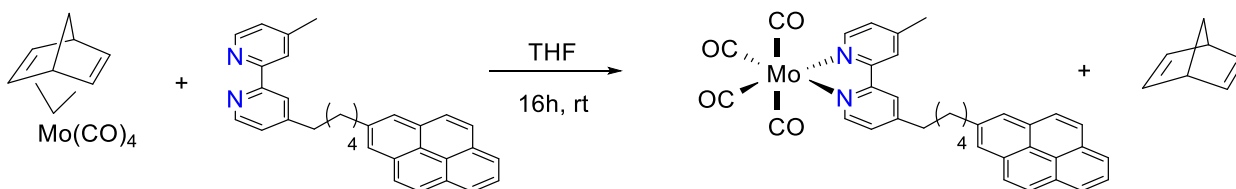
Scheme IV.1. Synthetic pathway for complex 4 .
