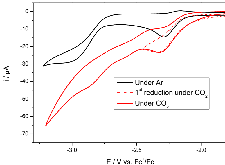
Figure III.19. CVs of complex 3 in THF under Ar (black) and CO 2 (red). The dashed curve corresponds to the CV for the first reduction process only. Conditions: 1 mM of complex, 0.1 M NBu 4 PF 6 , BDD working electrode, \nu = 0.1 \text{ V s}^{-1} .
