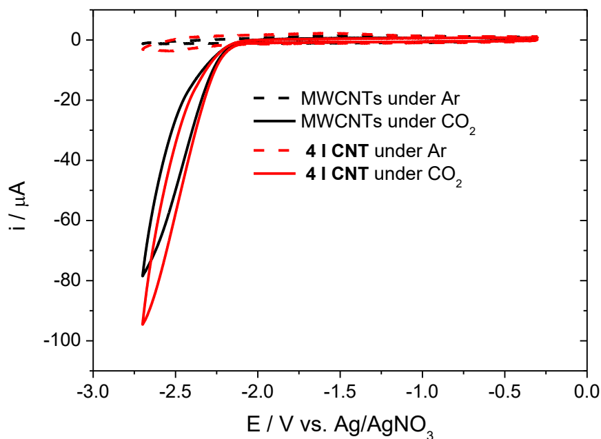
Figure IV.11. CVs of 4I-CNT modified glassy carbon electrodes (red) and bare MWCNT GC electrodes (black) under Ar (dashed) and CO 2 (plain) in THF / NBu 4 PF 6 , 0.1 M. Ref: Ag/AgNO 3 , \nu = 0.1 \text{ V s}^{-1} .
