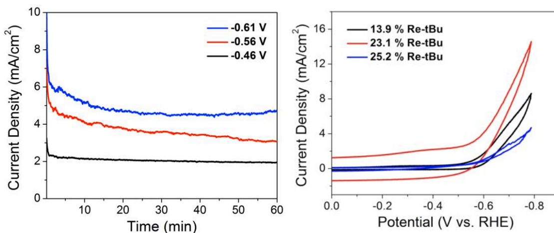
Figure I.23. Left: CPE responses at different potentials vs RHE under CO 2 . Right: CV responses for different catalytic loading onto MWCNTs under CO 2 . Reproduced from Ref. [106].
