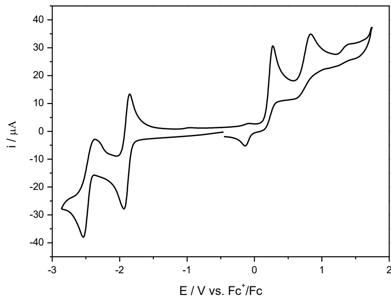
Figure I.25. CV ( \nu = 100 \text{ V s}^{-1} ) of [\text{Mo}(\text{CO})_4(\text{bpy})] (1 mM) at a glassy carbon working electrode in THF / \text{NBu}_4\text{PF}_6 (0.1 M).
