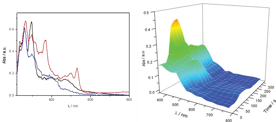
Figure II.26. Absorption spectra of bis-reduced (blue), mono-reduced (red) and neutral (black) species of 1 H in THF / 0.1 M NBu 4 PF 6 (left) with its corresponding 3D monitoring graph (right). Conditions: 1 mM of complex, BDD (WE), thin layer condition, 0.2 mm optical path, under CO 2 .
