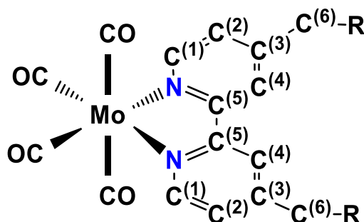
Figure II.37. Atom numbering for the calculated structures of [Mo(CO) 4 (bpy-(R) 2 )] (R = CO 2 Me, CF 3 ) complexes.
