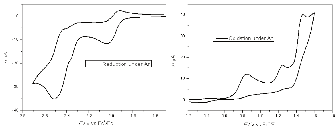
Figure IV.8. CV of complex 4 at a BDD working electrode in THF/NBu 4 PF 6 0.1 M under Ar. Conditions: 1 mM of complex, \nu = 0.1 \text{ V s}^{-1} .
