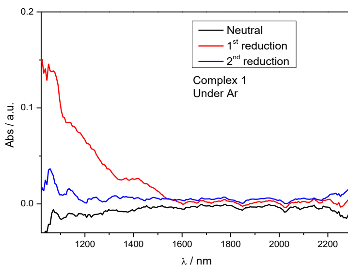
Figure III.17. Near-IR spectra of neutral (black), mono-reduced (red) and bis-reduced (blue) species of complex 1 in THF. Conditions: 5 mM of complex, 0.1 M NBu 4 PF 6 , GC working electrode, 0.2 mm optical path, under Ar.
