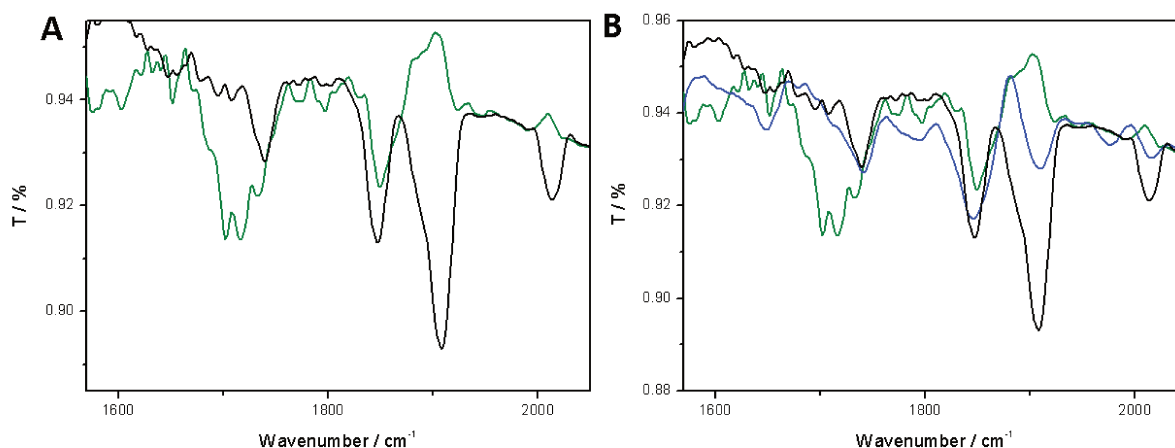
Figure II.20. Infrared spectra of the tris-reduced (green) and neutral (black) species of 1 CO 2 Me in THF/ 0.1 M NBu 4 PF 6 . For B) the blue trace represents the bis-reduced form of 1 CO 2 Me . Conditions: 5 mM of complex, GC working electrode, under Ar.
