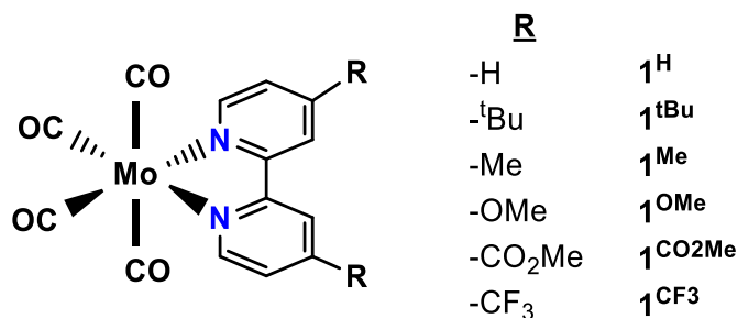
Figure II.2. General structure of [Mo(CO) 4 (bpy-(R) 2 )] derivatives studied in the present work.
