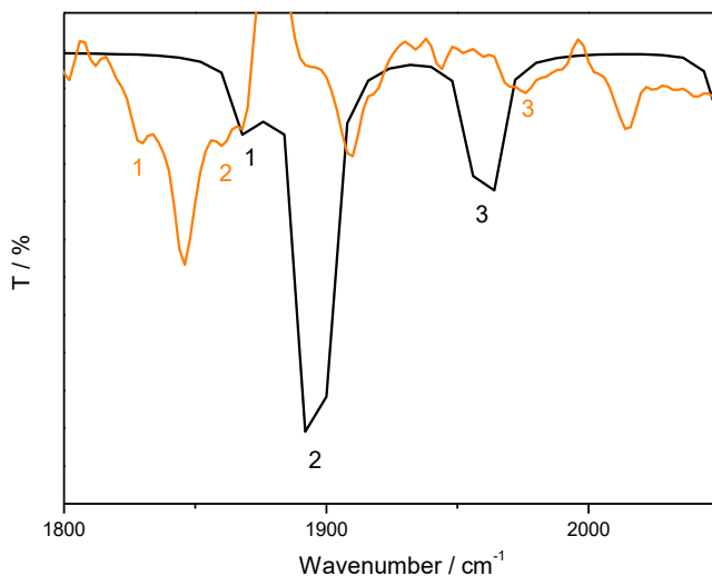
Figure II.36. IR spectra of [Mo(CO) 4 (bpy-(CO 2 Me) 2 )] 2- . The black and orange traces represent the theoretical and experimental spectra obtained in THF/ 0.1 M NBu 4 PF 6 respectively. The numbers correspond to the main ν CO bands of the species. Conditions: 5 mM of complex, GC (WE).
