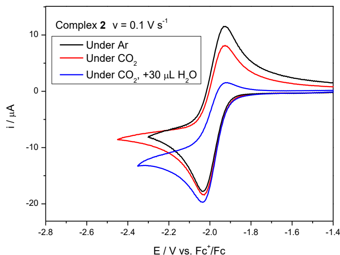
Figure III.23. CV of complex 2 in THF under Ar (black), under CO 2 (red) and under CO 2 with added water (0.5 M, blue). Conditions: 1 mM of complex, 0.1 M NBu 4 PF 6 , BDD working electrode, \nu = 0.1 \text{ V s}^{-1} .
