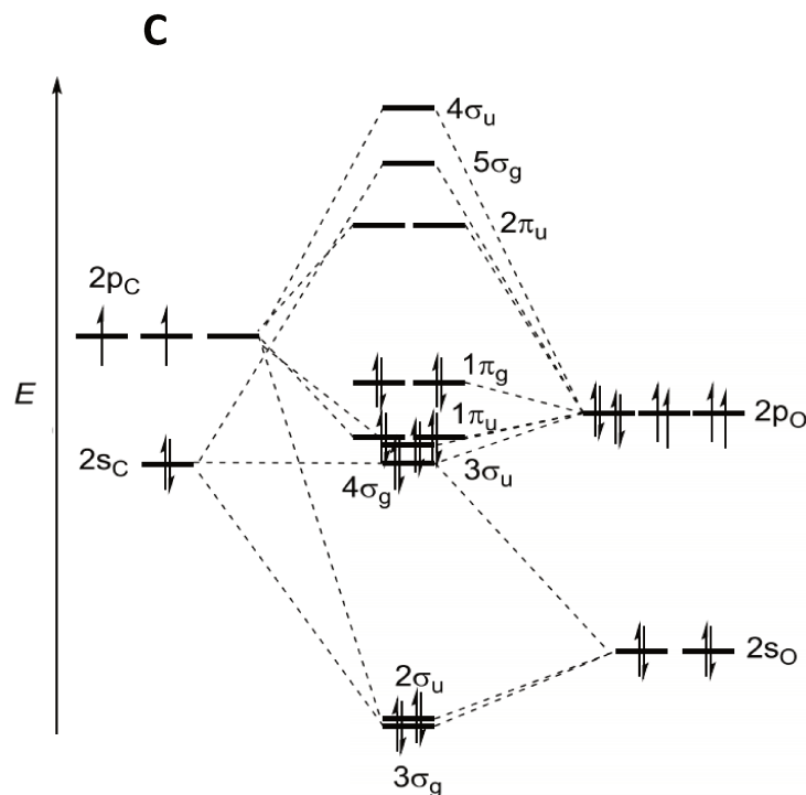
Figure I.10. Simplified MO diagram of the CO 2 molecule. Reproduced from Ref. [41].
