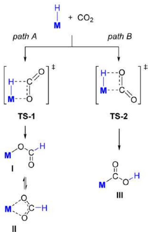
Figure I.14. Schematic representation of the different CO 2 insertion modes in a metal-hydride (M-H) bond. Reproduced from Ref. [29].
