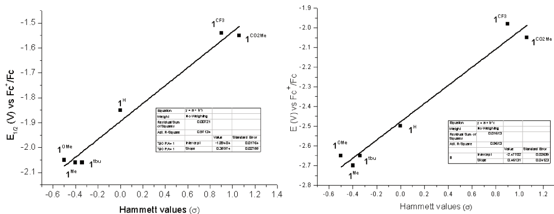
Figure II.10. Hammett plots of potential values for first (left) and second (right) reduction processes versus \sigma_p Hammett parameters of the R groups in [Mo(CO) 4 (bpy-(R) 2 )] complexes.
