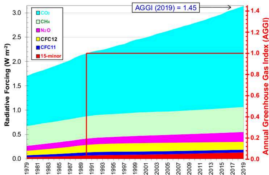
Figure I.3. Radiative forces of greenhouse gases until 2019. Reproduced from Ref. [8].
