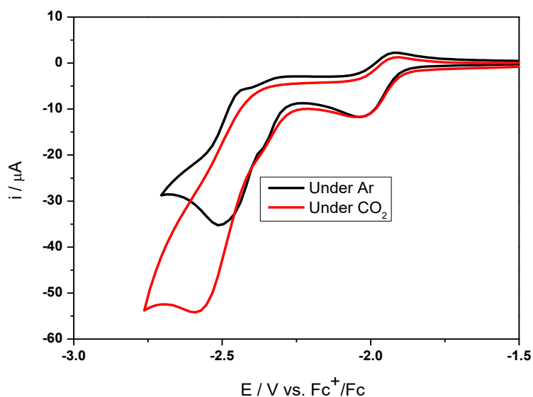
Figure IV.9. CV of complex 4 at a BDD working electrode in THF/NBu 4 PF 6 0.1 M under CO 2 (sat.). Conditions: 1 mM of complex, \nu = 0.1 \text{ V s}^{-1} .
