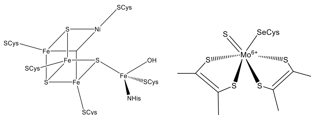
Figure I.7. Schematic representation of carbon dioxide dehydrogenase (left) and formate dehydrogenase (right) systems.
