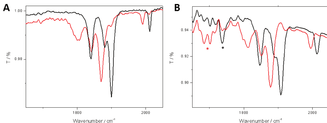
Figure II.17. Infrared spectra of neutral (black) and mono-reduced (red) forms of complex 1 H (A) and 1 CO 2 Me (B) under Ar in THF / 0.1 M NBu 4 PF 6 . Dots indicate the C=O frequency band of -CO 2 Me group. Conditions: 5 mM of complex, GC working electrode, under Ar.
