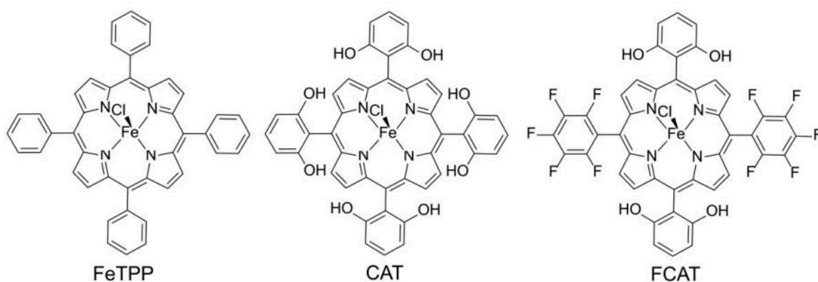
Figure I.19. Iron-substituted porphyrin complexes for PCET CO 2 reduction. Reproduced from Ref. [72].
