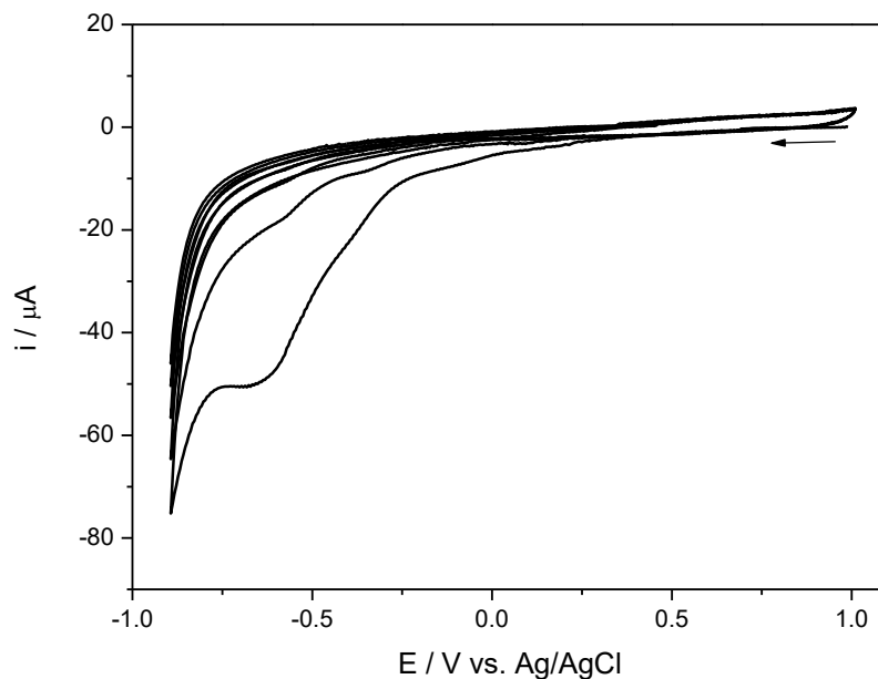
Figure IV.14. CVs of the diazonium solution of complex 5 at a GC working electrode in MeCN / NBu 4 PF 6 0.1 M (0 °C) under Ar. Conditions: \nu = 0.1 \text{ V s}^{-1} . See text for details.
