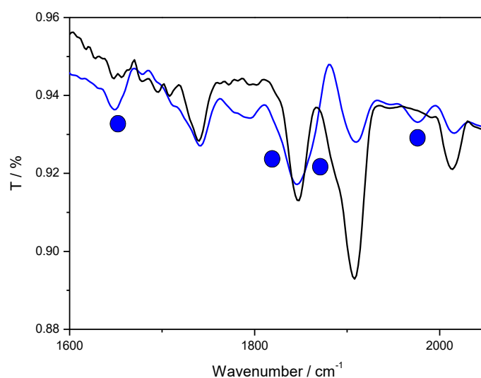
Figure II.19. Infrared spectra of the bis-reduced (blue) and neutral (black) species of \mathbf{1}^{\text{CO}_2\text{Me}} in THF/0.1 M NBu 4 PF 6 . Conditions: 5 mM of complex, GC working electrode, under Ar.
