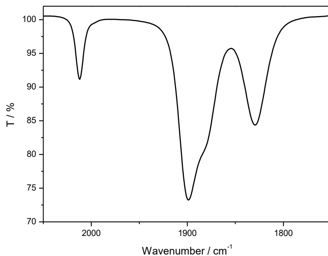
Figure IV.12. IR spectra of complex 5 in THF.
