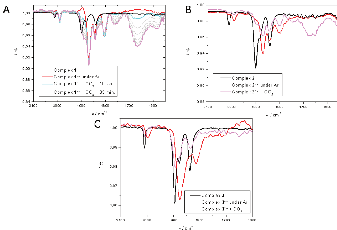
Figure III.34. IR spectra of chemically mono-reduced species under Ar (red) and CO 2 (pink) species in comparison with neutral species under CO 2 (black) in THF for A) complex 1 , B) complex 2 and C) complex 3 . Conditions: 5 mM of complex, 0.1 M NBu 4 PF 6 , GC working electrode. The cyan and grey curves in A represent intermediates curves during reaction of 1 •- with CO 2 .
