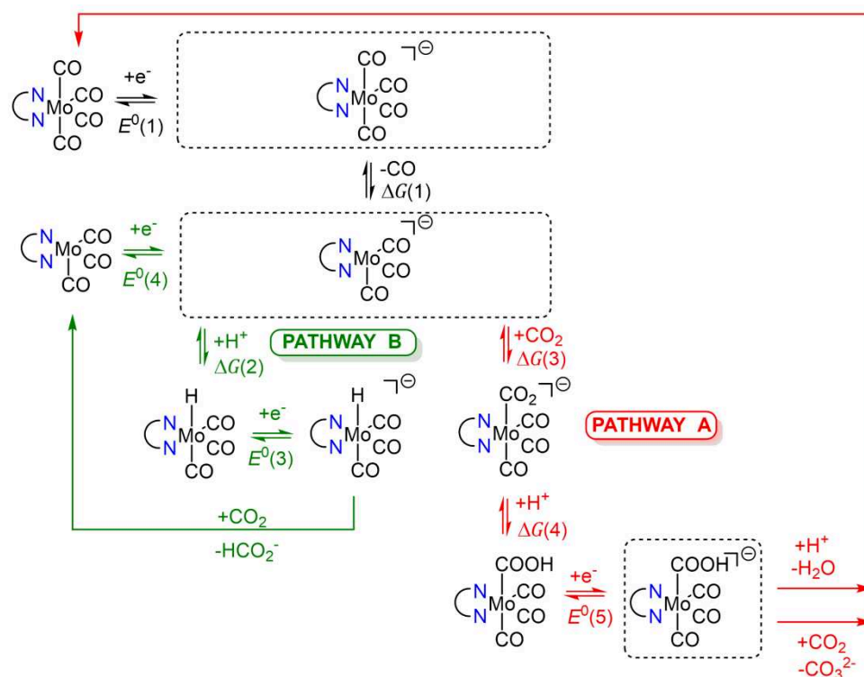
Scheme 2. Suggested mechanistic pathways for the \text{CO}_2 reduction mediated by Mo-dimine complexes 1 , 2 and 3 .
