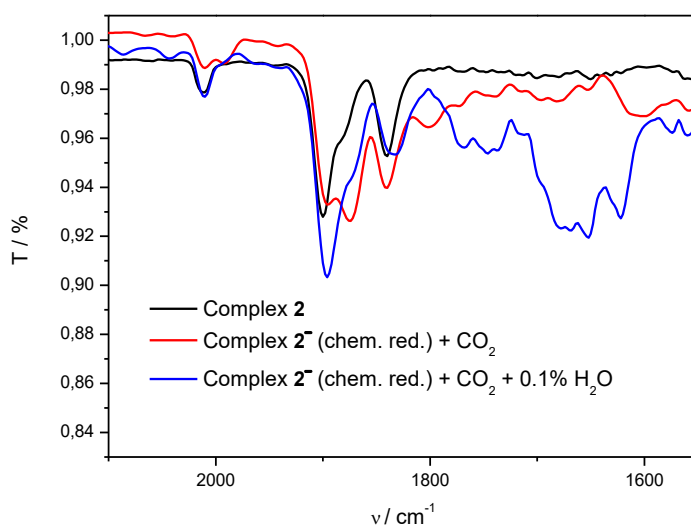
Figure III.35. IR spectra of chemically mono-reduced 2 in distilled THF under Ar (black), under CO 2 (red) and under CO 2 with added water (blue). Conditions: 5 mM of complex, 0.1 M NBu 4 PF 6 , GC working electrode.
