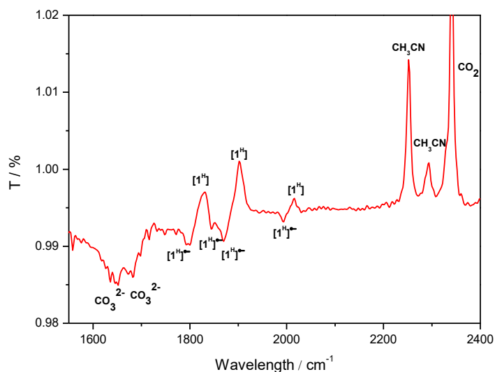
Figure II.29. 1^{\text{H}} differential infrared spectra of [\text{Mo}(\text{CO})_4(\text{bpy}-(\text{H})_2)]^{\bullet-} (red) under \text{CO}_2 in MeCN / 0.1 M \text{NBu}_4\text{PF}_6 . Consumption of \text{CO}_2 and MeCN is observed in the 2200-2400 \text{cm}^{-1} region. Conditions: 5 mM of complex, GC (WE).
