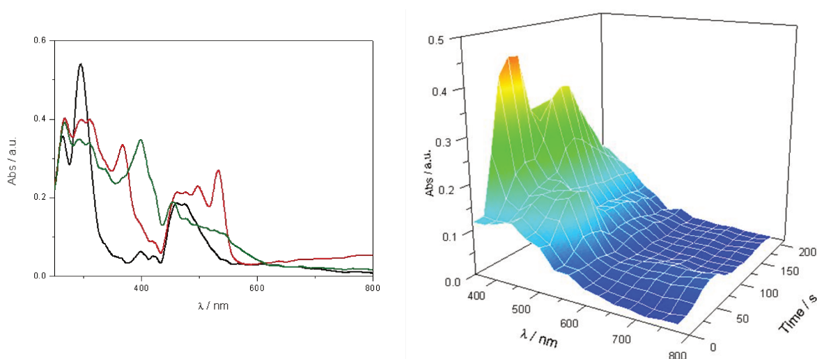
Figure II.14. Absorption spectra of bis-reduced (green), mono-reduced (red) and neutral (black) species of complex 1 H in MeCN / NBu 4 PF 6 0.1 M (left) with its corresponding 3D monitoring graph (right). Conditions: 1 mM of complex, 0.1 M NBu 4 PF 6 , BDD (WE), thin layer condition, 0.2 mm optical path, under Ar.
