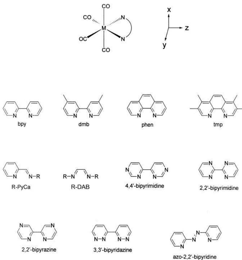
Figure III.1. Schematic representation of [M(CO) 4 (diimine)] systems (M = Cr, Mo, W). Reproduced from Ref. [1].
