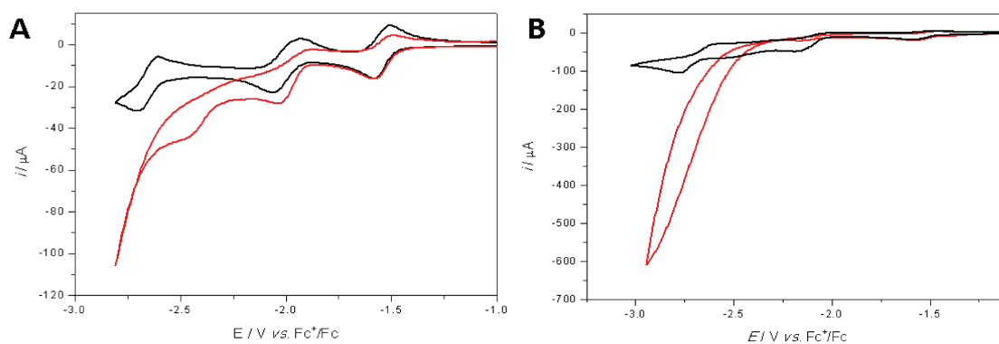
Figure II.24. CVs of A) 1 CO 2 Me and B) 1 CF 3 in THF/ 0.1 M NBu 4 PF 6 under Ar (black) and CO 2 (red). Conditions: 1 mM of complex, BDD working electrode, \nu = 0.1 \text{ V s}^{-1} .
