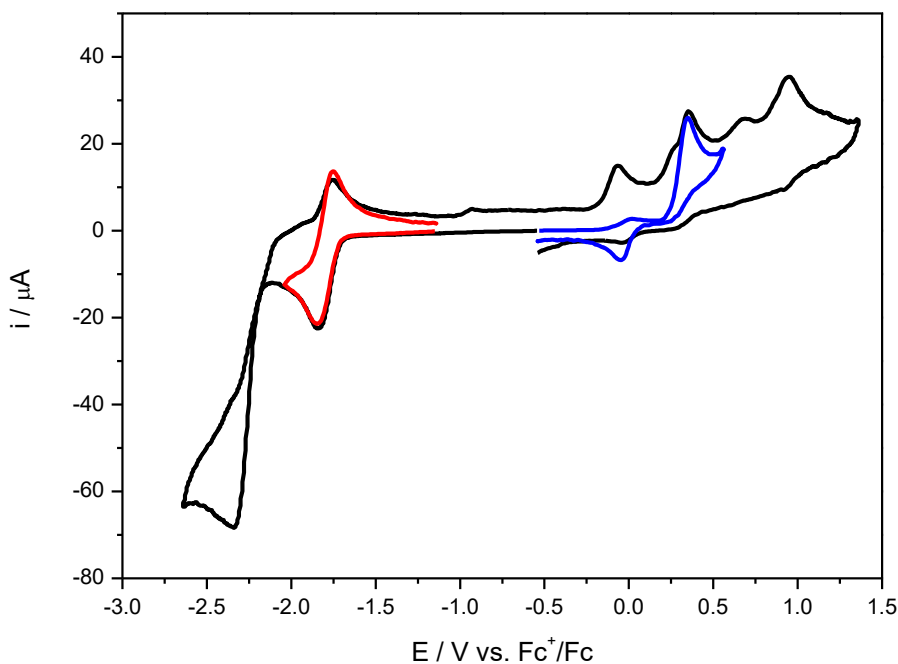
Figure IV.13. CV of complex 5 at a GC working electrode in MeCN/NBu 4 PF 6 0.1 M under Ar. Conditions: 1mM of complex, 0.1 V s -1 .
