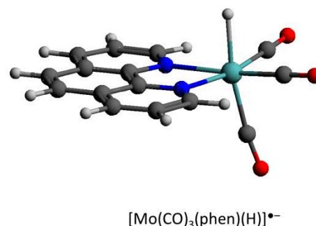
Figure 7. Calculated structure of [\text{Mo}(\text{CO})_3(\text{phen})(\text{H})]^{*-} . Atom colors: H (white), C (grey), N (blue), O (red) and Mo (green).
