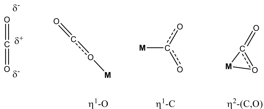
Figure I.13. Schematic representation of the \text{CO}_2 molecule and most common coordination modes with a metal center M.
