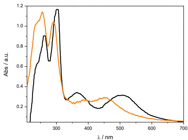
Figure II.4. UV-vis absorption spectra of 1 H (orange) and 1 CO 2 Me (black) in MeCN.
