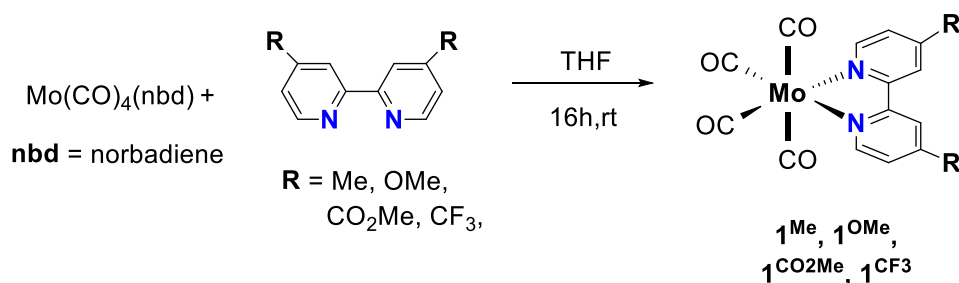
Scheme II.2. Synthetic pathway for 1 Me , 1 OMe , 1 CO 2 Me and 1 CF 3 complexes.
