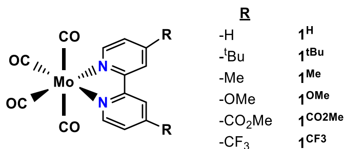
Figure I.31. General structure of [\text{Mo}(\text{CO})_4(\text{bpy}-(\text{R})_2)] derivatives.
