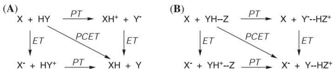
Figure I.18. Schematic representation of PCET (A) and concerted PCET (B) pathways. Reproduced from Ref. [64].
