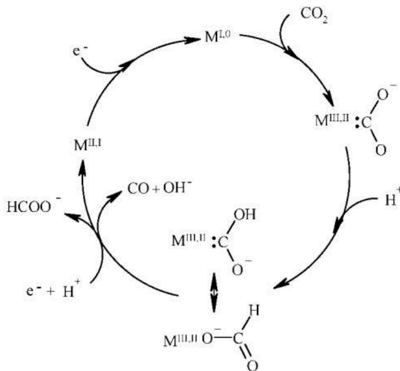
Figure I.16. General mechanism of formate formation by mediation of a transition metal system as a catalyst in a molecular CO 2 electroreduction reaction. Reproduced from Ref. [44].
