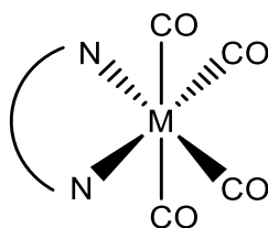
Figure I.24. General structure of [M(CO)_4(\text{diimine})] systems.
