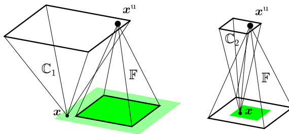
Figure 5.11.: Conic observation subsets with large ( \mathbb{C}_1 ) and small ( \mathbb{C}_2 ) aperture and resulting locations \mathbf{x} on the ground plane (green) that are observed from a point of view \mathbf{x}_{i,k}^u belonging to \mathbb{C}_1(\mathbf{x}) or \mathbb{C}_2(\mathbf{x}) .
