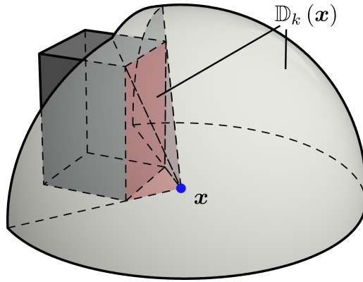
Figure 3.4.: Detectability set \mathbb{D}_k(\mathbf{x}) \subset \mathbb{R}^3 (red and gray) for a point \mathbf{x} \in \mathbb{X}_k^T (blue) located close to a box-shaped.
