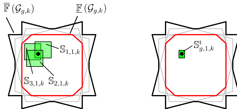
Figure 5.10.: Set estimate \mathbb{S}_{i,1,k} processed by different UAVs i \in \{1, 2, 3\} of group g (left) and resulting group estimate \mathbb{S}_{g,1,k}^t for target j = 1 (right).
