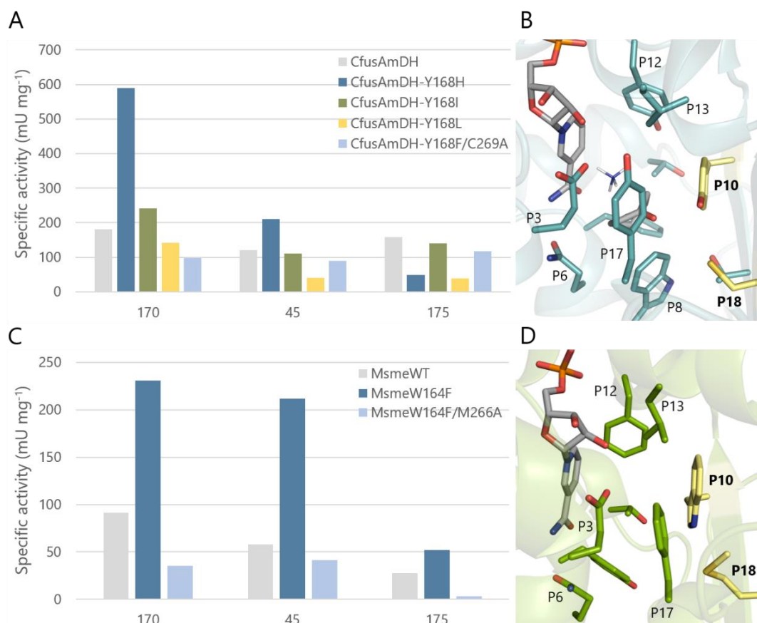
Figure 29. Influence of additional mutations at P10 in CfusAmDH and double mutations at P10 and P18 in CfusAmDH and MsmAmDH . (A)-(C) Specific activity (mU mg -1 ) of CfusAmDH and MsmAmDH P10- and P18-variants, respectively. The reaction conditions were as follows: final volume 100 \mu L, 10 mM carbonyl substrate, 1 M \text{NH}_4\text{HCO}_2 buffer pH 8.5-8.8, 0.2 mM NAD(P)H, 0.02-0.3 mg mL -1 purified enzyme, RT. (B)-(D) P10 and P18 highlighting (yellow) in CfusAmDH and MsmAmDH , respectively. CfusAmDH and MsmAmDH active sites with P10 and P18 highlighted in yellow.
