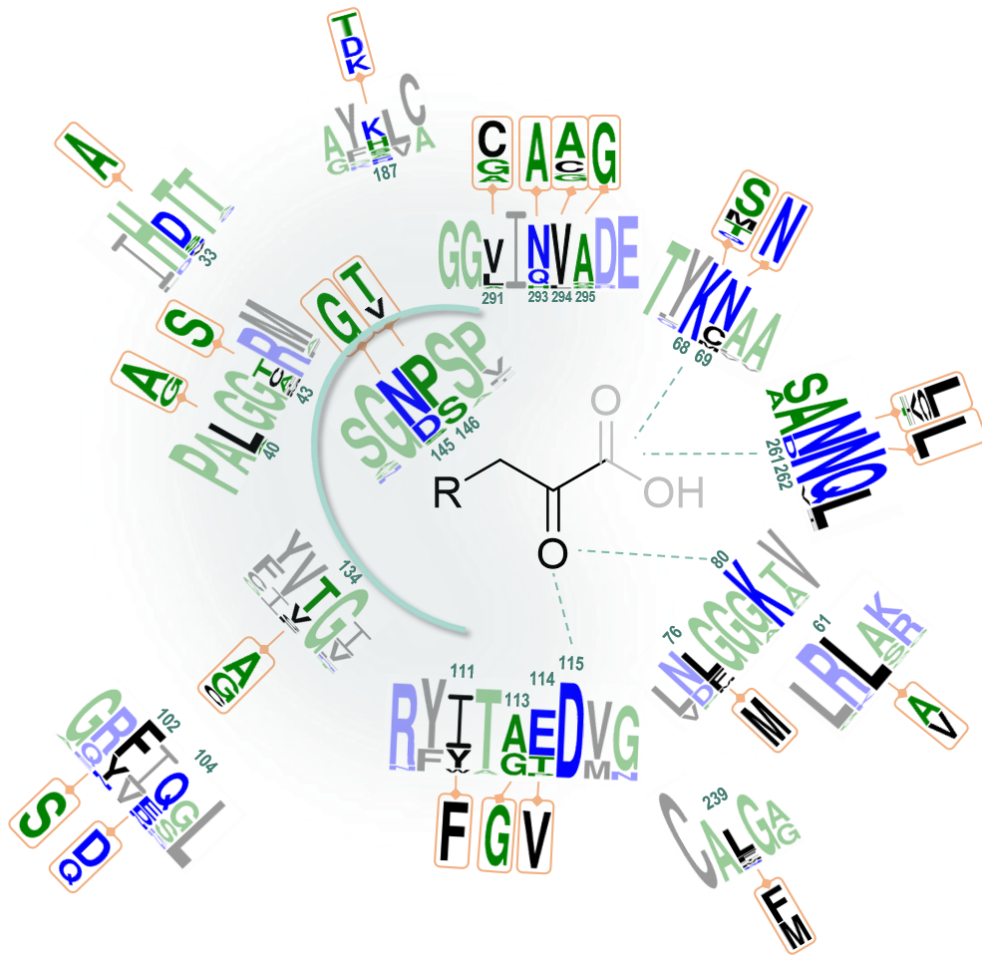
Figure 11. Logo representation of the mutational work done on LeuDHs and PheDHs. This representation shows the conservation patterns of all the residues targeted for mutation in the different studies focusing on engineered AADHs. The two residues described as essential for the catalytic mechanism (K80 and D115) are also indicated. The two neighboring residues located before and after the key residues in the protein sequence are also included to illustrate their environment. The sequence numbering used is that of LeuDH from Bacillus stearothermophilus . The logo of the variants produced for each of them are highlighted in orange. The color code is based on hydrophobicity (low hydrophobicity: blue, middle hydrophobicity: green, high hydrophobicity: black). Logo was generated using the webservice WebLogo3. Adapted from Ducrot et al. , 2020.
