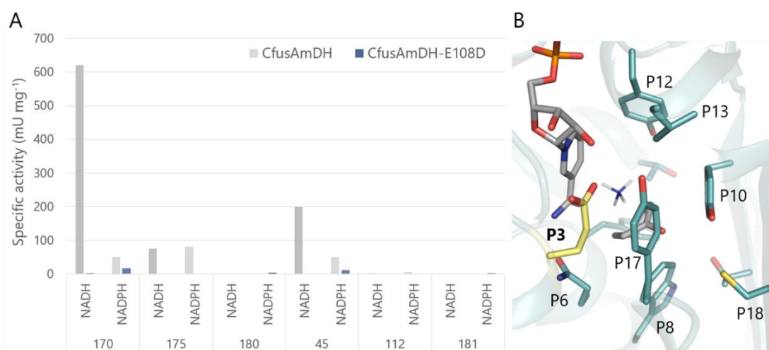
Figure 25. Influence of mutations at P3 in CfusAmDH . (A) Specific activity (mU mg -1 ) of CfusAmDH and its P3 variant. The reaction conditions were as follows: final volume 100 \mu L, 10 mM carbonyl substrate, 1 M NH 4 HCO 2 buffer pH 8.5, 0.2 mM NADPH or NADH, 0.03-0.15 mg mL -1 purified enzyme, room temperature (RT). (B) CfusAmDH active site with P3 highlighted in yellow.
