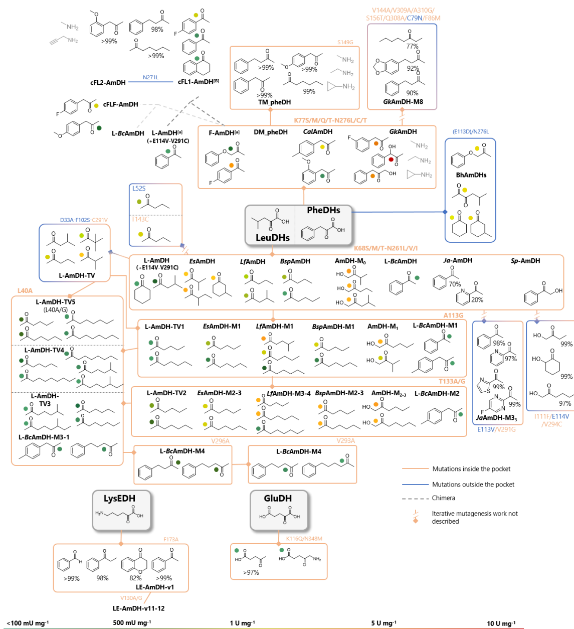
Figure 12. Substrate specificity of all the engineered AADHs and \epsilon -deaminating L-lysine dehydrogenase described in this part. The substrates associated to each variant were selected as the ones displaying the highest activities or considered as “new” substrates compared to the substrate scope of the whole family. Carbonyl and amine substrates are drawn in black and grey, respectively. If not mentioned, the amine substrate is ammonia ( 11 ). The orange and blue lines correspond to a set of mutations respectively inside or outside the catalytic pocket. The grey dashed lines correspond to the creation of a chimera from two parental enzymes. The specific activities indicated in this Figure are given as information but not to be compared as all the assays were not done with the exact same conditions. The following ones correspond to a range of typical conditions: 10–80 mM carbonyl substrate, 0.1–0.2 mM NAD(P)H cofactor, 1–6 M ammonium-based buffer pH 8.5–9.6, 25–30°C. In the case of enzymes without activity data, the substrates showing the highest conversion rates for one experimental condition were selected. For the sake of clarity, the numbering of the molecules is not indicated. [a] Activity assays done with lower 11 concentrations 0.225–0.5 M that could not allow to reach the saturation of 11 . [b] Activity assays done at 60°C, conversion tests at 30°C. The mutations written in bold correspond to the L-AmDH or F-AmDH numbering while the other mutations refer to the numbering of the targeted enzymes.
