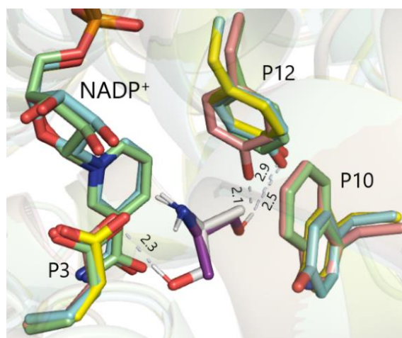
Figure 34. Docking of ( 2S )-1-hydroxypropan-2-amine ( 196 ) and ( 2R )-1-hydroxypropan-2-amine ( 197 ) in Micro AmDH and alignment with Cfus AmDH, Msm eAmDH and MATOUAmDH2. Structural alignment of Cfus AmDH RX structure (PDB: 6IAU; blue), Micro AmDH homology model (PDB template: 6IAQ; pink) and MATOUAmDH2 homology model (PDB template: 6IAU; yellow) to Msm eAmDH RX structure (PDB: 6IAQ; green). The corresponding NADP + cofactors are shown in the same color as the enzyme to which it belongs. Docked structures of 196 and 197 in Micro AmDH are respectively shown in white and purple. The distance between the H-atom of the hydroxyl group of 196 and the O-atom of the carboxylate group of E104 (P3) in Micro AmDH, and between the H-atom of the hydroxyl group of 197 and the O-atom of the hydroxyl group of Y169, Y173 and Y176 (P11), respectively of Micro AmDH, Cfus AmDH and MATOUAmDH2, are given in Angstroms (Å). RMSD ( Cfus AmDH- Msm eAmDH) = 0.987 Å; RMSD ( Micro AmDH- Msm eAmDH) = 0.254 Å; RMSD (MATOUAmDH2- Msm eAmDH) = 0.984 Å. Adapted from Ducrot et al. 2021.
