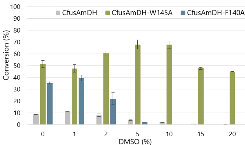
Figure 40. Conversion rates obtained from heptanal ( 217 ) with CfusAmDH , CfusAmDH-F140A and CfusAmDH-W145A with various ratios of DMSO. Conversion rate obtained for CfusAmDH , CfusAmDH-F140A and CfusAmDH-W145A reported in this paper towards heptanal ( 217 ). Reaction conditions: final volume 100 \mu L, 10 mM 217 (final ratio of DMSO 1-20%), 2 M \text{NH}_4\text{HCO}_2 buffer, pH 8.5, 0.2 mM \text{NAD(P)}^+ , 1.2 eq. 222 , 3 U \text{mL}^{-1} GDH-105, 0.5 mg \text{mL}^{-1} purified enzyme, 25°C, 24 h, 400 rpm. The temperature was set at 25°C after a preliminary study that displayed lower conversions at 30°C (Appendix 21). The monitoring of heptan-1-amine ( 213 ) was performed by UHPLC-UV after derivatization with BzCl. Error bars represent standard deviations of two independent experiments.
