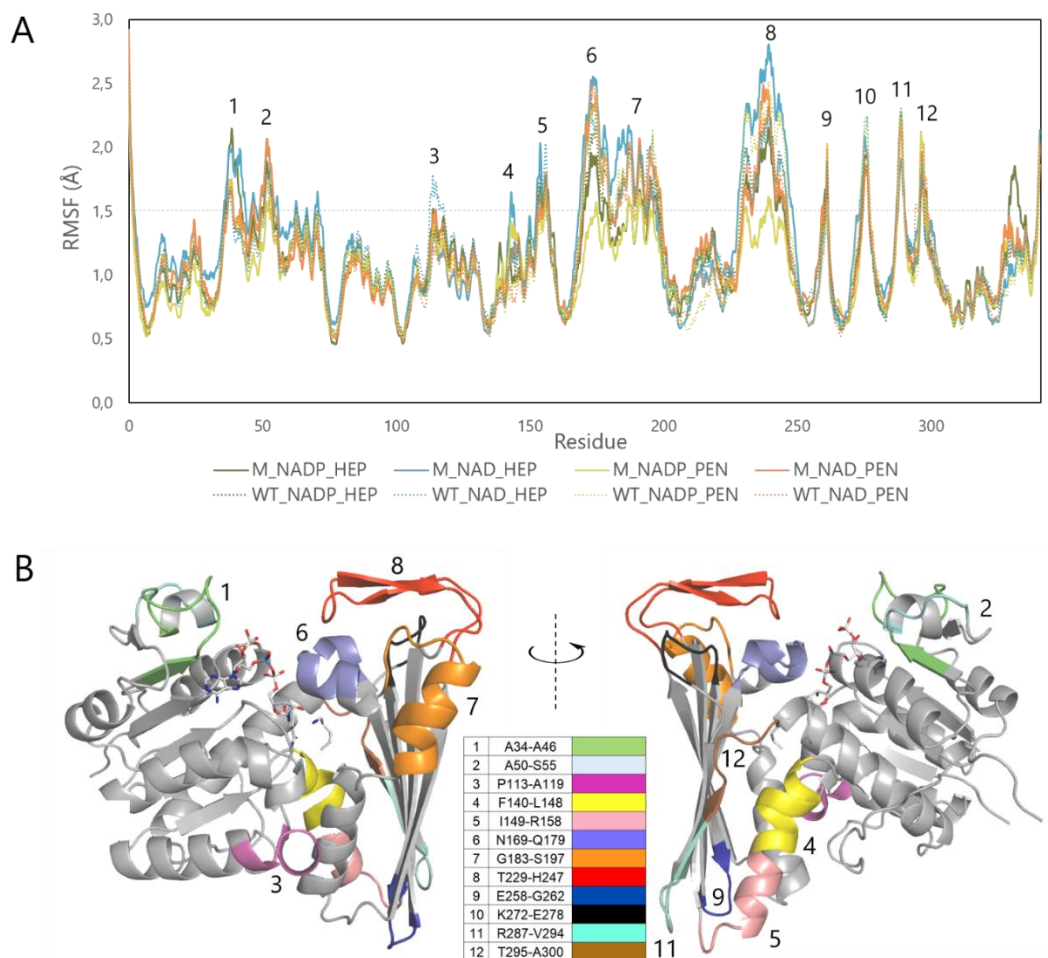
Figure 50. Cfus AmDH flexible sections. (A) RMSF analysis (B) 3D representation at 0° and 180° of WT monomer in complex with NAD and PEN. Segments 1-12 display a backbone fluctuation beyond 1.5 Å in RMSF analysis and are highlighted with a gradient of colors reported in the inserted table.
