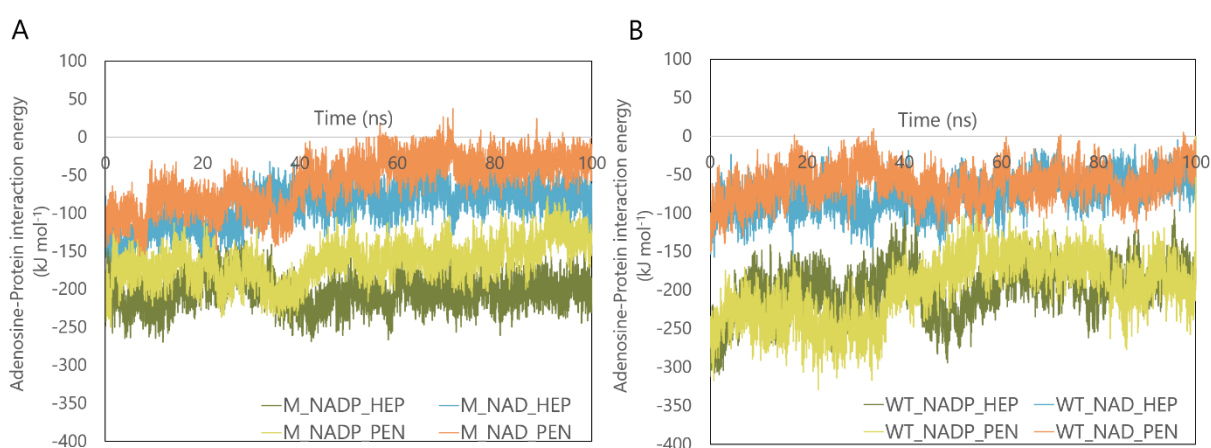
Figure 57. Interaction energies calculated between atoms of the adenosine moiety (C4B; C3B; C2B; O4B; C1B; O2B; N9A; N9A; N7A; C4A; C5A; N3A; C2A; N1A; C6A; N6A; O3B; ± P2B; ± O1X; ± O2X; ± O3X) and (A) M and (B) WT. These energies, given in kJ mol -1 , were calculated by addition of short-range Coulombic and Lennard-Jones interaction energies.
