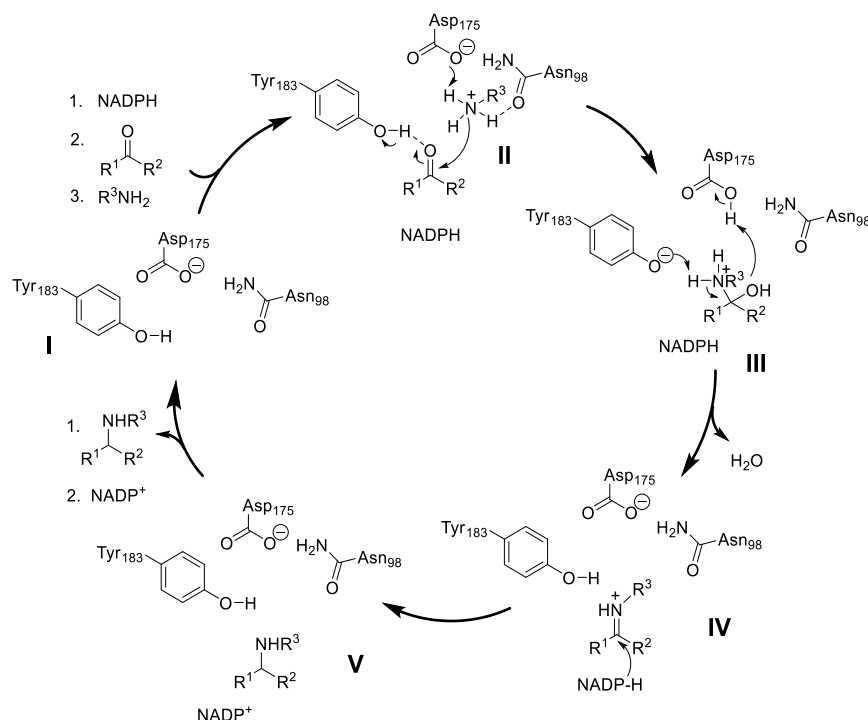
Scheme 11. Mechanism proposed for the fungal RedAm-catalyzed reductive amination of a ketone by small amines. Residue numbers correspond to those of AtRedAm . Extracted from Ducrot et al. , 2020, adapted from Sharma et al. , 2018.
