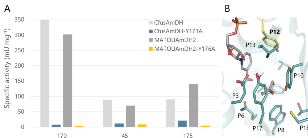
Figure 26. Influence of mutations at P12 in Cfus AmDH and MATOUAmDH2. (A) Specific activity ( \text{mU mg}^{-1} ) of Cfus AmDH, MATOUAmDH2 and P12 variants. The reaction conditions were as follows: final volume 100 \mu\text{L} , 10 \text{ mM} carbonyl substrate, 1 \text{ M} \text{NH}_4\text{HCO}_2 buffer pH 8.5, 0.1 \text{ mM} NADPH, 0.1 \text{ mM} NADH, 0.05\text{-}0.22 \text{ mg mL}^{-1} purified enzyme, RT. (B) Cfus AmDH active site with P12 highlighted in yellow.
