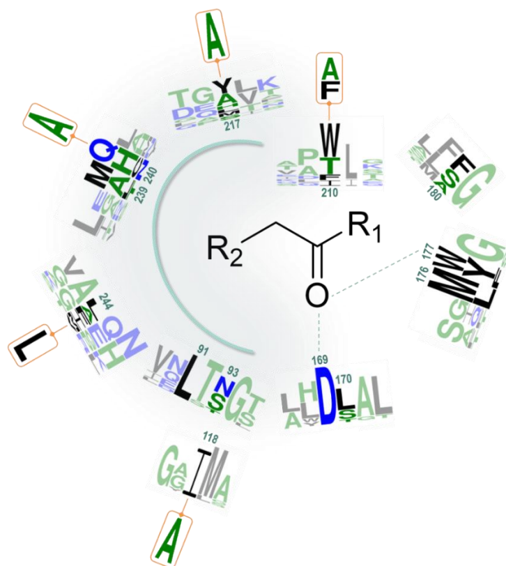
Figure 6. Logo representation of summary of key residues and mutation work done on selected IREDs with reductive aminase activity i.e. the ability to catalyze secondary amine formation from equimolar or low eq. of ketone and amine. This representation gives the conservation patterns of main residues of these enzymes defining the catalytic pocket and targeted for mutations inside or outside the active site. The two neighboring residues before and after these residues are included as part of the logos to illustrate their environment. The logo of the variants produced for extending substrate scope are placed above the corresponding WT residue and are highlighted in orange. Mutated residues of the variants M1-M3 of GSK_IR46 used by Schober et al. have not been included for clarity. The sequence numbering used is that of AspRedAm . The color code is based on hydrophobicity (low hydrophobicity: blue, middle hydrophobicity: green, high hydrophobicity: black). Logos were generated using the webservice WebLogo3. Extracted from Ducrot et al. , 2020.
