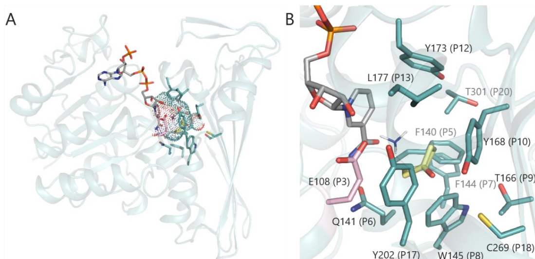
Figure 15. Global structure and active site of CfusAmDH . (A) Structure of CfusAmDH (PDB: 6IAU), the volume of the active site is represented with the dot surface of the residues constituting the first layer of the pocket (B) Active site of CfusAmDH with a focus on the P1-P21 positions (blue), shown in cylinder format, defining the cavity with NADPH (grey), 45 (yellow) and 11 . The catalytic residue E108 (P3) is highlighted in pink. For clarity, P1-2-4-11-14-15-16-19-21 are omitted. P1-P21 numbering explanations are given later on in this paragraph.
