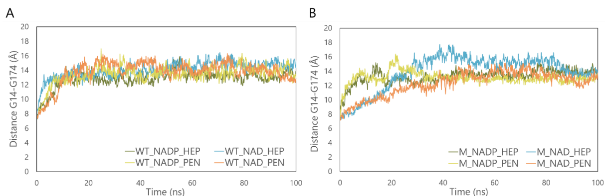
Figure 51. Evolution of G14-G174 distance (Å) as a function of time (ns) (A) WT in complex with NAD + (NAD) or NADP + (NADP) and PEN or HEP (B) Same curves with M. The curves are averaged onto four independent simulations starting with a random velocity seed.
