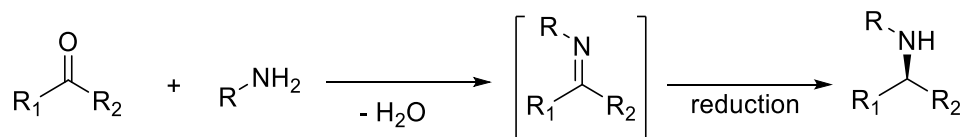
Scheme 2. Reductive amination reaction.
