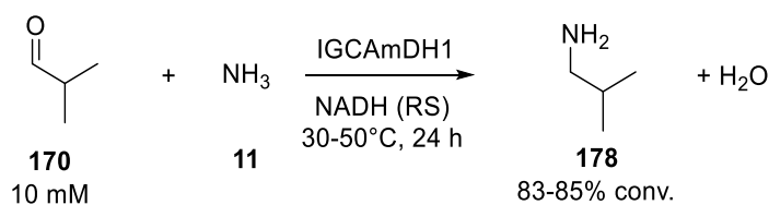
Scheme 28. Example of reductive amination reaction catalyzed by IGCAmDH1 obtained from metagenomic data. RS = recycling system.
