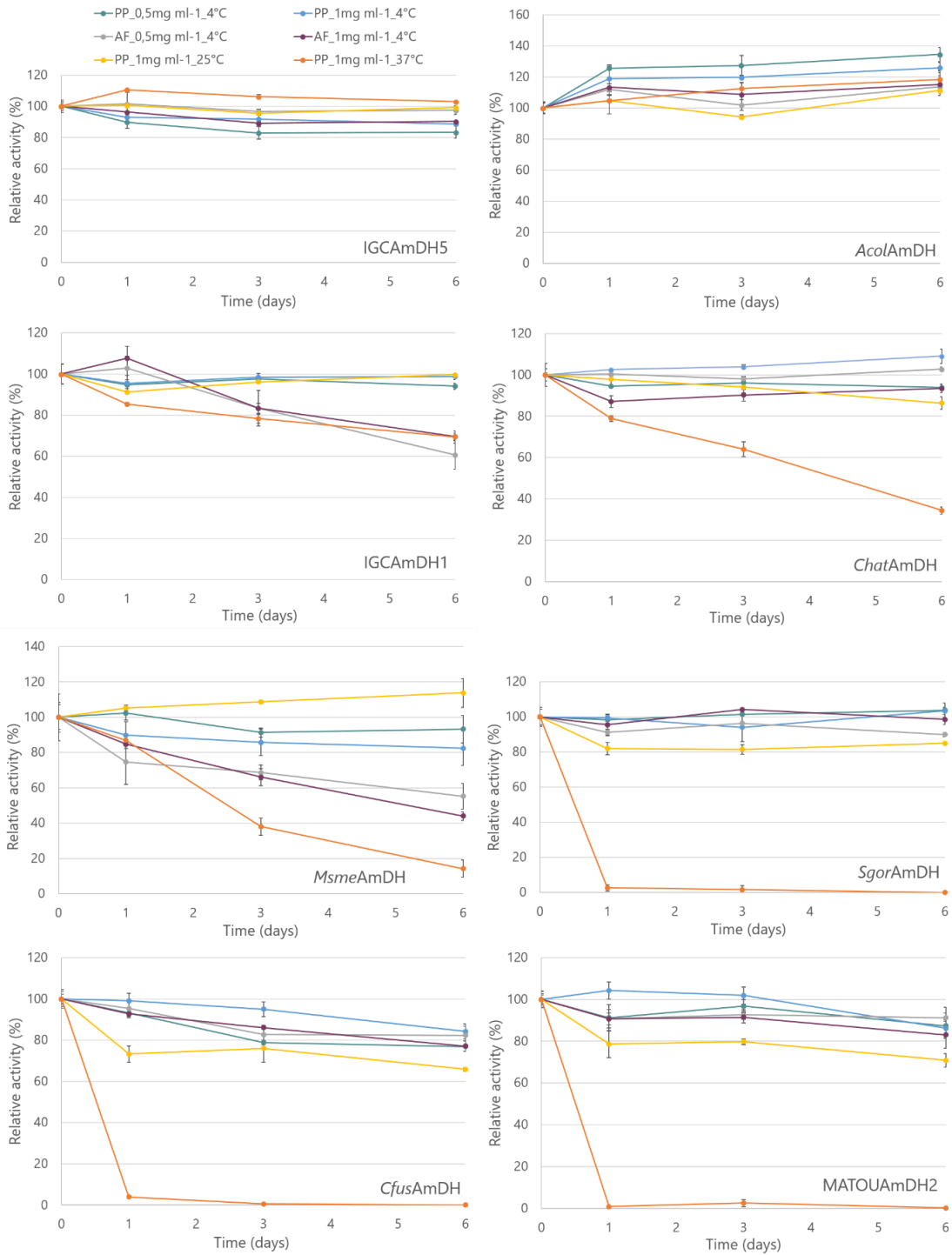
Figure 30. Relative remaining activity of IGCAmDH5, AcolAmDH , IGCAmDH1, ChatAmDH , MsmeAmDH , SgorAmDH , CfusAmDH and MATOUAmDH2 towards 170 after different storage conditions. 100% alludes to the enzyme specific activity measured the day of the purification (IGCAmDH5: 619.0-661.2 mU mg -1 ; AcolAmDH : 219.0-274.3 mU mg -1 ; IGCAmDH1 349.7-525.5 mU mg -1 ; ChatAmDH : 801.5-858.0 mU mg -1 ; MsmeAmDH : 59.0-147.2 mU mg -1 ; SgorAmDH : 790.0-986.7 mU mg -1 ; CfusAmDH : 3.6-3.8 U mg -1 ; MATOUAmDH2: 3.4-4.0 U mg -1 ). Reaction conditions were as follows: final volume 100 \mu L, 10 mM 170 , 2 M NH 4 HCO 2 buffer pH 8.5, 0.2 mM NADH (NADPH for MATOUAmDH2), 0.001-0.12 mg mL -1 purified enzyme, 40°C. Errors represent standard deviations of two independent experiments with two different enzymes aliquots stored in the same conditions. PP = potassium phosphate buffer; AF = ammonium formate buffer.
