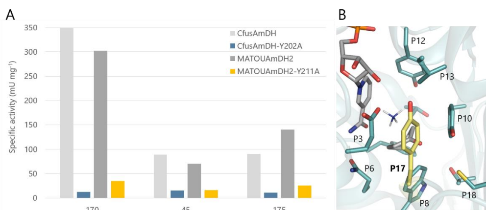
Figure 27. Influence of mutations at P17 in CfusAmDH and MATOUAmDH2. (A) Specific activity (mU mg -1 ) of CfusAmDH and MATOUAmDH2 P17-variants. The reaction conditions were as follows: final volume 100 \mu L, 10 mM carbonyl substrate, 1 M NH 4 HCO 2 buffer pH 8.5, 0.1 mM NADPH, 0.1 mM NADH, 0.05-0.22 mg mL -1 purified enzyme, RT. (B) CfusAmDH active site with P17 highlighted in yellow.
