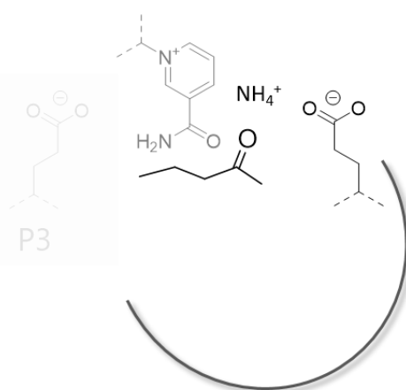
Scheme 34. Schematic view of a catalytic glutamate located on the opposite side of P3 in the active site. As an example, pentan-2-one ( 112 ), ammonia ( 11 ) and a part of the nicotinamide cofactor are also represented.
