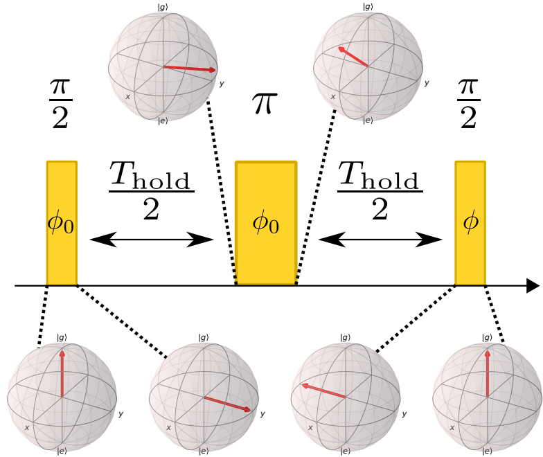
Figure 3.8 – Scheme of a Ramsey with spin echo sequence. The internal state of the probed two levels is represented in the Bloch sphere picture (red arrow) before and after each laser pulse, here for \delta_E T_{\text{hold}} = \frac{\pi}{4} and \phi = 0 . Here the effect of the static dephasing has been canceled by the intermediate \pi pulse.
