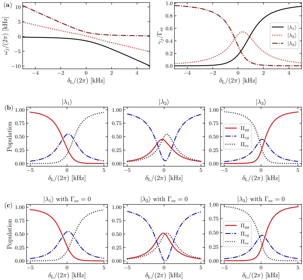
Figure 5.7 – Diagonalization of \hat{H}^{(2)} in the strong coupling limit. (a) Real ( left ) and imaginary ( right ) parts of the eigenvalues. (b) Bare state composition of each dressed state. (c) Bare state composition of each dressed state in absence of dissipation.
