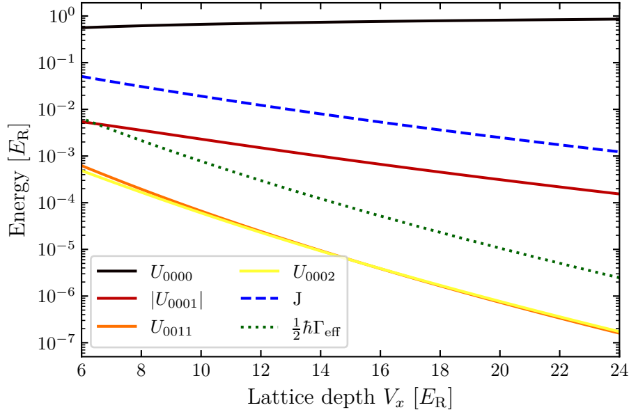
Figure 6.9 – Comparison between the first matrix elements of the extended Bose-Hubbard model, the tunneling energy and the effective loss rate for different depth of the 1D lattice, assuming V_{y,z} = \{25, 27\} E_R in the strong directions of the optical lattice.
