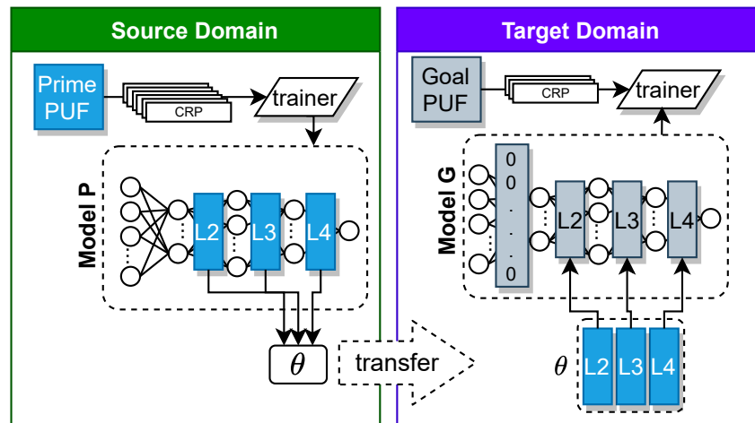
Figure 3.7: Our proposed Transfer Learning Plan, based on reusing the hidden layers of Mursi’s MLP model.
