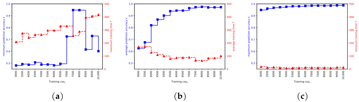
Figure 3.5: Illustration showing the minimum, average, and maximum training time T and prediction accuracy \epsilon for various csstr . (a) Max T and Min \epsilon ; (b) average T and \epsilon ; (c) Min T and Max \epsilon .
