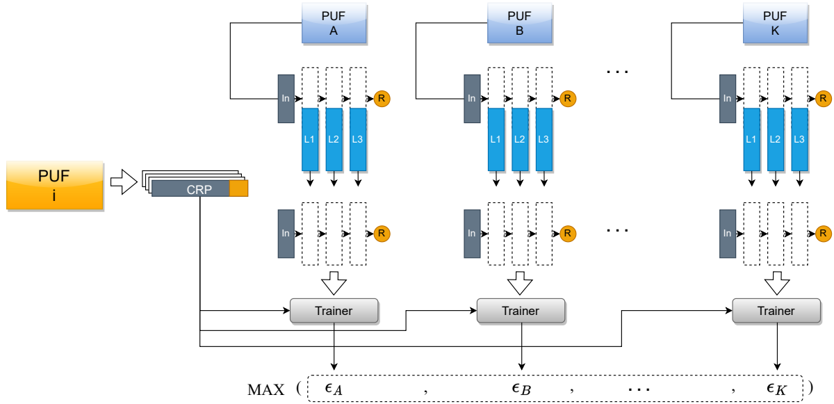
Figure 5.1: Illustration showing the schematic of bagging-enabled transfer learning solution for modeling PUF.
