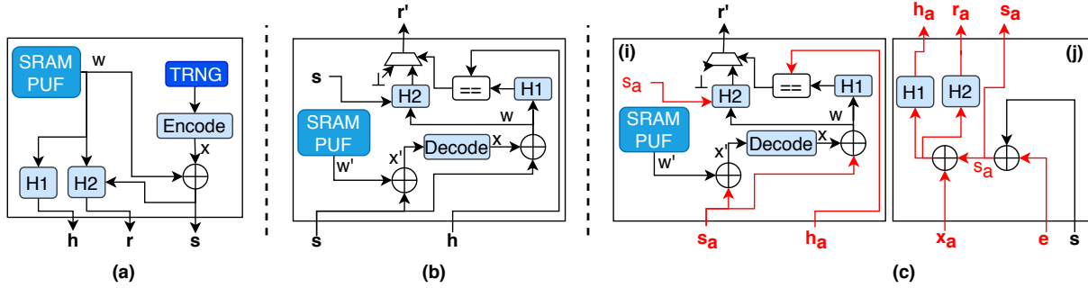
Figure 4.1: Illustration showing the RFE-like construction (a) the registration phase, (b) the recovery phase, and (c) the recovery phase with presence of HDMA, of the SRAM-PUF based encryption key generation.
