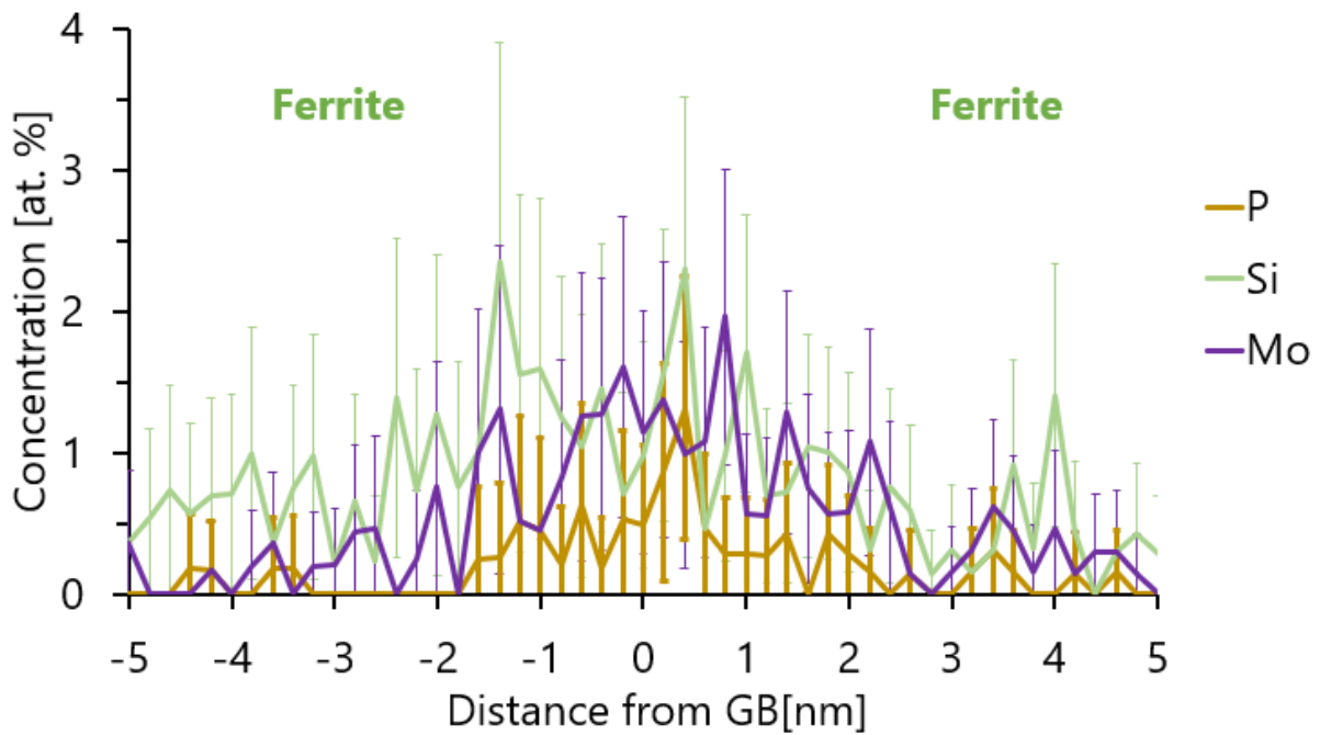
Figure 7. CT RPV steel F irradiated up to 0.06 dpa ( \phi t 4.09; E > 1\text{MeV} ). Concentration profile plotted through GB for P, Si and Mo atoms.
