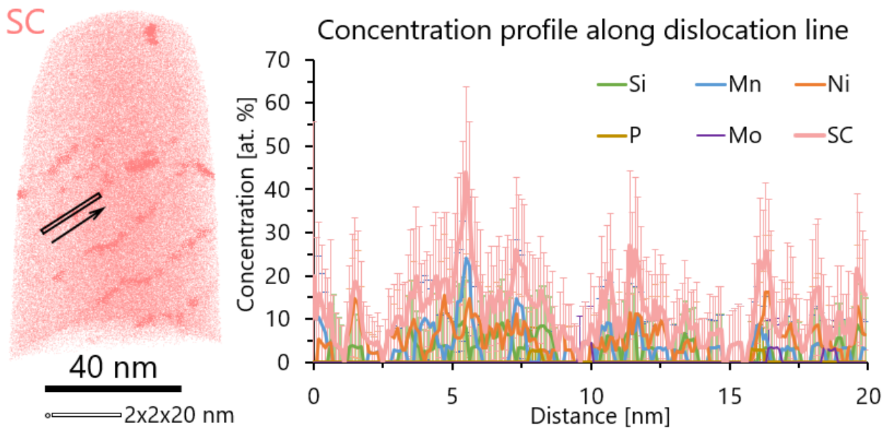
Figure 11. CT RPV steel N irradiated up to 0.075 dpa (qt 5.21; E > 1 MeV). Concentration profile plotted alongside the LAGB dislocation line for Si, Mn, Ni, P and Mo (and combined as SC) atoms.
