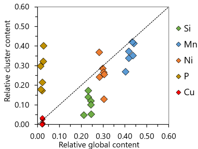
Figure 65. Relative cluster solute content as a function of relative global solute content in steel O irradiated up to 0.063 dpa (both values are given excluding all chemical species except Si, Mn, Ni, P and Cu and normalised to 1). Each diamond represents the results obtained in one APT experiment. 1:1 trend line is also plotted.
