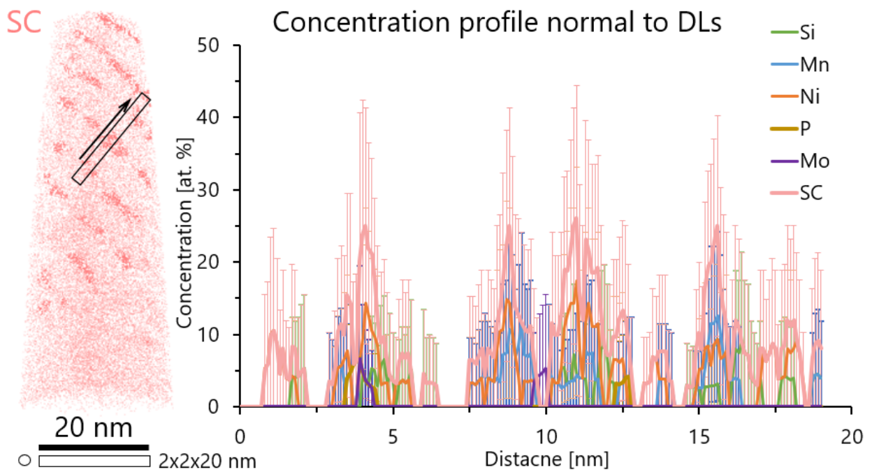
Figure 8. CT RPV steel I irradiated up to 0.08 dpa ( \phi t 5.72; E > 1\text{MeV} ). Concentration profile plotted normal to LAGB dislocation lines for Si, Mn, Ni, P and Mo (and combined as SC) atoms.
