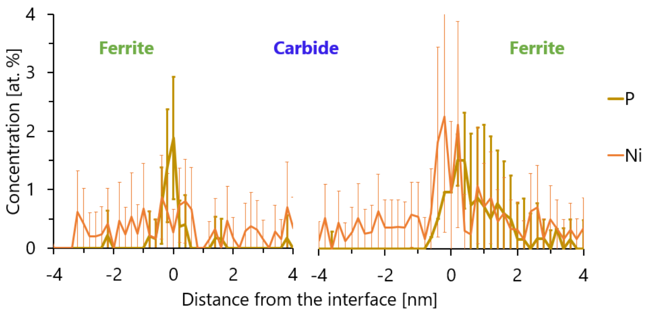
Figure 12. CT RPV steel O irradiated up to 0.063 dpa (qt 4.38; E > 1 MeV). Concentration profile plotted through ferrite / carbide interfaces for P and Ni atoms.
