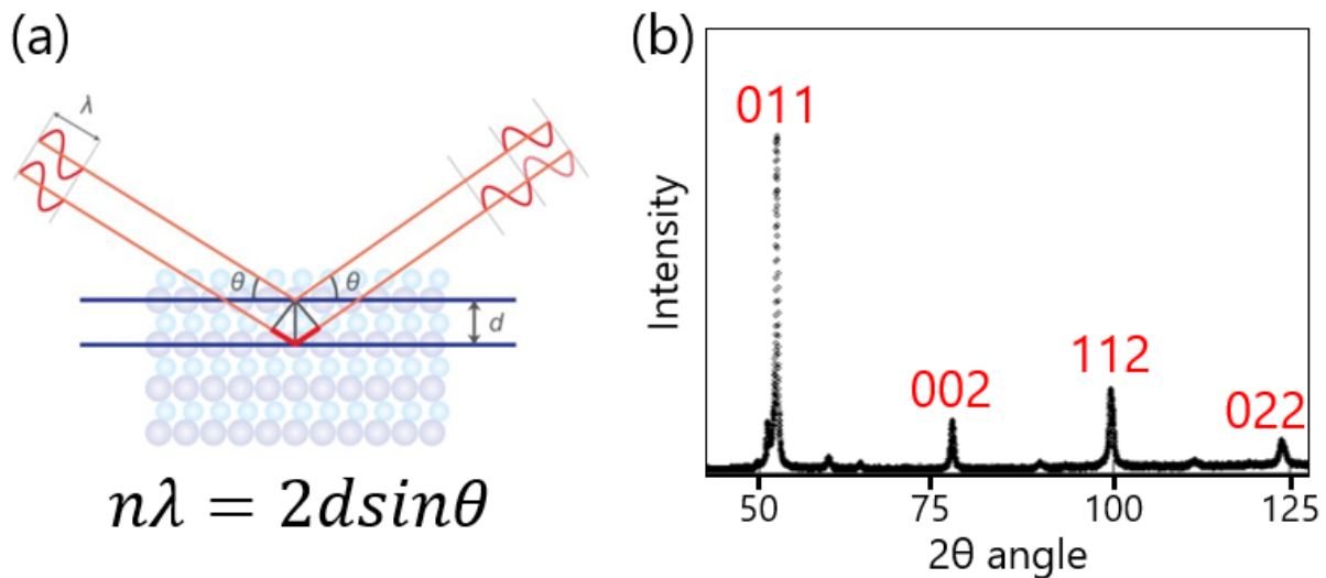
Figure 1. (a) Planes satisfying the Bragg's condition [2]. (b) Diffractogram of CT RPV steel I in the non-irradiated state.
