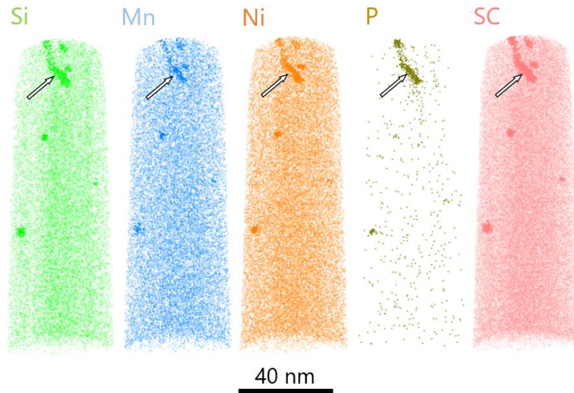
Figure 25. Atom maps of steel E irradiated up to 0.09 \text{ dpa} . Solute clusters enriched in Si, Mn, Ni and P are observed. Arrows indicate solute clusters on the dislocation line.
