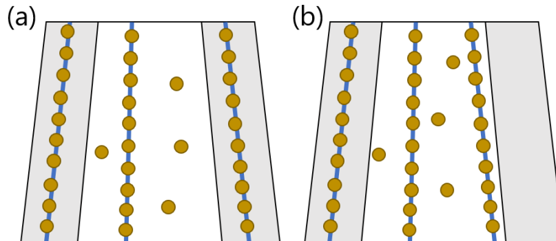
Figure 17. Possible distribution of P atoms between APT specimens. Grey areas are the initial APT specimen. White areas are the detected by APT volume. Blue lines represent [222] and [011] poles. (a) Volume where only one crystallographic pole is located inside the detected volume. Lower P concentration is measured. (b) Volume where two crystallographic poles are inside the detected volume. Higher P concentration is measured.
