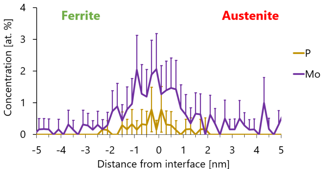
Figure 9. CT RPV steel I irradiated up to 0.08 dpa (pt 5.72; E > 1\text{MeV} ). Concentration profile plotted through ferrite / austenite interface for P and Mo atoms.
