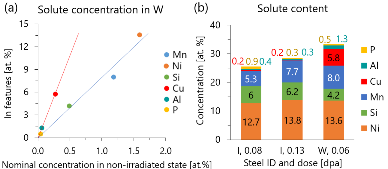
Figure 17. (a) Evolution of enriched feature solute concentrations as a function of nominal concentration in steel W. Red line is the trend for Cu atoms. Blue line is the trend for Mn, Ni and Si. (b) Solute concentrations of clusters and solute-enriched features observed in steels I and W irradiated from 0.06 to 0.13 dpa.
