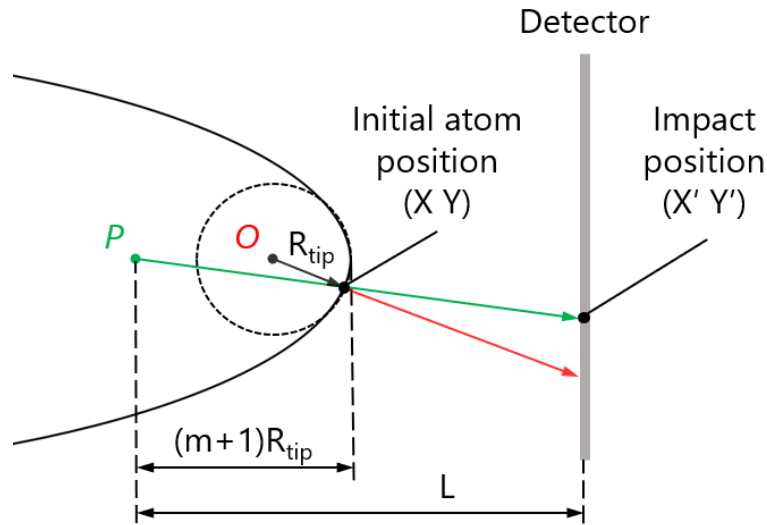
Figure 22. The schematic view of the point projection model. O is the centre of the hemisphere cap. P is the projection point. The initial atom position (X, Y) is identified from the impact point (X', Y') with the point projection model.
