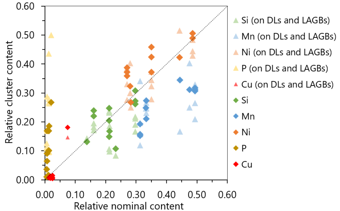
Figure 26. Evolution of relative cluster solute content as a function of relative nominal solute content (both values given excluding Fe, impurities and normalised to 1). Pale triangles represent clusters observed on dislocation lines and low-angle GBs. Diamonds represent cluster formed in ferrite matrix. 1:1 trend line is also plotted.
