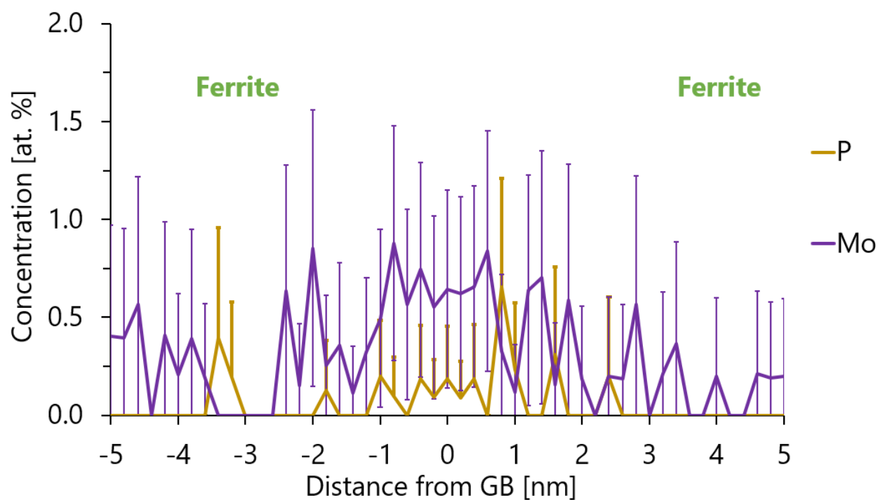
Figure 10. CT RPV steel I irradiated up to 0.13 dpa (pt 9.14; E > 1\text{MeV} ). Concentration profile plotted through GB for P and Mo atoms.
