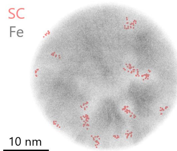
Figure 31. Artefact Mn-Ni-Si-P cluster identified alongside the poles and zone lines in the non-irradiated steel O. C_{th} = 6.6 \% , N_{min} = 8 SC atoms. The low Fe density at poles and zone lines is evident.
