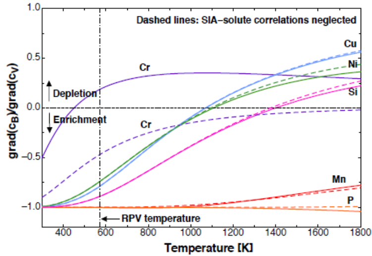
Figure 10. Radiation-induced segregation profiles as a function of irradiation temperature. Solute enrichment on sinks occurs for negative values [22].
