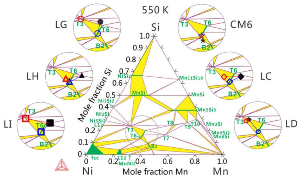
Figure 14. Ternary phase diagram of Mn-Ni-Si system at 277 °C. Filled symbols represent the APT composition of MNSFs from experimental data on six RPV steels with different chemical compositions. Open red and blue symbols are the predictions from commercial and homemade CALPHAD databases [35,98,99].
