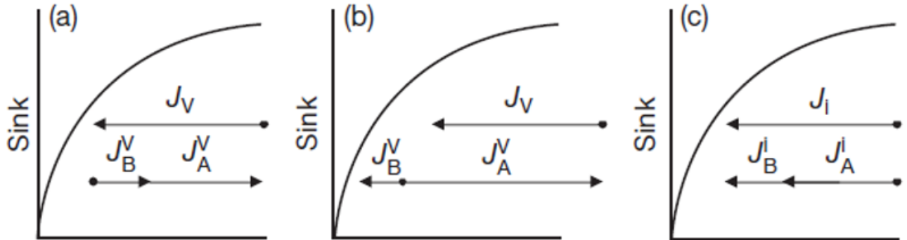
Figure 6. Irradiation-induced segregation in a binary A-B alloy. (a) Fluxes of A and B solute atoms are in the opposite direction of vacancy flux. A atoms diffusing faster than B ones will result in the depletion of A and enrichment of B at sink. (b) Vacancies and B atoms are attracted. Vacancies flux will create the enrichment of B and depletion of A at the sink. (c) Both A and B atoms are transported by SIA towards the sink, enrichment in A and B elements will occur. Enrichment will depend on respective A and B nominal compositions [18].
