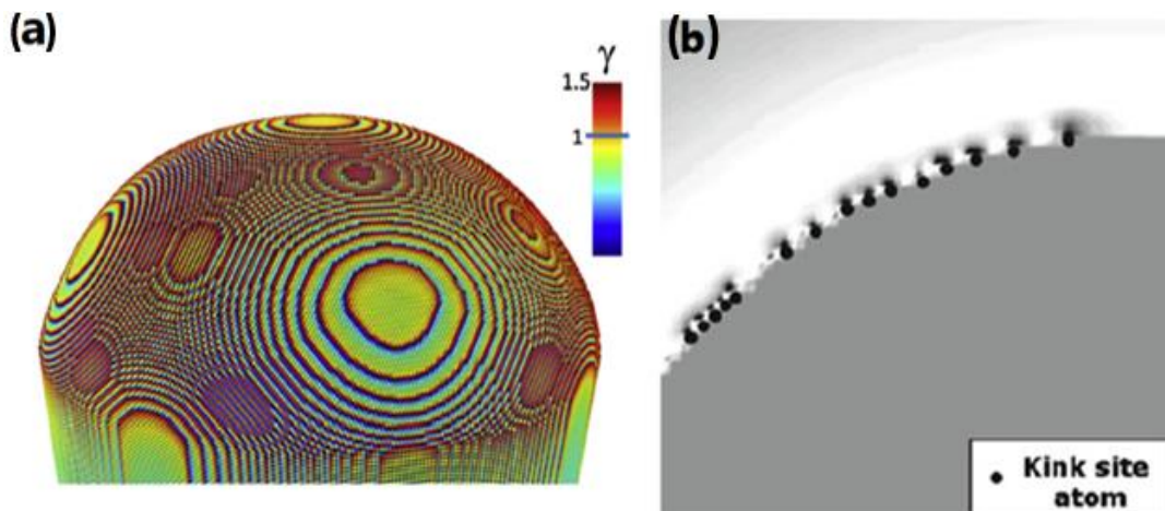
Figure 29. (a) Distribution of the surface enhancement factor. Maximum enhancement factor of 1.5 is found above the atoms on the edge position of the crystalline terraces. (b) A simulation of the electric field around the kink atoms around the apex of the tip. Dark regions represent the higher field above the kink atoms [38].
