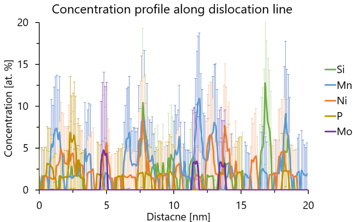
Figure 3. CT RPV steel E irradiated up to 0.07 dpa ( \phi t 4.78; E > 1\text{ MeV} ). Concentration profile plotted alongside the dislocation line for Si, Mn, Ni, P and Mo atoms.
