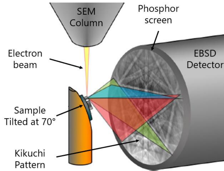
Figure 10. Schematic view of an EBSD experiment. The electrons backscattered for the specimen tilted at 70° are projected toward the phosphor screen of EBSD detector [19].
