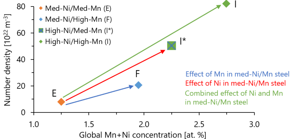
Figure 12. Evolution of cluster number density as a function of combined Mn+Ni concentrations in materials irradiated up to the high dose. Diamonds represent the average values for material where several APT experiments are performed. Crossed square symbol is the number density evaluated from one APT experiment on I* where lower than expected global Mn concentration is measured.
