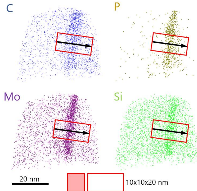
Figure 21. Atom maps of segregation on the GB in steel D. Enrichment in C, P, Mo and Si atoms is observed.
