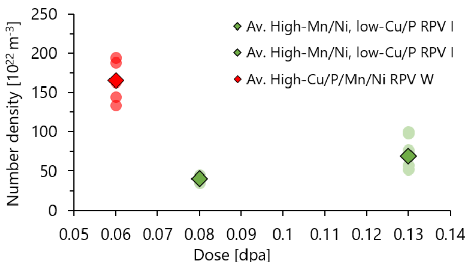
Figure 16. Evolution of cluster (I) and solute-enriched feature (W) number densities as a function of irradiation dose. Pale circles represent number density of clusters for each APT experiment. Diamonds represent the average values (pale circles can be hidden by diamonds symbols).
