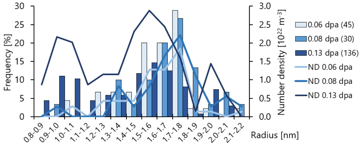
Figure 40. Size distribution for clusters formed inside ferritic matrix.
