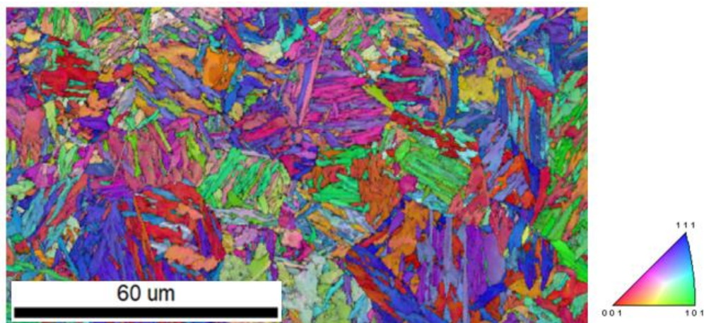
Figure 12. IPF orientation EBSD map of the CT RPV steel I.
