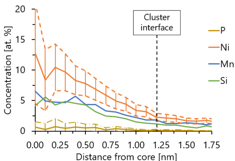
Figure 9. Erosion profile of clusters in I irradiated up to medium dose. Concentration of main solutes measured inside clusters is plotted. For visual simplicity, statistical uncertainty only for Ni and P atoms are plotted. The step size of the erosion profile is 0.1 nm, and only radial volumes containing more than 80 atoms were selected.
