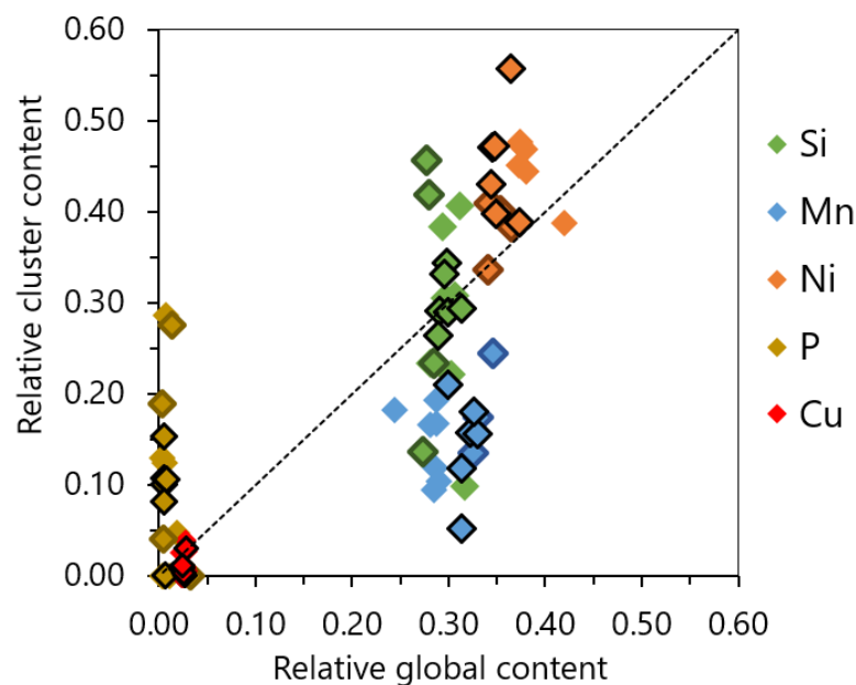
Figure 29. Evolution of relative cluster solute content as a function of relative global solute content in steel E. Each diamond represents the results obtained in one APT experiment. Low dose represented by symbols without borders, medium dose by symbols with darker border and high dose by symbols with black border. 1:1 trend line is also plotted.
