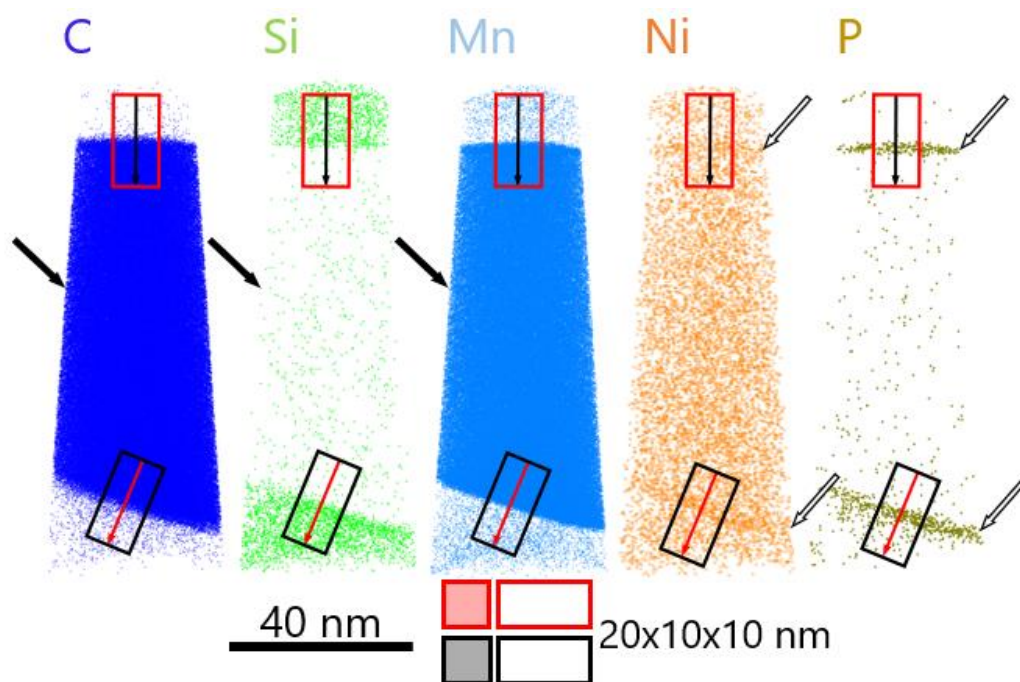
Figure 66. Atom maps of steel O irradiated up to 0.063 dpa. Black arrows indicate M_3C carbide enriched in C and Mn and depleted in Si. White arrows indicate ferrite / carbide interfaces.
