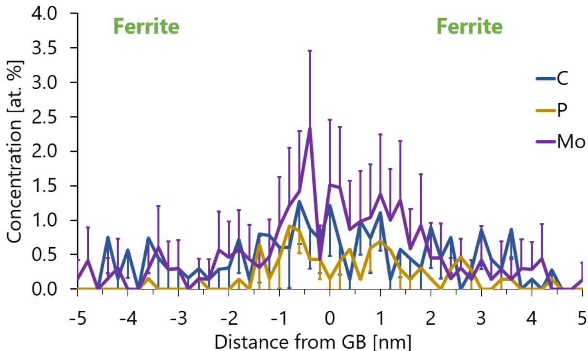
Figure 2. CT RPV steel D irradiated up to 0.09 dpa ( \phi t 6.29; E > 1\text{ MeV} ). Concentration profile plotted through GB for C, P and Mo atoms.
