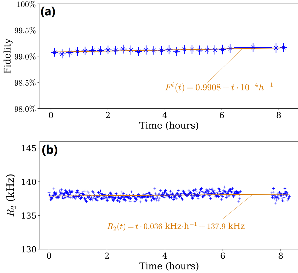
Fig. 3.19: Features of the source measured over an 8-hours time-span. The 1-hour gap at the end of the data series is due to a cooling cycle of the detectors. (a) Fidelity of the source's state to a Bell state. (b) Biphoton detection rate R_2 .
