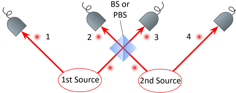
Fig. 3.20: Typical layout of a optical multipartite quantum experiment.
