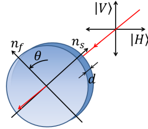
Fig. 2.5: Axes of a wave plate, relatively to |H\rangle and |V\rangle axes. The fast and slow axes are labeled by n_f and n_s respectively.
