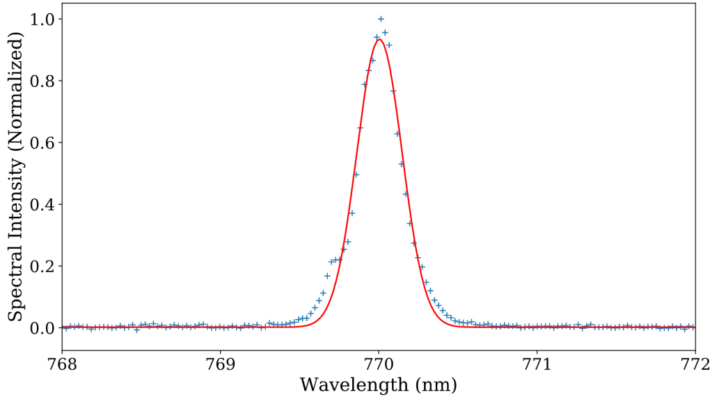
Fig. 3.6: Measured spectrum of the mode-locked pump Laser, with a Gaussian fit giving the 770nm central wavelength and 0.48nm FWHM.
