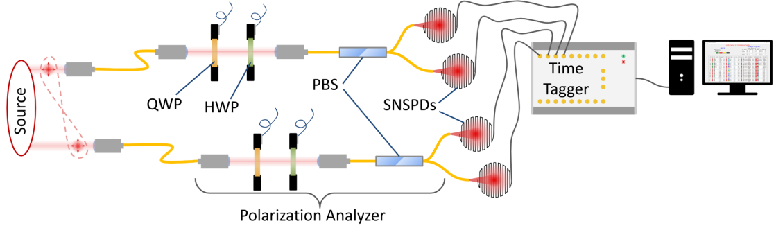
Fig. 3.15: Full apparatus used to analyze the bi-photon polarization state. Two polarization analyzers allow the local measurement of each photon of the pair. Correlations between detection events are then assessed by the time tagger and computer.
