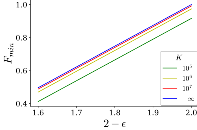
Fig. D.1: Minimum fidelity of the average output state to a Bell state, up to isometries, as a function of the deviation to maximum violation. As we make no IID assumption, we give the evolution for different numbers K of states measured. We set a confidence level 1 - e^{-x} \approx 0.999 .
