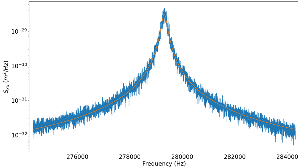
Fig. III.16 Noise displacement spectrum of the mechanical mode at room temperature and ambient pressure with 1.9 \mu\text{W} of input optical power (blue curve). The Lorentzian fit (orange curve) corresponds to a mechanical quality factor Q = 1360 and yields an effective mass of 134 \pm 3 \mu\text{g} .
