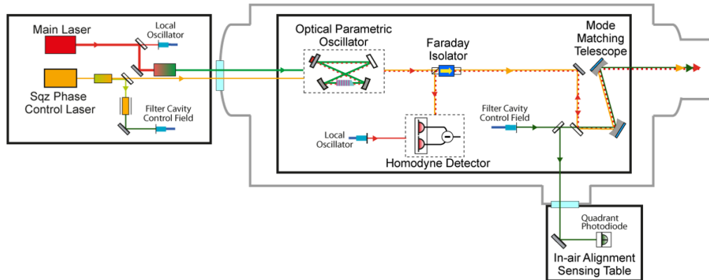
Fig. IV.34 Experimental setup. On the left is the in-air bench where we have the main laser, the two SHGs and the Mach-Zender interferometer (not represented here). Then, under vacuum, we have the OPO, the homodyne detector and the 50-m long rotation cavity. Maintaining the alignment of such a long cavity requires extra-control fields and a quadrant photodiode detection.
