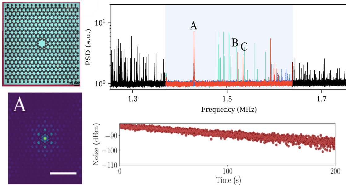
Fig. V.1 A phononic-crystal SiN membrane as a high-Q optomechanical system. Top Left: Optical view (false color) of a 2.5 \text{ mm} \times 2.5 \text{ mm} \times 100 \text{ nm} membrane, with a phononic crystal and a defect. Bottom: Simulated profile of the fundamental defect mode. Top right: Noise spectrum, with only a few localized modes of the defect present in the frequency gap of the phononic crystal. The mode A is the main mode of interest. Bottom right: Mechanical decay measurement of the Q of the fundamental mode of a non-patterned membrane. The Q value is here above 10^8 at \simeq 1 \text{ K} , which makes us optimistic we can reach 10^9 with a patterned membrane in a dilution fridge.
