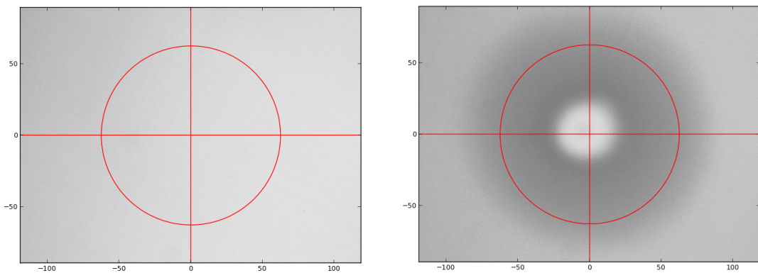
Fig. III.9 Interferometric profile of a Suprasil sample before and after a CO 2 laser shot of 90 ms. We have obtained a concave structure with a 60- \mu\text{m} diameter and a radius of curvature of 1.3 mm.
