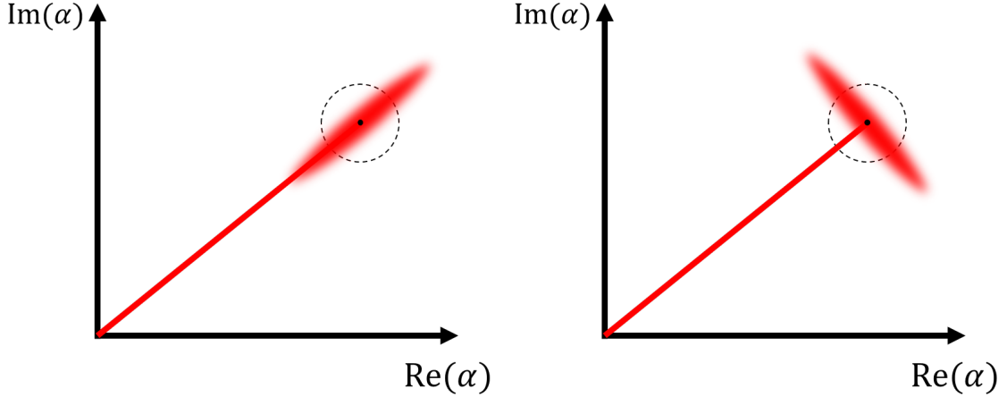
Fig. II.7 Phase squeezed state and amplitude squeezed state representation on the complex plane.
