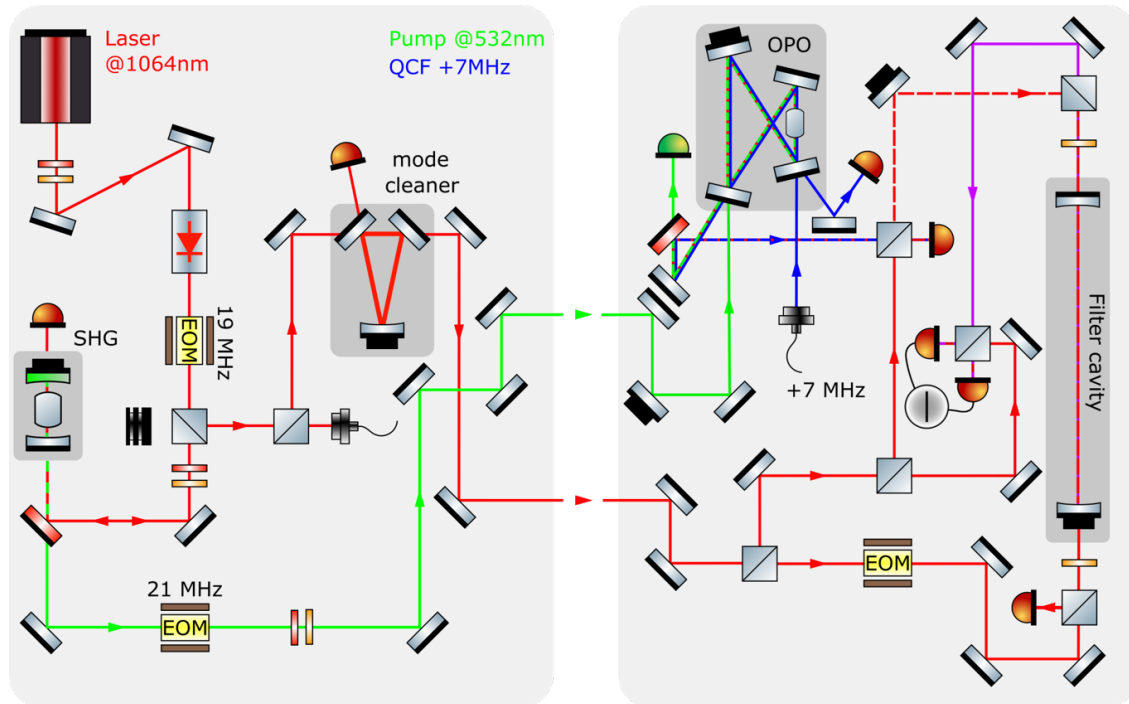
Fig. IV.22 Simplified optical setup with all the principal elements. EOM stands for Electro-Optic Modulator . Those are used to generate phase modulation for the PDH locks mentioned in section IV.7. The detuned coherent control field is represented in blue, the vacuum squeezed field is represented in dashed red and frequency dependent squeezing is represented in purple.
