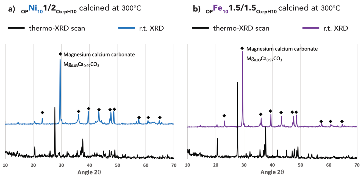
Figure 4.7: X-ray diffractograms of a) OPNi_{10}1/2_{Ox-pH10} , and b) OPFe_{10}1.5/1.5_{Ox-pH10} catalysts calcined at 300°C recorded at room temperature (r.t.) and compare to X-ray thermodiffractogram at 300°C of the corresponding precursors.
