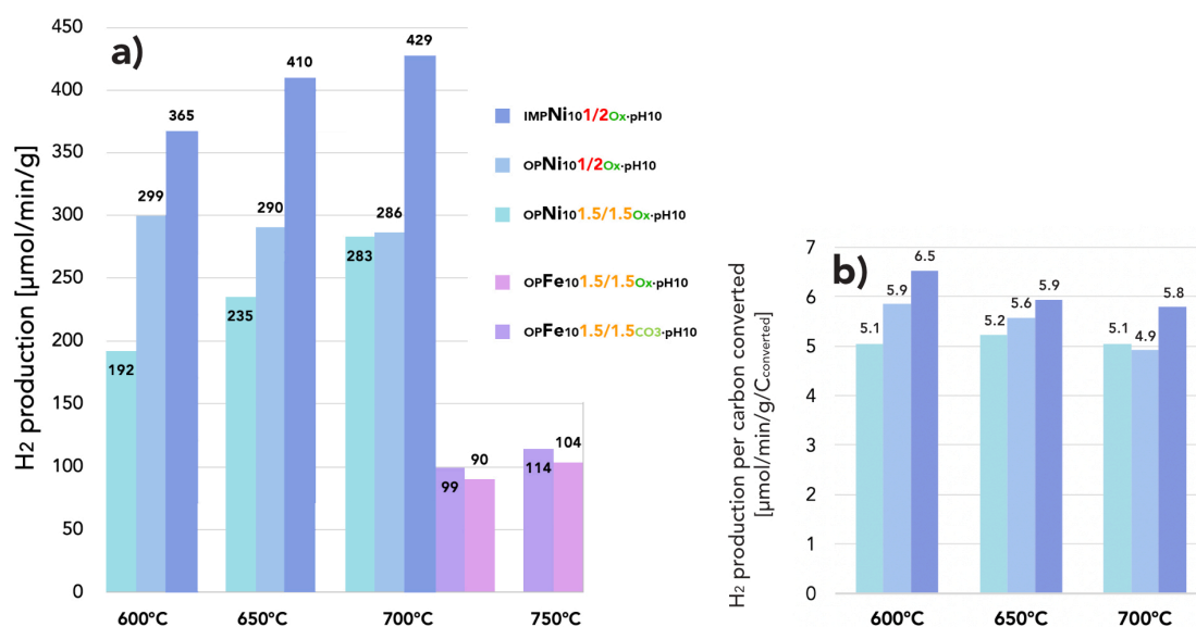
Figure 5.4: a) Productivity of H 2 according to temperature for selected nickel and iron catalysts at S/C ratio at 6, b) Productivity expressed per carbon converted.
