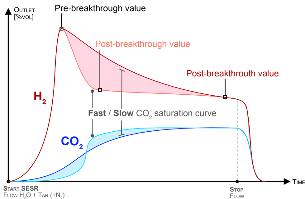
Figure 2.5: Pattern and method for catalytic SESR reactivity test measurement
