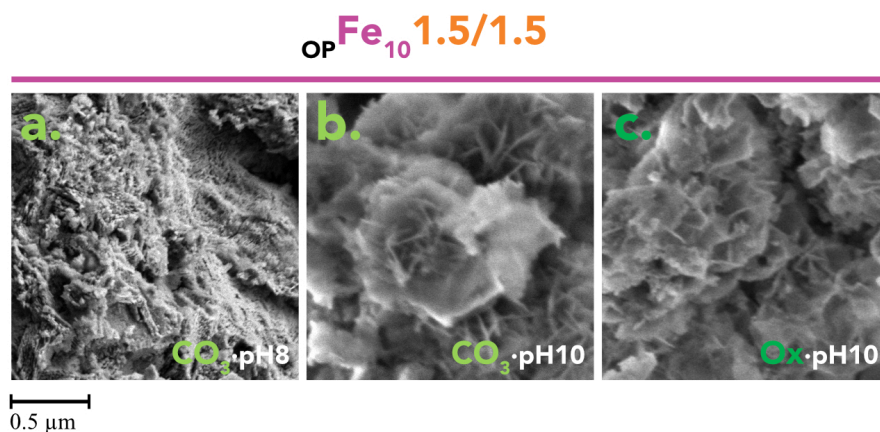
Figure 4.18: SEM pictures of OPFe_{10}1.5/1.5 catalysts calcined at 500^{\circ}C according to pH and anion.
