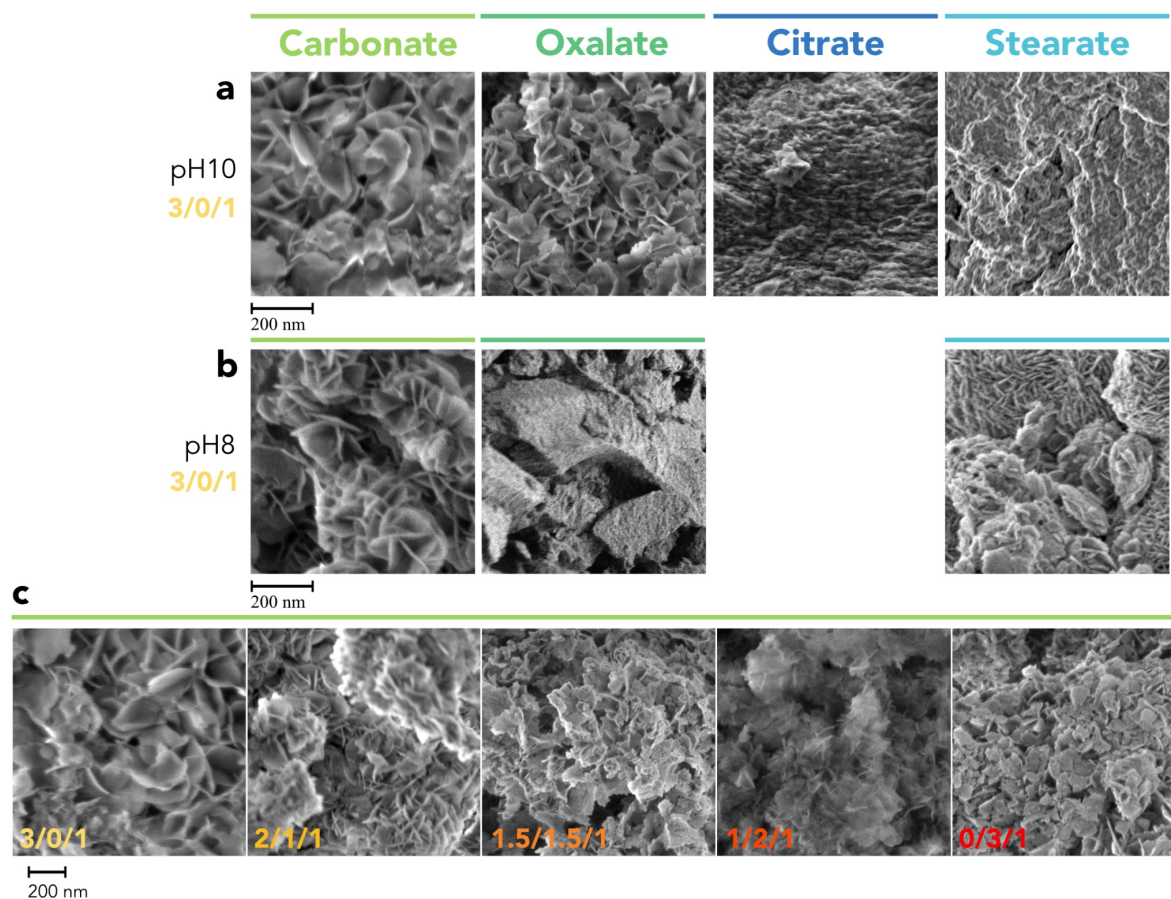
Figure 3.19: SEM pictures of a) Mg/Ca/Al pH10 samples versus interlayer anions, b) Mg/Ca/Al pH8 samples versus interlayer anions, and c) Mg/Ca/Al CO 3 -pH10 samples versus Mg/Ca ratio calcined at 500°C.
