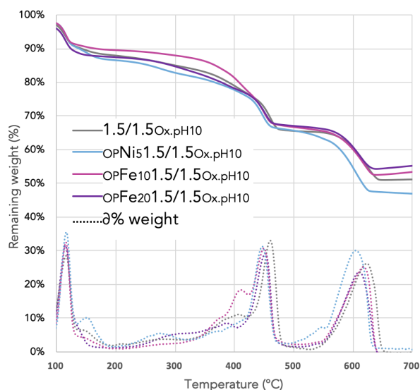
Figure 4.4: TGA oxidation of OP1.5/1.5_{\text{Ox-pH10}} catalysts compared to their corresponding sorbent.
