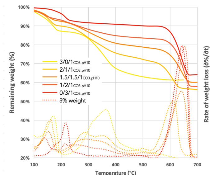
Figure 3.8: TGA oxidation of Mg/Ca/AlCO 3 -pH 10 samples with various Mg/Ca ratios.
