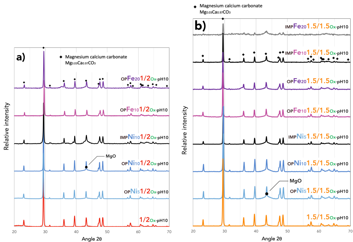
Figure 4.10: X-ray diffractograms of Ni and Fe catalysts prepared using Ox·pH10 according to Mg/Ca ratio (a) 1/2 and b) 1.5/1.5) and synthesis method compared to their corresponding sorbents.
