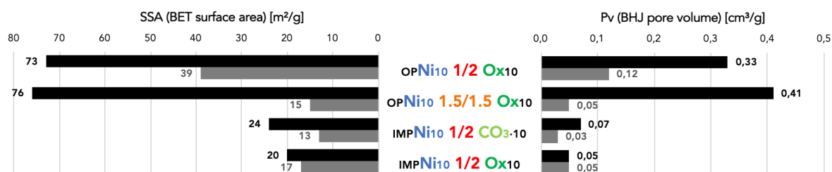
Figure 5.12: SSA and Pv for nickel catalysts pre- (in black) and post-SESR test (in grey).
