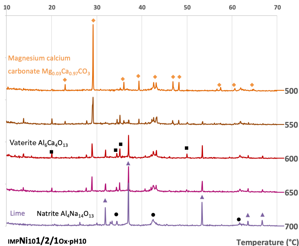
Figure 4.8: X-ray thermo-diffractograms of \text{IMPNi}_{10}1/2\text{Ox-pH}_{10} precursor according to temperature.
