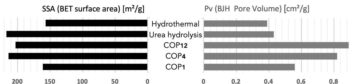
Figure 3.2: BET surface area (SSA) and BJH pore volume (Pv) for LDO samples calcined at 500°C according to synthesis method and sodium carbonate quantity.
