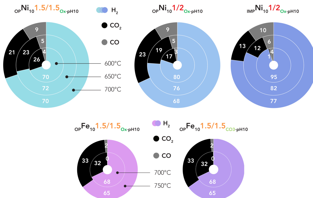
Figure 5.5: H 2 /CO 2 /CO ratio of outlet gas for nickel and iron catalysts according to temperature.
