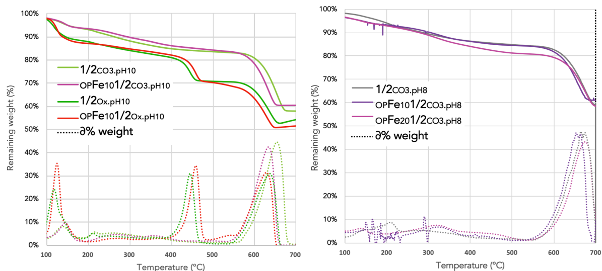
Figure 4.5: TGA oxidation of OPFe 10 1/2CO 3 .pH 10 , OPFe 10 1/2Ox.pH 10 catalysts (left) and OPFe 10&20 1/2CO 3 .pH 8 (right) compared to their corresponding sorbents.
