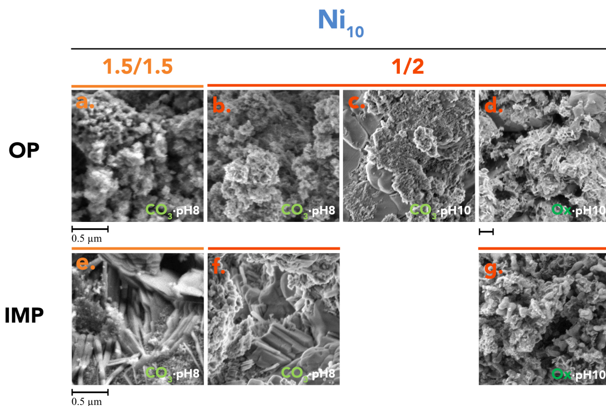
Figure 4.17: SEM pictures of Ni_{10} -LDO based catalysts calcined at 500^{\circ}C according to synthesis method, Mg/Ca ratio, pH, and anion.
