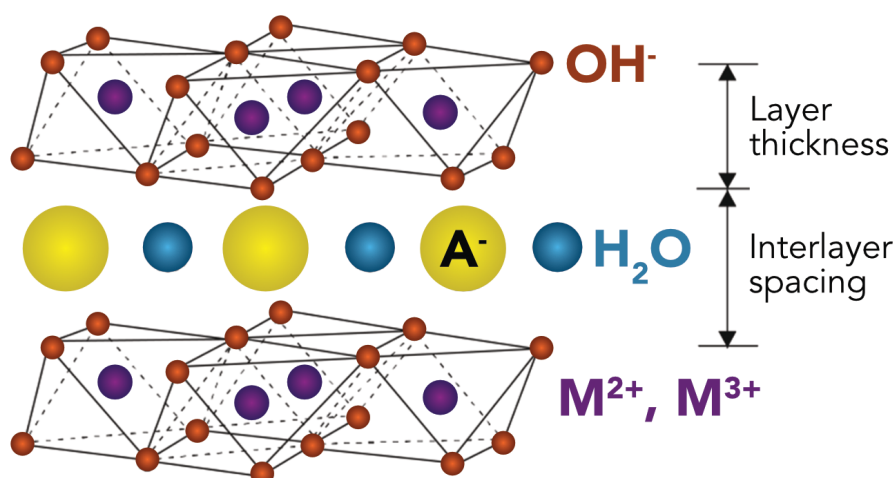
Figure 1.7: Illustration of LDH structure. The neutral charge is respected between hydroxide, interlayer anions and metal charges.
