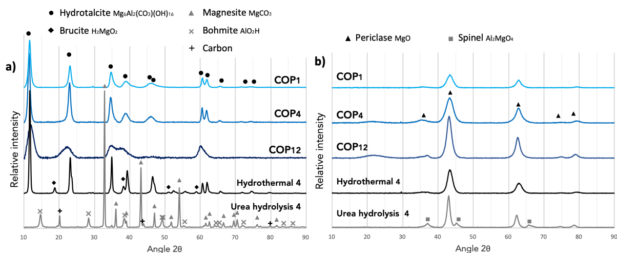
Figure 3.1: X-ray diffractograms of a) LDH prepared according to synthesis method and sodium carbonate quantity, b) corresponding LDO samples calcined at 500°C.
