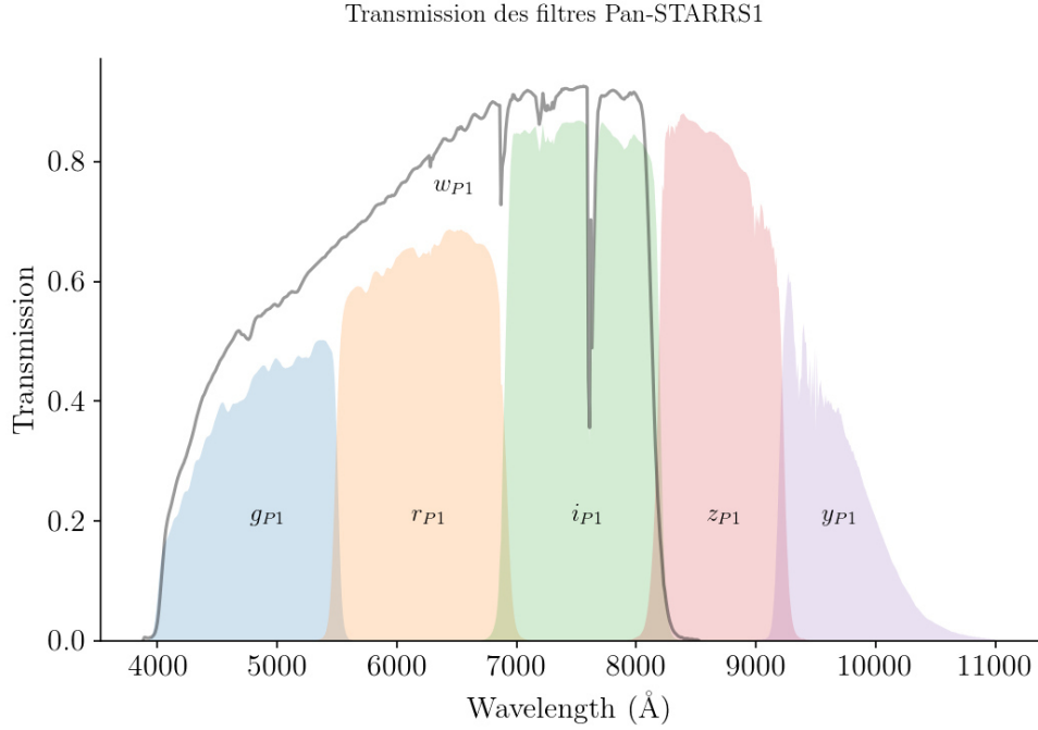
FIGURE 6.2 – Transmission des filtres grizy de Pan-STARRS1 (TONRY et al., 2012).
